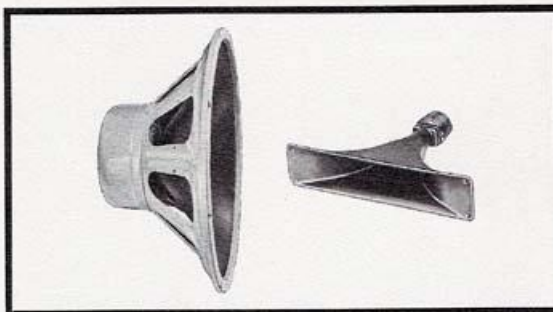
The Berkshire speaker system utilizes a super-power 15" bass speaker with 24-ounce magnet and a 1000-cycle exponential horn, ten times as efficient as the Concerto's speakers.
