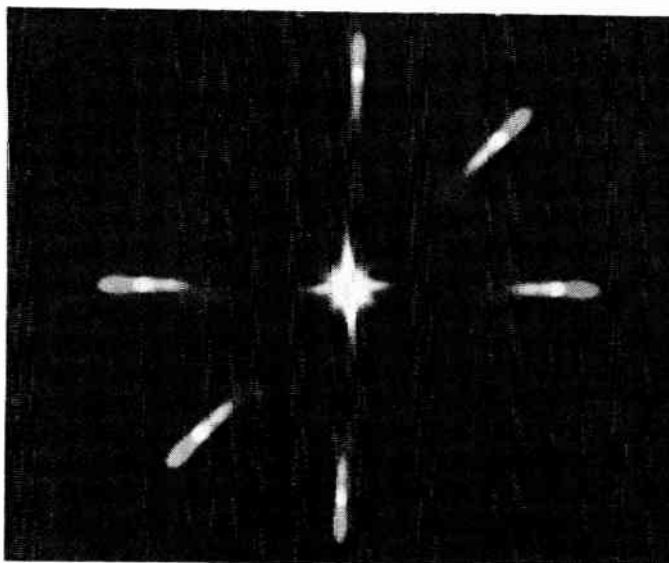
Fig. 4 Basic Fraunhofer Diffraction from ABTO film recording showing 3 images spatially separated.
