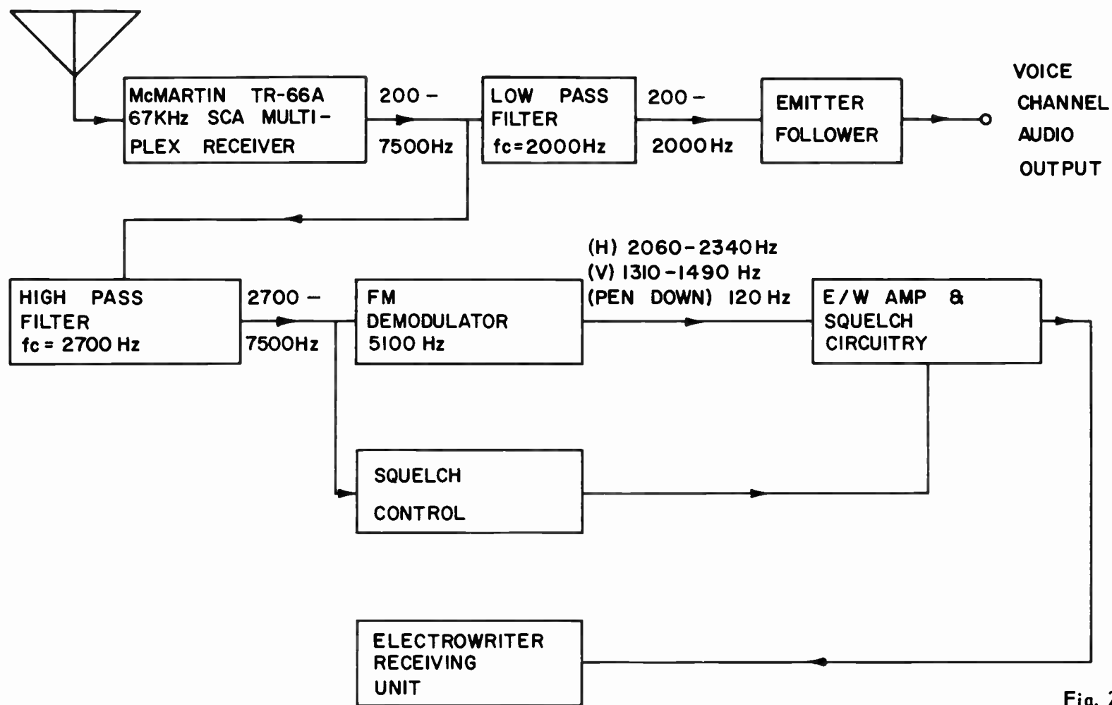
BLOCK DIAGRAM RECEIVING SYSTEM ELECTROWRITER / VOICE SIMULTANEOUS TRANSMISSION
