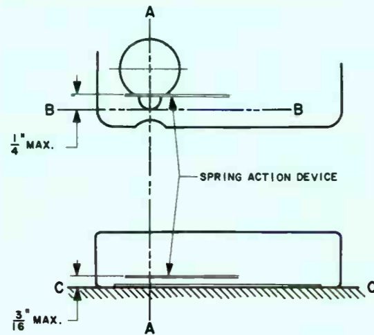
FIG. 1 REQUIRED SPRING ACTION DEVICE LIMITATIONS
