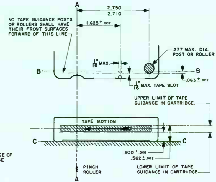
FIG. 4 TAPE GUIDANCE LIMITS
