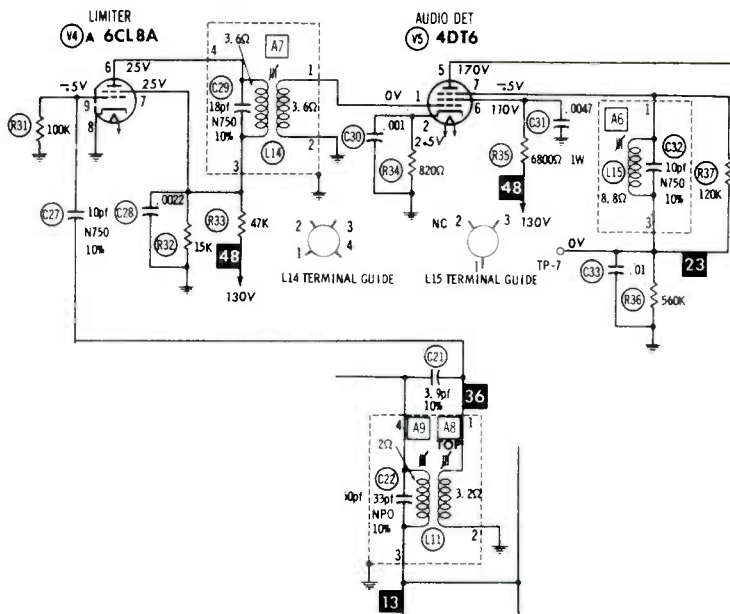
FIGURE 3. SOUND SYSTEM OF WESTINGHOUSE HP-3032.
