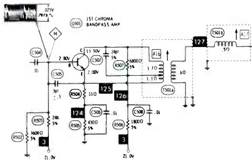
FIGURE 1. TOSHIBA BANDPASS AMPLIFIER.
