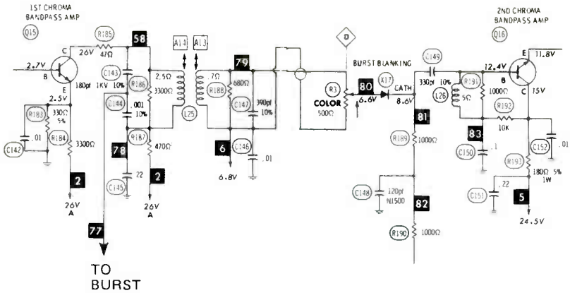
FIGURE 3. ADMIRAL CHASSIS K10-2A.
