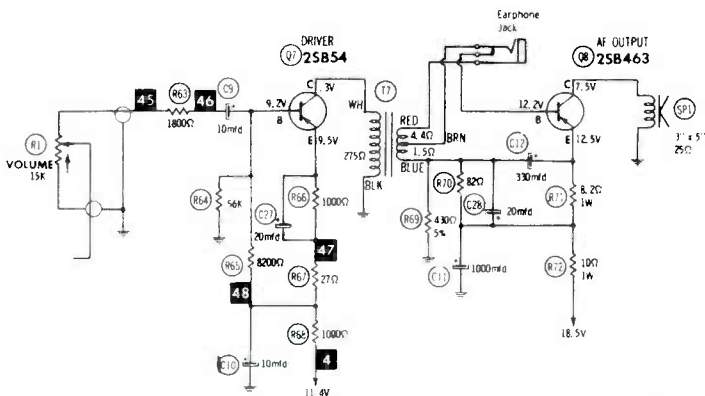
FIGURE 5. AUDIO SECTION OF SEARS MODEL 5024.
