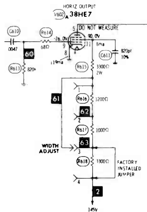
FIGURE 4. HORIZONTAL OUTPUT TUBE OF TRUETONE MODEL MIC 39128-17.
