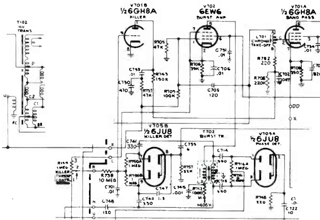
FIGURE 2. RCA VICTOR CHASSIS CTC15.
