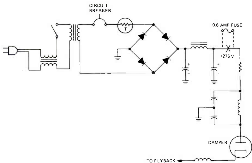
FIGURE 1. POWER SUPPLY AND DAMPER IN PHILCO 21ST90.
