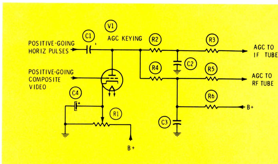
Fig. 1 Basic AGC keyer stage using a tube. Bias changes the plate resistance, and the plate resistance determines the amount of rectified negative voltage.
