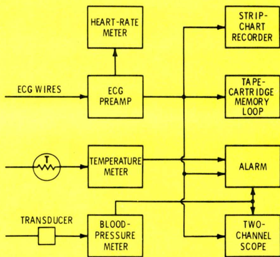
Fig. 12 Block diagram of a typical patient-monitor system.
