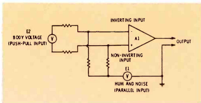
Fig. 4 Illustration of how hum and noise are cancelled in the differential amplifier of the IC, yet the wanted signal receives full amplification.
