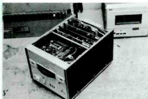
Fig. 8 Top view of the Model 7807C Hewlett-Packard heart-rate meter. The meter on front has a long, horizontal, analog scale. Complexity of the circuit is shown by the several plug-in circuit boards.
