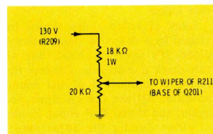
Fig. 5 Build this bias clamper to aid in testing the AGC action in RCA hybrid portable color receivers.
