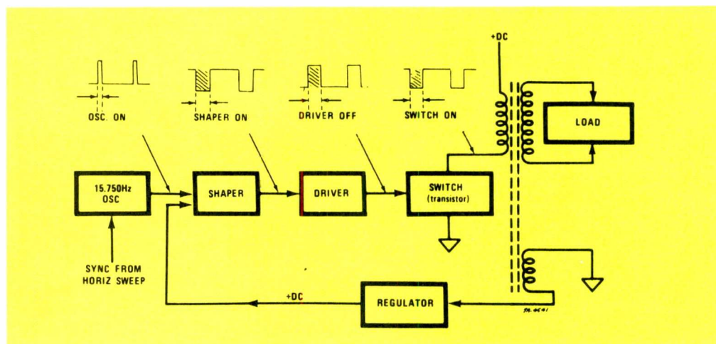
Fig. 6 Block diagram of the JA panel electronic regulation used in the TS931 and TS938 chassis. Synchronization from the horizontal oscillator in the sweep circuit is necessary to prevent the displaced scanning lines. (Courtesy of Motorola)
