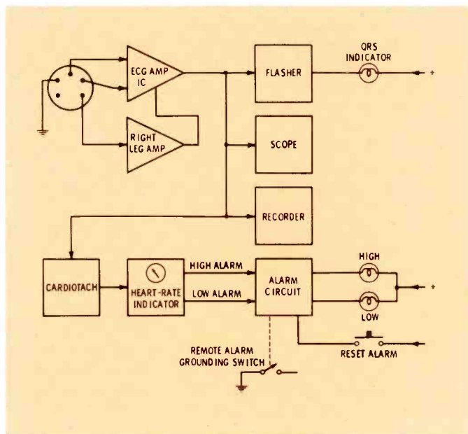
Fig. 7 Block diagram of a heart-rate meter, including an ECG pre-amplifier.
