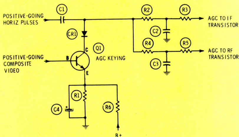
Fig. 2 When a transistor is substituted for a tube in the keyer circuit, a diode in series with the collector is necessary to prevent the negative rectified voltage from leaking away through the collector-to-base circuit.
