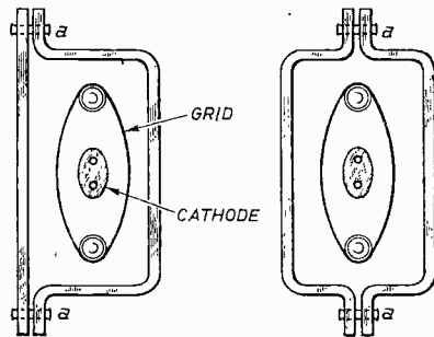
Fig. 2: Left - old style construction, vibration at anode fixing points a-a. Right - improved style, two halves lessen resonant peaks.
