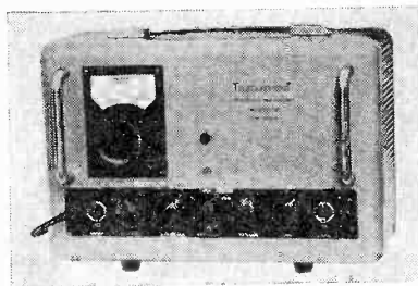
The Telequipment WG/44 provides a complete sound and vision signal with sync waveform.
