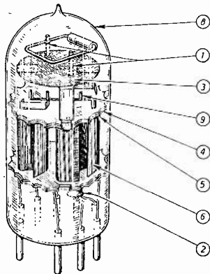
Fig. 1: Sketch of idealized modern valve showing some of the new design features described in the text.
