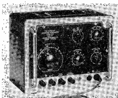
The Cossor 1324, a popular low-priced f.m. receiver alignment generator.
