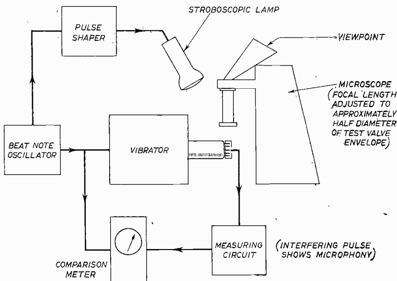
Fig. 3: Block diagram showing set-up for stroboscopic testing of microphonic sources.
