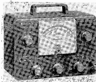
Appearance of the Beulah AG-9U-F (assembled) and the Heathkit AG-9U kit) sine wave a.f. generator covering from 20 c/s to 20 kc/s.
