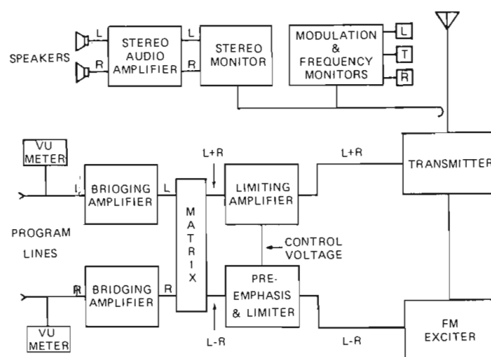
Belar compatible AM stereo transmitter system.
