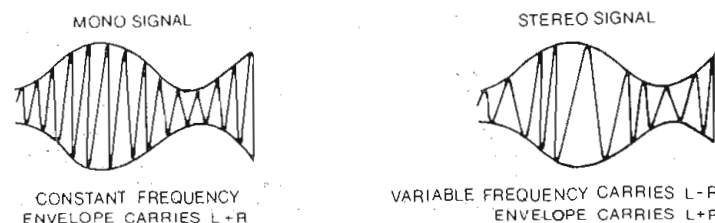
Monophonic and stereophonic modulation of a carrier.
