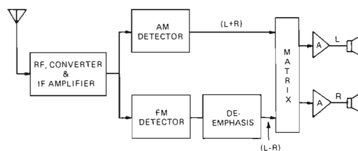
A compatible AM stereo receiver.
