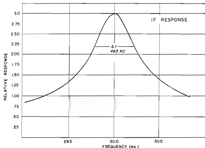
Fig. 5: (Left) Curve showing I-F response with constant input voltage. A scale convenient for measurement was used on the ordinate axis Fig. 6: (Right) Curve showing r-f response with constant input voltage. A scale convenient for measurement was used on ordinate axis
