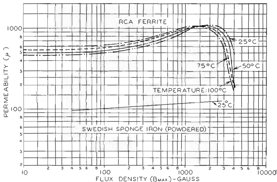
Fig. 4: Curves showing variation of permeability with flux density and temperature
