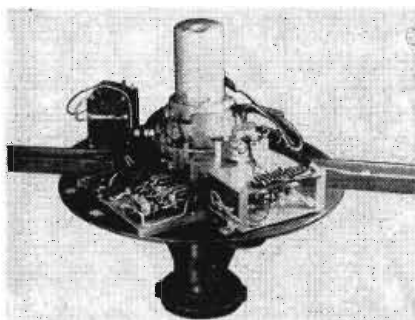
Fig. 1: Mechanical details of rotator base
