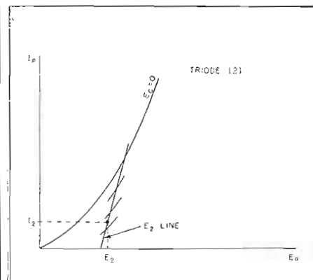
Fig. 2: Triode (2) plate curve construction
