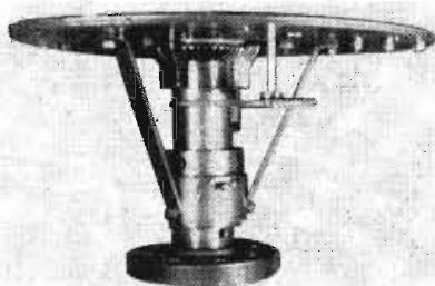
Fig. 2: Rotator and horizontal drive gear
