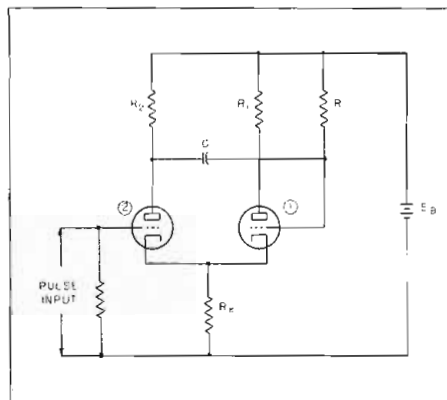
Fig. 1: Diagram of the multivibrator circuit
