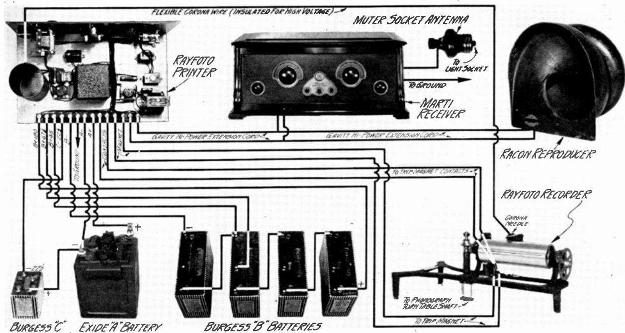
How the Cooley Rayfoto picture receiver is connected to an ordinary radio set for the reception of "still" pictures, either photographs or drawings.
