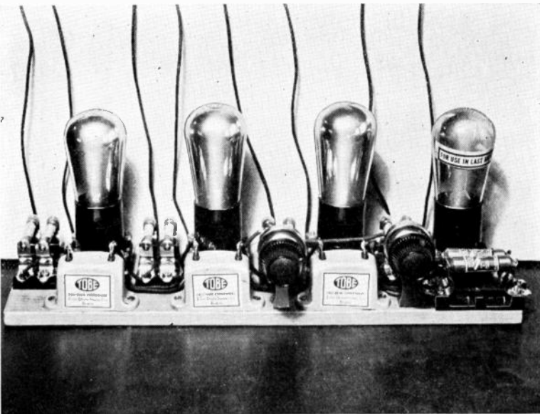
A photograph of a special resistance-coupled amplifier designed for the amplification of television signals.
