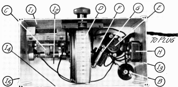
Showing the arrangement of the instruments within the short wave tuner. C is a short wave condenser, D a drum dial, G a grid leak, F a grid condenser, E a cushion socket, B a choke, and H a small variable condenser used to control the oscillations of the detector.
