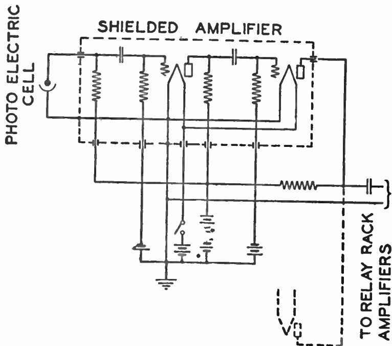
FIG. 35.—Ideal circuit of the resistance coupled type for amplification from a photoelectric cell. The dotted lines represent the copper shield about the amplifier. (Courtesy Bell Telephone Laboratories, Inc.)
