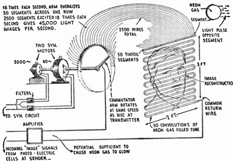
FIG. 2.—Showing the method used in impressing impulses upon a great neon tube provided with 2500 electrodes and a revolving contactor which properly distributes the light changes to the electrodes in such a way as to create the picture illusion. (Courtesy "Radio News.")
