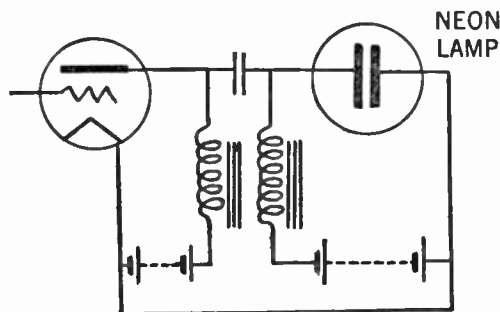
FIG. 44.—Neon lamp connected to the output circuit of vacuum tube amplifier using two impedances and two sets of B batteries.
