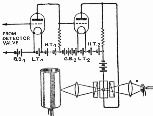
FIG. 7.—The essentials of the Karolus picture receiving system. The Kerr cell, which automatically regulates the intensity of the light beam to correspond with the fluctuations at the transmitter, is shown connected to the output of the vacuum tube amplifier. The cylinder carries the photo-sensitive paper upon which the picture is to be placed.
