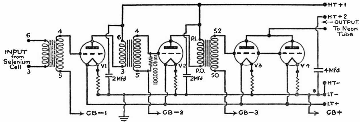
FIG. 26.—Circuit diagram of an audio-frequency amplifier suited to television experiments. The audio transformers used should be of an exceptionally good quality.
