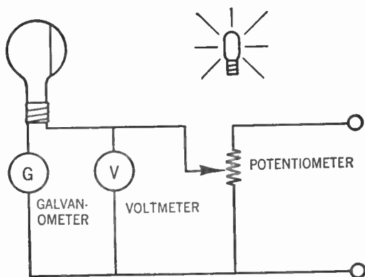
FIG. 21.—The simple circuit used to determine the volt-ampere characteristics of a cell. Such characteristics are plotted in the curves illustrated in Figs. 22 and 23. The potentiometer is naturally connected across a source of voltage, which as one of the curves shows, may go as high as 220.
