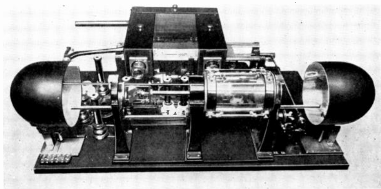
The transmitter of the Ranger system. As in all other photo-telegraphic systems, the picture is progressively explored with a fine pencil of light.
