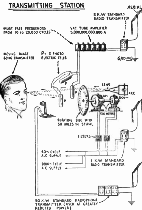
FIG. 1.—Simplified diagram of a complete television and telephonic broadcasting system. Three different wave-lengths are employed, one for the transmission of the picture of the living image, one for the voice or music, and one for the synchronism of the television scanning discs. (Courtesy Experimenter Publishing Company.)
