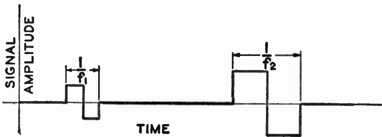
FIG. 34.—Signal detail of concentrated frequency spectrum for illustrating the effect of envelope delay. (Courtesy Bell Telephone Laboratories, Inc.)
