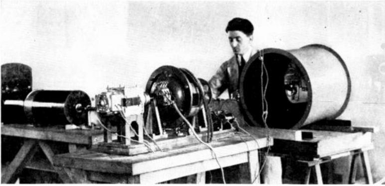
The electrical apparatus involved in the Belin-Holweck television transmitter. The photoelectric cell is mounted at the focal point of a large concave mirror which in turn is mounted at the end of the large cylinder shown. A cathode ray receiver is used in this system.
