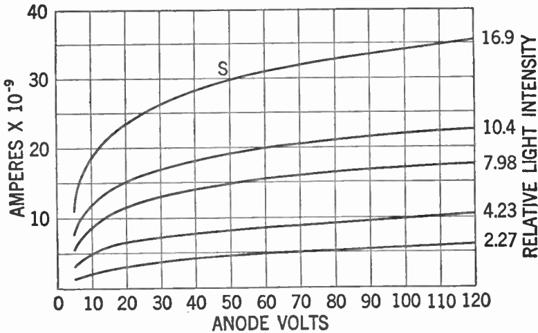
FIG. 22.—Here is a group of curves for a vacuum type photoelectric cell. This curve shows the output in current with different voltages and a uniform source of light. The anode voltage reached a maximum of 120.
