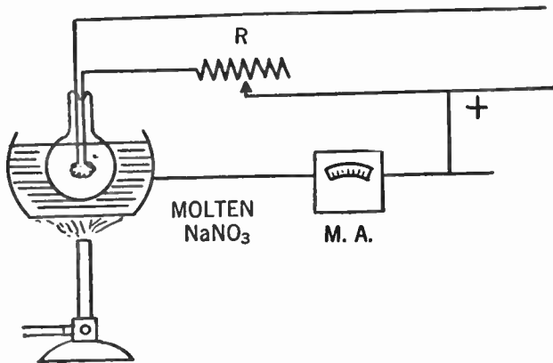
FIG. 24.—Electrolyzing sodium nitrate to deposit pure sodium upon the inside of a glass tube. It is this process that is employed in the manufacture of the Burt photoelectric cell. Such a process produces an extremely pure surface of the metal inside the cell. The milli-ammeter is included in the circuit to indicate the progress of the deposition.
