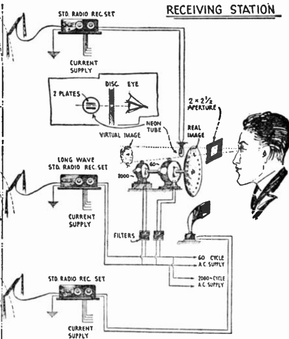
FIG. 1.—Simplified diagram of a complete television and telephonic broadcasting system. Three different wave-lengths are employed, one for the transmission of the picture of the living image, one for the voice or music, and one for the synchronism of the television scanning discs. (Courtesy Experimenter Publishing Company.)
