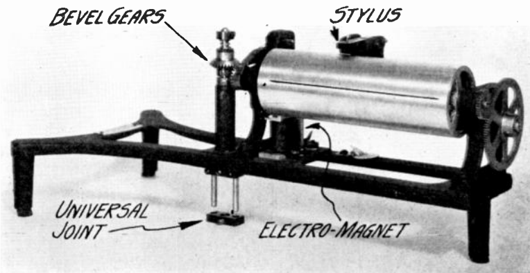
The printing drum of the Rayfoto picture receiver. The ends of the photo-sensitive paper used are pushed into the slot. The electro-magnet mounted beneath the drum is used to control the motion of the drum and to bring about synchronism between the transmitter and receiver. The high-voltage discharges take place at the point of the needle or stylus.
