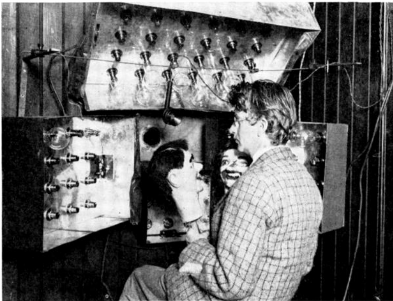
The Baird scanning mechanism. This system is similar to that illustrated in the diagram, Fig. 62. The disadvantage of this system lies in the fact that the subject has to remain exposed to a powerful source of illumination.
