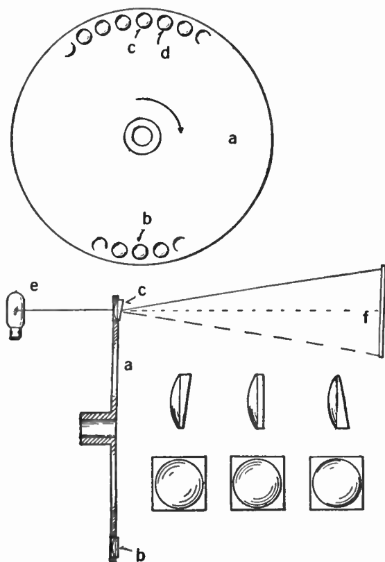
FIG. 60.—Jenkins' scanning discs using lenses ground in forms between the extremes shown in the lower right hand corner of the diagram.
