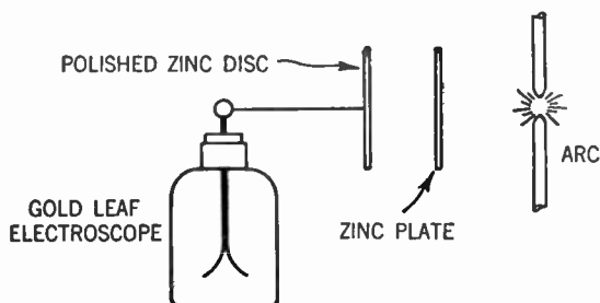
FIG. 19.—Hallwachs' first experiment. Light from an arc fell through a window in the zinc plate striking a second polished zinc plate connected to a charged electroscope. When the electroscope was positively charged, the light produced no effect. However, when the electroscope was negatively charged, the light caused the leaves in the electroscope to fall proving that the plate was losing its charge. It was these experiments that led up to the development of the photoelectric cell.
