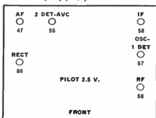
Models 551 (550), 561 (560) (1933)
