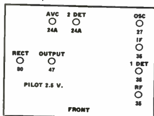
Model 05AA Series (1933)
