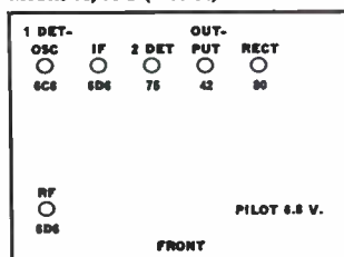
Model 58
