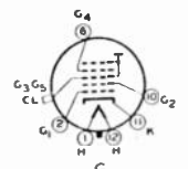
- G - ULTOR = G_2 + G_3 + CL FOCUSING ELECTRODE = G_4
