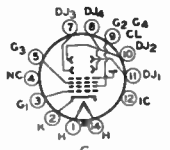
- C - ULTOR = G_2 + G_3 + CL FOCUSING ELECTRODE = G_3
