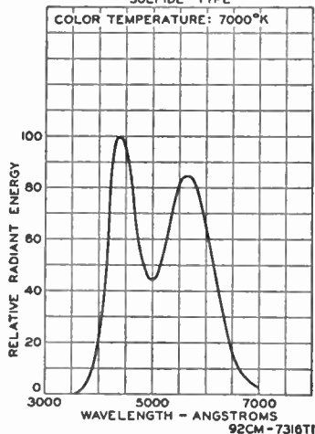
SPECTRAL-ENERGY EMISSION CHARACTERISTIC OF PHOSPHOR P4 SULFIDE TYPE
