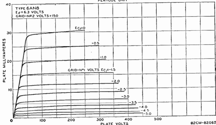
AVERAGE PLATE CHARACTERISTICS PENTODE UNIT
