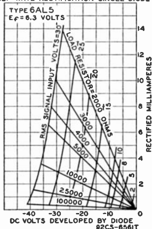
AVERAGE CHARACTERISTICS HALF-WAVE RECTIFICATION-SINGLE DIODE
