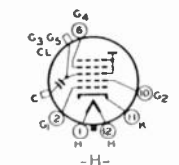
- H - ULTOR = G_3 + G_4 + CL FOCUSING ELECTRODE = G_4
