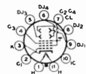
- A - ULTOR = G_2 + G_3 + CL FOCUSING ELECTRODE = G_3
