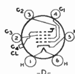
- D - ULTOR = G_4 + CL FOCUSING ELECTRODE = G_3
