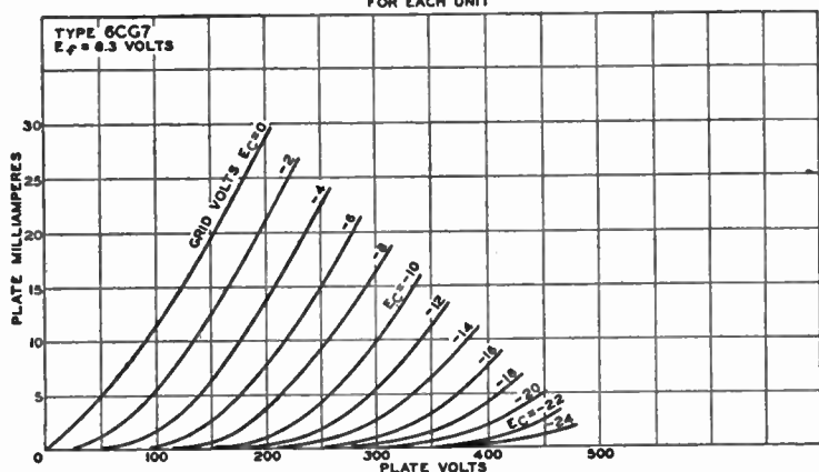
AVERAGE PLATE CHARACTERISTICS FOR EACH UNIT
