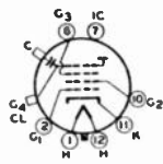
- B - ULTOR = G_4 + CL FOCUSING ELECTRODE = G_3
