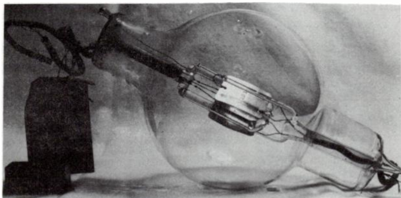
Fig. 7-9. A high-power Oscillon, vintage of 1915, 50 watts input.
