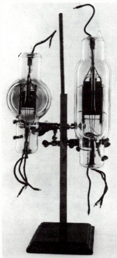
Fig. 7-25. Early 250-watt and 500-watt (input) Oscillions.
