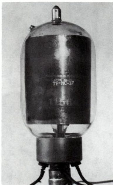
Fig. 11-14. Round Type TF-HC-3F valve without tubulation.
