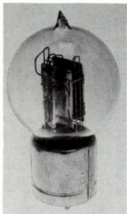
Fig. 6-17. A Type O or 104A repeater bulb; early construction, 1918.
