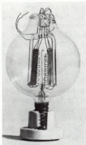
Fig. 6-3. The third improvement in the Audion: addition of second grid-plate assembly to increase the plate area.
