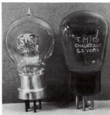
Fig. 19-2. SIF receiving tubes. Left: TM. Right: TM15.
