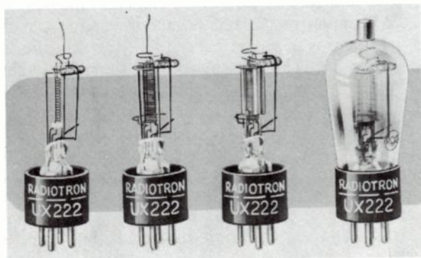
Fig. 16-10. Stages in the assembly of the Radiotron UX222.
