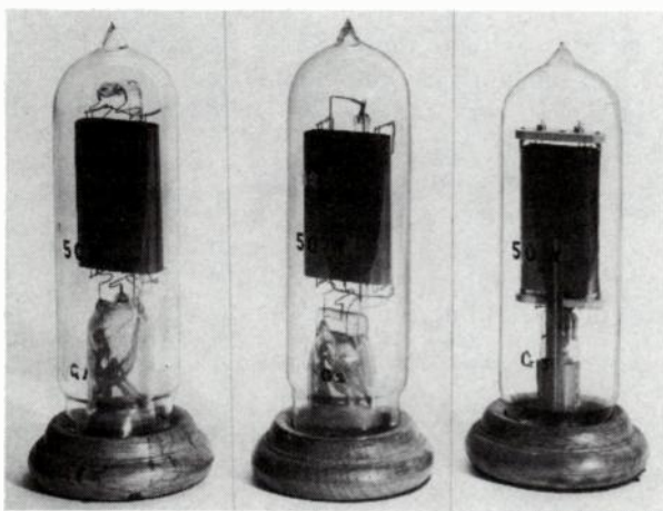
Fig. 14-11. Three experimental Type G tubes.
