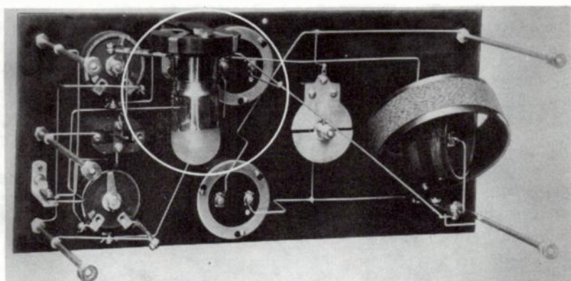
Fig. 17-12. Early Sodian tube mounted in a receiver.
