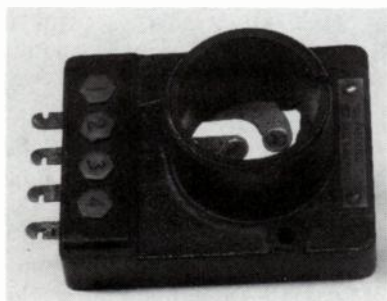
Fig. 6-9. Socket for the Type M telephone repeater element.
