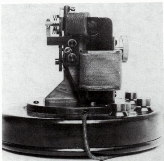
Fig. 11-1. Brown's Type G telephone relay.
