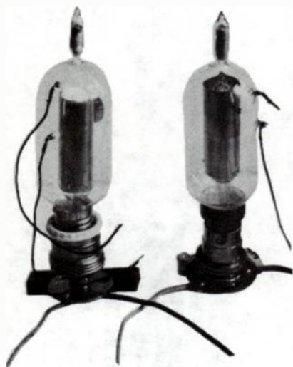
Fig. 11-8. Left: Round Type N with Edison medium screw base. Right: Round Type N with Edison bayonet base.
