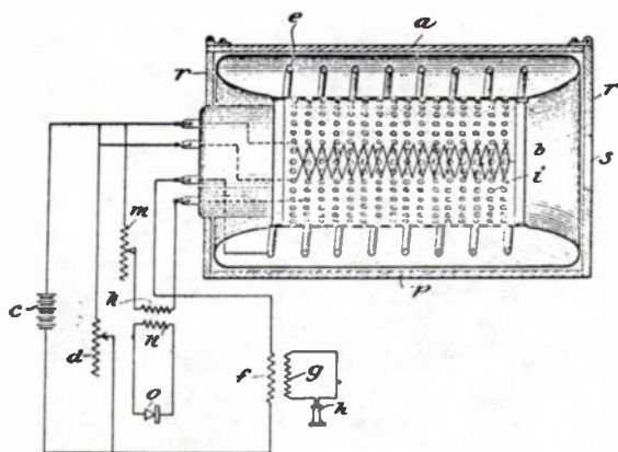
Fig. 13-8. The Tigerstedt telephone relay arrangement using magnetically and statically shielded concentric electrode assembly. (Reproduced from U.S. Patent No. 1,212,163.)
