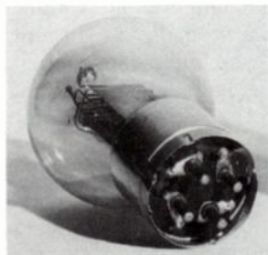
Fig. 6-12. An early type of fabricated sheet-metal base (before wax filling), showing the cruciform insert to hold contact pins.
