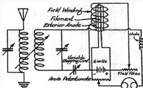
Fig. 17-8. Circuit in which the Connecticut J117 tube was used. (Reproduced from QST , Oct. 1921.)
