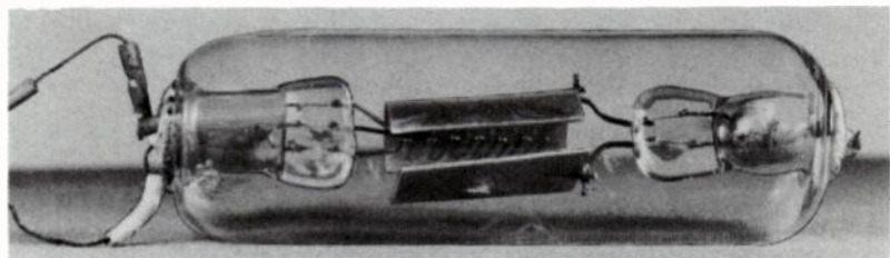
Fig. 22-17. Japanese TWW tube, showing electrode structure.
