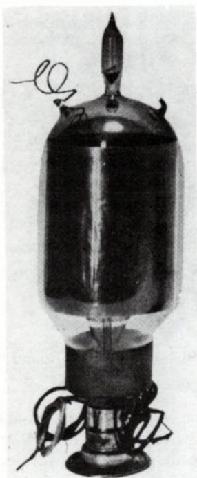
Fig. 11-10. Round Type T valve with multiple cathodes.
