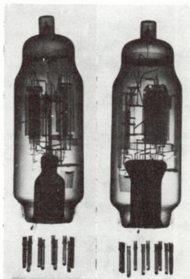
Fig. 21-33. X-ray photographs of Loewe WG36.
