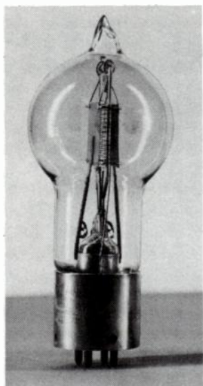
Fig. 9-17. The de Forest singer-type tube, 1920.
