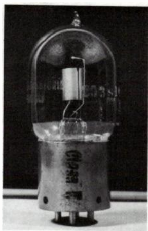
Fig. 9-12. Marconi VT with "Class II" rubber-stamped on base.
