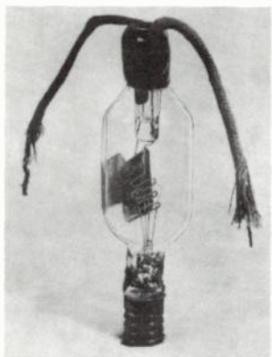
Fig. 4-14. Grid-type Audion used by the U.S. Navy in 1907-1908.
