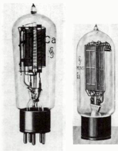
Fig. 21-14 (Left). Siemens & Halske Type Ca tube. (Reproduced from Veröff. NachrTech. , 1935, 5.)
