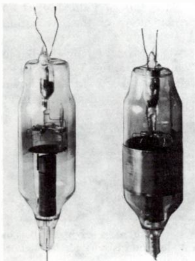
Fig. 9-26. Developmental Weagant transmitting valve. The view at the right has the external control electrode removed to show the internal construction of the valve.
