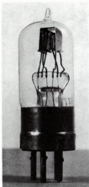
Fig. 18-32. Economic Electric Xtraudion.
