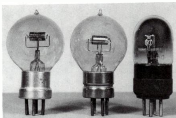
Fig. 19-3. La Radiotechnique tubes. Left to right: R3, R5, and Radio Ampli R5. The RT marking on the Radio Ampli R5 was adopted in 1923 with the change to a thoriated filament.
