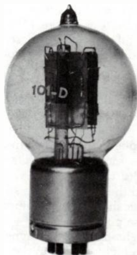
Fig. 14-1. The earliest type of 101D repeater bulb, 1921.
