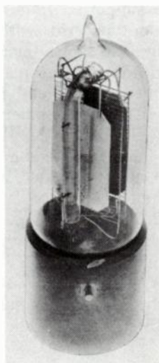
Fig. 6-18. The earliest version of the 203A vacuum tube (Type J). This tube has a machined brass base and glass arbor construction (1916).
