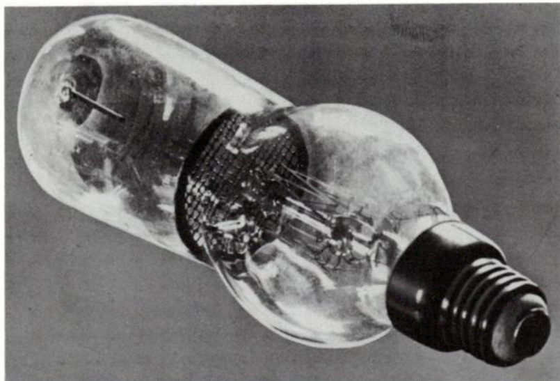
Fig. 5-7. Von Lieben electrostatically controlled cathode-ray relay of 1910.
