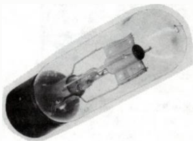
Fig. 8-23. Type U Pliotron (CG-1144, VT-18).
