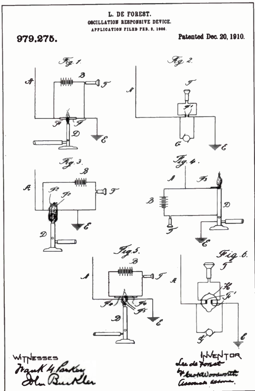
Fig. 4-2. Apparatus arrangement of de Forest's U.S. Patent No. 979,275.
