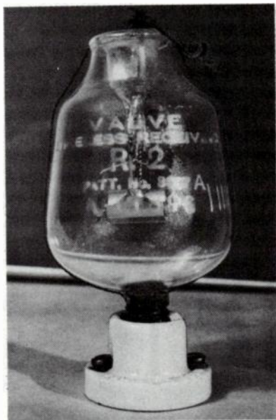
Fig. 11-19. Osram R2A valve fitted with a candelabra base for use in British naval apparatus designed to use the de Forest Audion. This valve was usually supplied unbased; the user applied whatever base he required.
