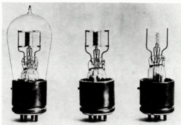
Fig. 8-22. Type T Pliotron (VT-14 or CG-1162). Left: complete tube. Center: with bulb removed. Right: with bulb and anode removed.
