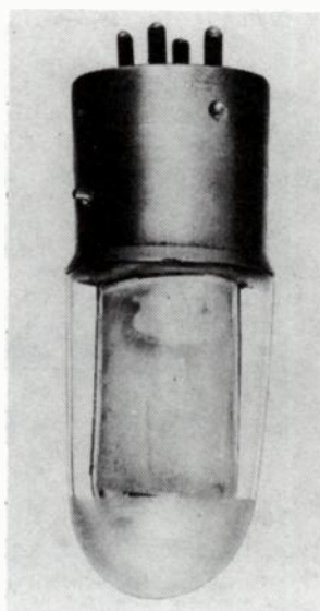
Fig. 17-10. Photograph of an early Sodian detector tube. (Reproduced from Proc. I.R.E. , Apr., 1923.)
