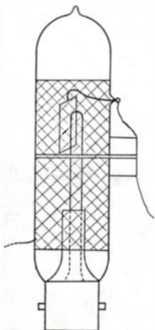
(A) Drawing. (Reproduced from Fleming's Thermionic Valve , London, 1919.)
