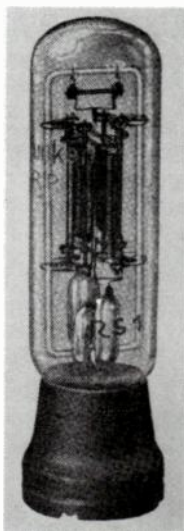
Fig. 12-34 (Left). Telefunken's first transmitting tube, the RS1. (Reproduced from Telefunken Fest. , 1928.)
