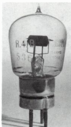
Fig. 11-23. The Os- ram R4B valve.
