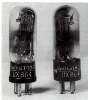
Fig. 16-27. Two versions of the Radiotron UX864: the one at the right has a low loss insulating compound in the base.
