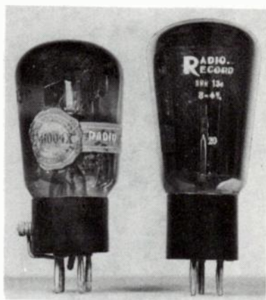
Fig. 20-18. Radio Record tubes. Left: M1004X. Right: RRR134.
