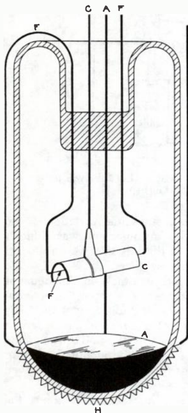
Fig. 17-9. Diagram of an early Sodian detector. (Reproduced from Proc. I.R.E. , Apr. 1923.)
