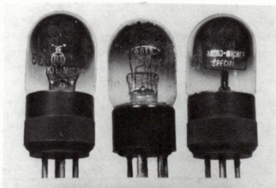
Fig. 19-5. La Radiotechnique tubes. Left to right: Radio Micro, Micro-Bigril, and Radio Micro Special.
