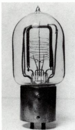
Fig. 8-8. Later sample of the Type CA Pliotron with cylindrical bulb and Shaw standard base. This tube has an improved electrode structure.
