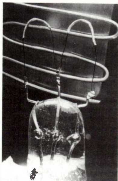
Fig. 7-2. Enlarged view of the Hudson filament as it was first made by McCandless.
