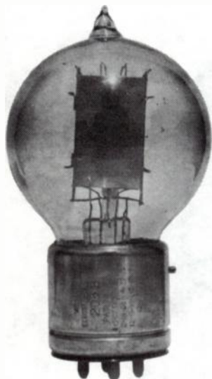
Fig. 14-10. The 205B vacuum tube. It is the same as the VT-2 except for the markings.
