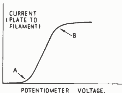
Fig. 11-32. Characteristic curve of the Fleming valve. (Reproduced from Bulletin L163 of Marconi's Wireless Telegraph Co. Ltd.)
