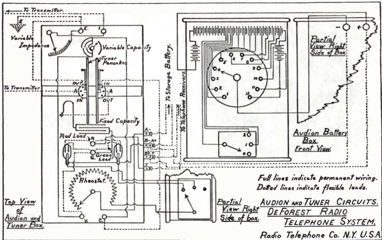
Fig. 4-17. Connections of Audion detector used on U.S. Navy ships in 1907-1908.
