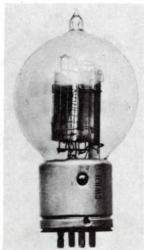
Fig. 6-22. The final form of the VT-2, Navy CW-931 vacuum tube. Note the phenolic insert in base.
