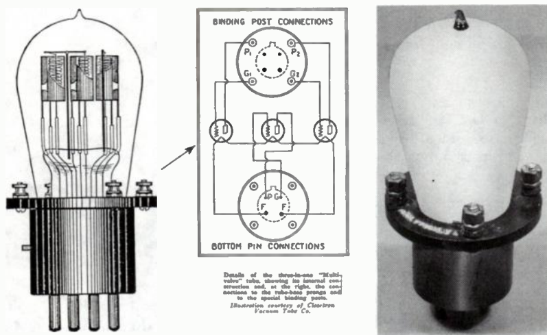
Fig. 17-20. The Emerson Multivalue. Note that the drawing was supplied by Cleartron Vacuum Tube Co.
