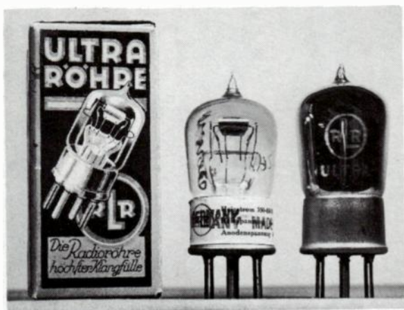
Fig. 21-42. Ultra UL550 (left) and U60 (right) tubes, with carton.
