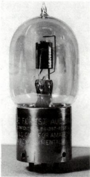
Fig. 7-22. Moorhead-Marconi-de Forest Electron Relay.
