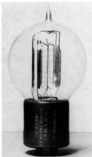
Fig. 6-8. Type M telephone repeater element, later coded the 101A repeater bulb.
