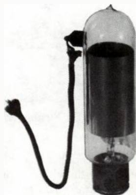
Fig. 3-10. Another commercial form of the Fleming valve.
