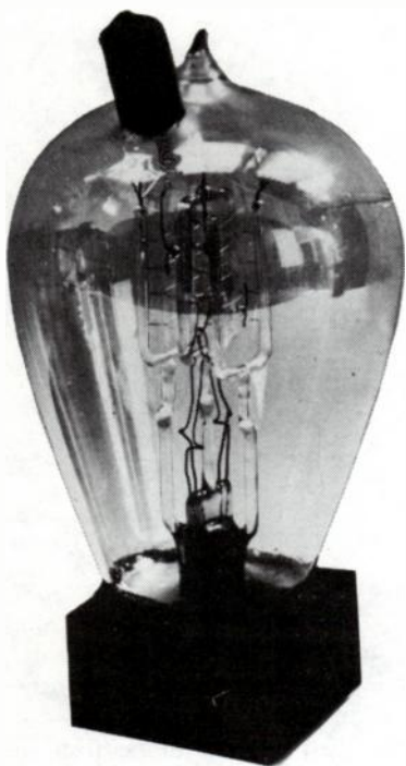
Fig. 8-4. An early type of wire-element Pliotron, now in the Science Museum, London.
