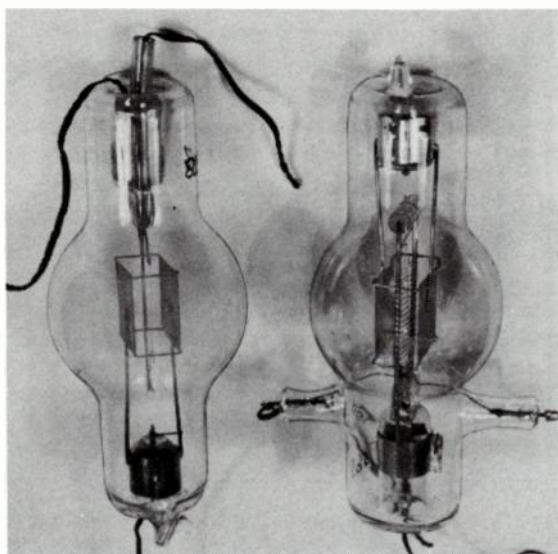
Fig. 15-2. The de Forest Types H and HR.
