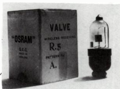
Fig. 11-24. The Osram R5 valve, with shipping carton.
