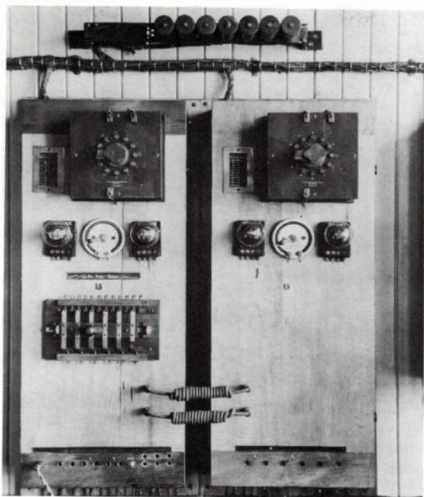
Fig. 6-10. The repeater at Brushton, Pennsylvania on the transcontinental line in 1915.
