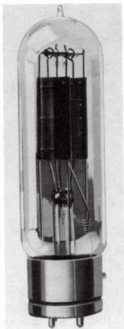
Fig. 16-23. Radiotron UV204 tube.
