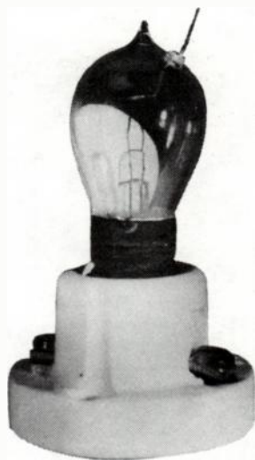
Fig. 4-3. Fleming valve made for C. D. Babcock by McCandless & Company in latter part of 1905.
