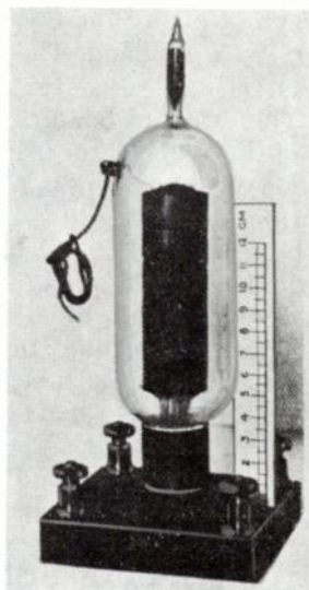
Fig. 11-2. The original British Post Office amplifying valve (Round type). Reproduced from P.O.E.E.J. , 1919.)
