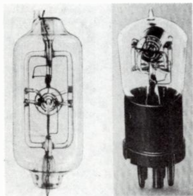
Fig. 12-32. Development of the Schottky triple-grid tube. Left: development model. Right: commercial tube. (Reproduced from Veröff. NachrTech. , 1935.)
