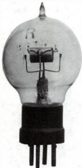
Fig. 11-20. Osram Type R valve.
