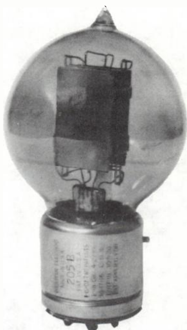
Fig. 6-23. The 205B vacuum tube. The same as the VT-2 except for markings.
