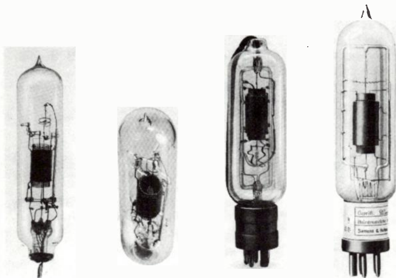
Fig. 21-4. Development series of the R tube. (Reproduced from Veröff. NachrTech. , 1935, 5.)
