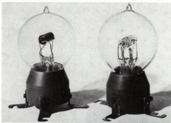
Fig. 11-5. Two forms of "Valve, Amplifying, No. 1" used by British Post Office as the first standard amplifying valve. The one at the right is the earlier construction.
