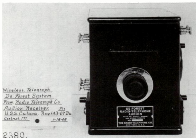
Fig. 4-18. Photograph of Audion detector in Fig. 4-17.
