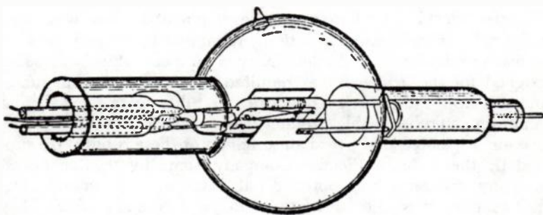
Fig. 8-13. Langmuir's drawing of large Pliotron. (Reproduced from Proc. I.R.E. , 1915, 3.)
