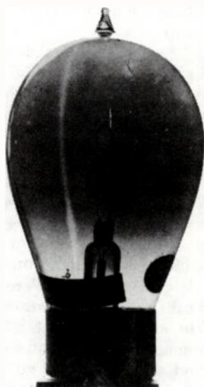
Fig. 2-2. Photograph of Edison lamp, discolored by use, but having a clear streak.
