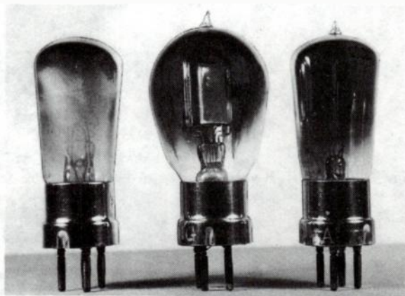
Fig. 18-35. B.T.H. B3, B4, and B5 valves (left to right).
