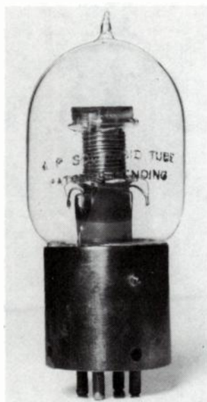
Fig. 9-20. Moorhead A-P solenoid tube.
