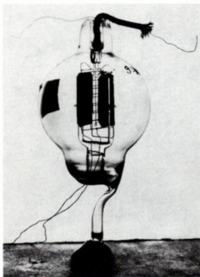
Fig. 6-7. Type B telephone repeater element.
