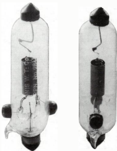
Fig. 11-27. Two views of the Marconi V24 valve.
