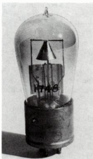
Fig. 8-27. Small receiving-type Plotron with helical grid and filament and conical anode. Made about 1919.
