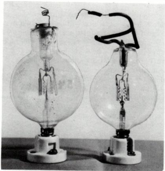
Fig. 7-19. American Marconi Type D valves.
