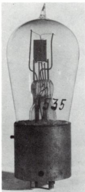
Fig. 8-20. The VT-13, or later Type CG-890 tube.
