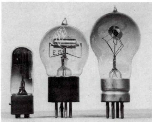
Fig. 19-16. SFR tubes. Left to right: R5, E52, E.
