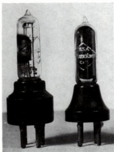
Fig. 18-5. S.T.&C. 4215A with adapter for use in British socket (left) and the 4215AB, with base to fit British socket.
