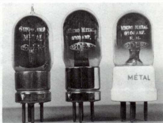
Fig. 19-4. Variants of 6/100 Micro-Métal. The tube at the extreme right, "MICRO-MÉTAL 6/100 AMP. R.M.," was intended for operation with ac on the filament. Note G·D·E·R· markings.
