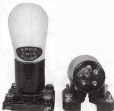
Fig. 17-19. The Apco Twin tube. The base with the switching mechanism is shown at the right.
