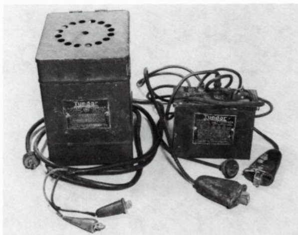
Fig. 8-30. Tungar rectifiers for home use. Left: for automobile batteries. Right: for radio A batteries.
