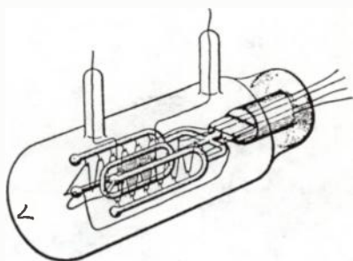
Fig. 8-12. Langmuir's drawing of small Pliotron. (Reproduced from Proc. I.R.E. , 1915, 3.)
