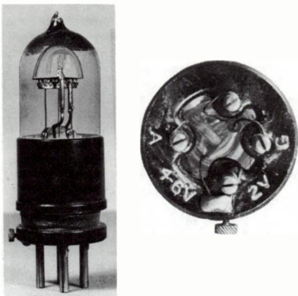
Fig. 18-13. Cossor WR2 valve with view of the base.
