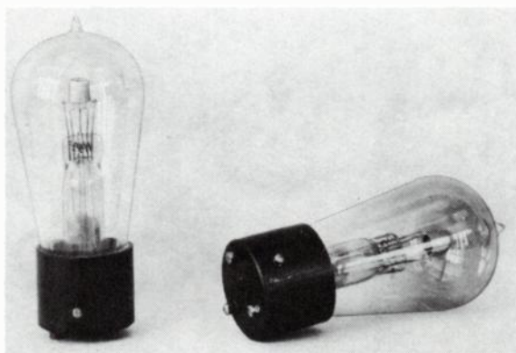
Fig. 8-18. Type G Plotron with three-point composition base, designated CG-886 by U.S. Navy.
