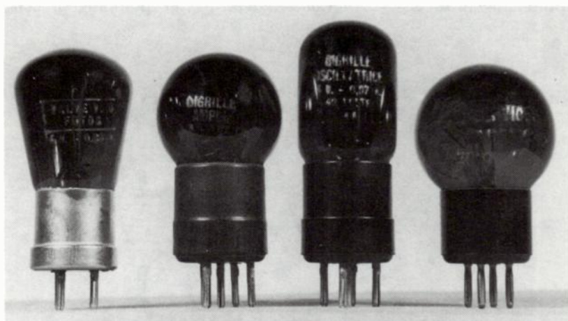
Fig. 19-6. Fotos (Grammont) tubes with blue glass envelopes. Left to right: V.O., Bigrille-Ampli, Bigrille-Oscillatrice, 209 Marine. Note difference in spelling as compared with La Radiotechnique tubes shown in Fig. 19-5.
