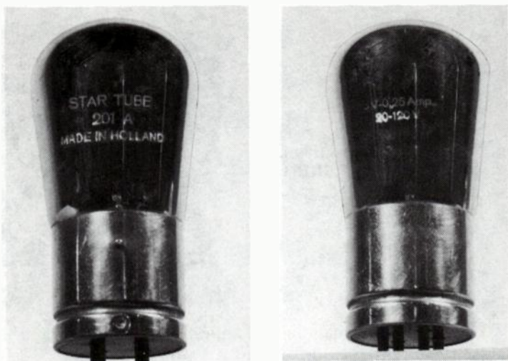
Fig. 20-20. "Star Tube 201A Made in Holland." Left: front view. Right: back view.
