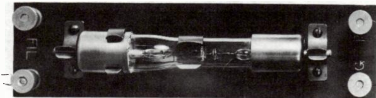
Fig. 9-24. Proposed commercial form of Weagant receiving valve in mounting. Note that the external control electrode is part of the mounting, not of the tube.
