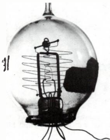
Fig. 8-5. An early Pliotron before exhaust (Pliotron 225). The exact date is unknown, but probably late 1915. The grid is tungsten wire 0.4 mil in diameter, wound on a metal frame with pitch of 120 turns per inch. The anode is 7-mil tungsten wire. Note the five leads: two filament, one grid, and both ends of the anode.
