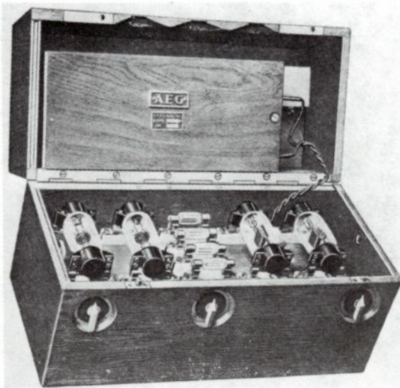
Fig. 12-16. The AEG K4 amplifier using K6 tubes in the output stage. (Reproduced from J. Zenneck and H. Rukop, Lehrbuch der drahtlose Telegraphie , 5th ed., Stuttgart, 1925.)
