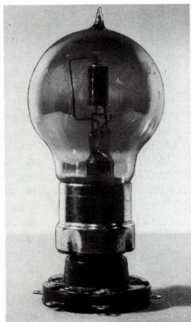
Fig. 18-40. Radion Type A valve.
