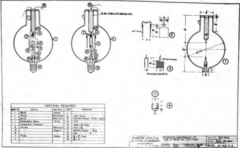
Fig. 7-20. American Marconi manufacturing drawing for Type D valve.
