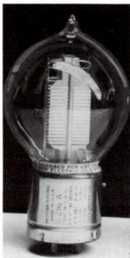
Fig. 14-19. An early 216A vacuum tube.
