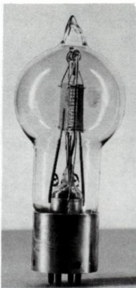
Fig. 7-5. Final construction of the singer-type Audion.
