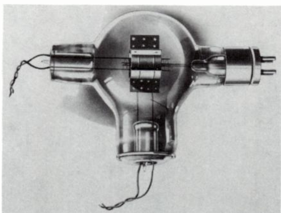
Fig. 16-26. Radiotron UX852 tube.
