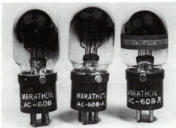
Fig. 17-17. Marathon ac tubes.
