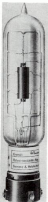
Fig. 21-7. Siemens & Halske BE tube. (Reproduced from Siemens-Z. , 1922.)
