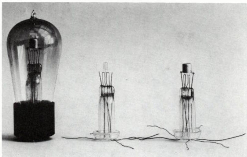
Fig. 8-19. Type G Pliotron (VT-11, early CG-890). Left: completed tube. Center: with bulb removed. Right: with bulb and anode removed.
