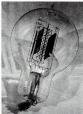
Fig. 14-32. Nicolson's "Experimental Audion No. 1000" with indirectly heated cathode.
