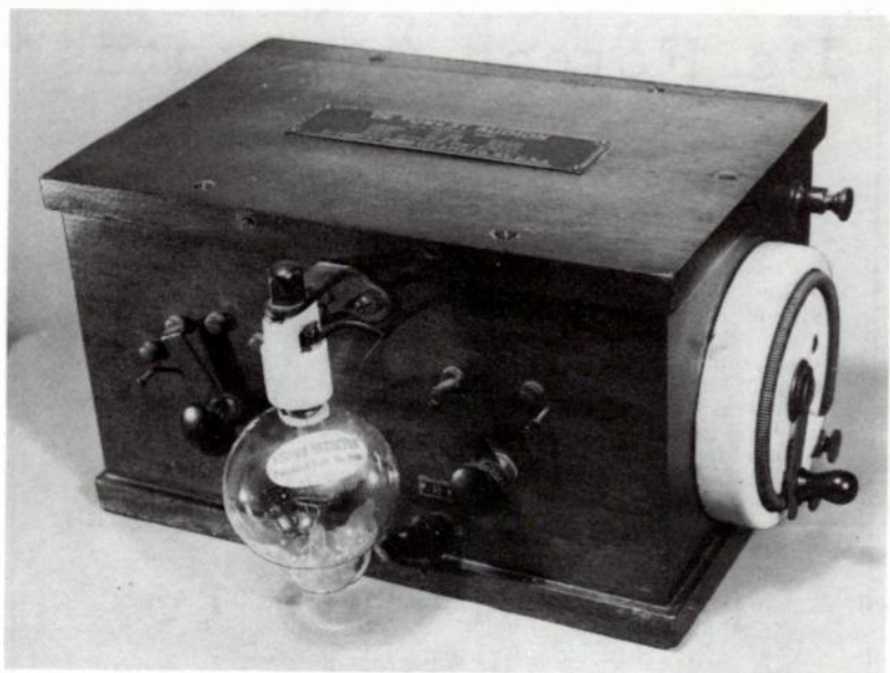
Fig. 4-23. The RJ4 detector. The tap switch at the left controls the plate voltage, that at the right is the off-on switch for the filament. The filament rheostat is mounted on the right-hand end of the box.
