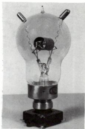
Fig. 19-1. SIF low-power transmitting tube for high-frequency use.
