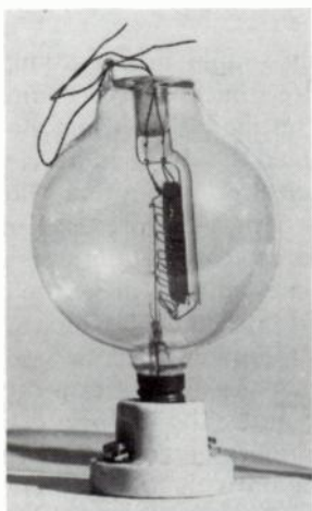
Fig. 6-2. The second improvement in the Audion: addition of glass arbor to promote rigidity.
