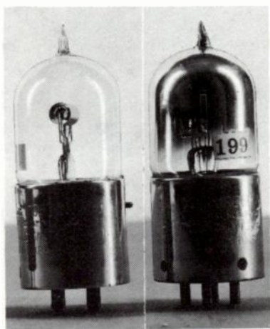
Fig. 7-24. The de Forest Type 20 detector. Left: early type of soft tube. Right: later type with getter.
