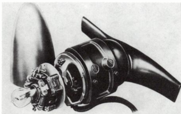
Fig. 8-17. Wind-driven generator, showing the TB1 regulator tube in mounting.
