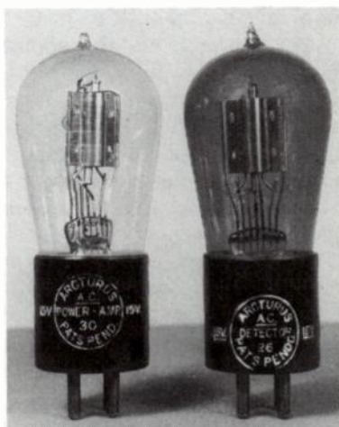
Fig. 17-15. Arcturus AC-30 and AC-26 tubes.
