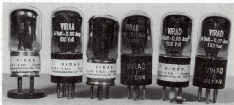
Fig. 20-19. VIR tubes. Two samples each of VIRAA, VIRAC, and VIRAD, showing variations in markings.
