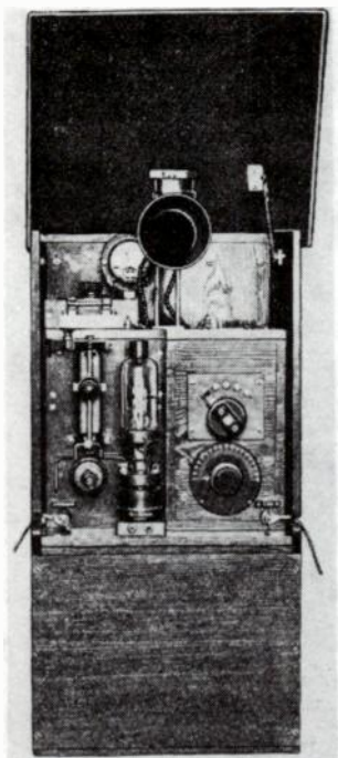
Fig. 12-26. Telefunken transmitter, made in 1915, using EVN129 tube. (Reproduced from Zenneck and Rukop, Lehrbuch der drahtlose Telegraphie .)
