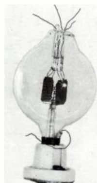
Fig. 4-21. A double Audion with separate leads from each grid and plate.
