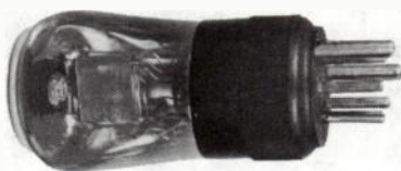
Fig. 19-9. Visseaux RO4215. Note difference in length of base pins.
