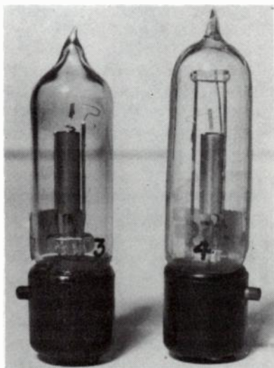
Fig. 14-25. Left: model of 215A vacuum tube with redesigned filament tension spring. Right: later model with small-diameter glass bead added for stiffening the element assembly.
