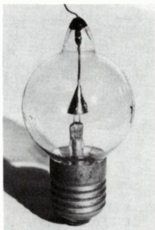
Fig. 8-26. Small Kenotron with medium screw base and conical anode. Used about 1919.
