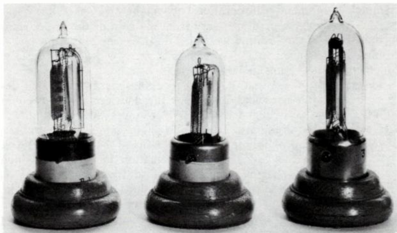
Fig. 6-19. Successive steps in the transformation of the early Type J tube into a rugged unit, suitable for military applications.
