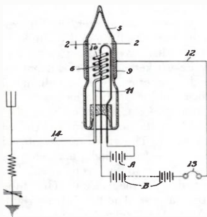
Fig. 17-3. Drawing of the Donle electron valve. (Reproduced from U.S. Patent No. 1,291,441.)
