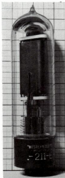
Fig. 14-14. The 211E vacuum tube with molded base.
