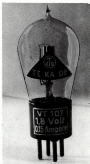
Fig. 21-43. Te-Ka-De VT107 tube.
