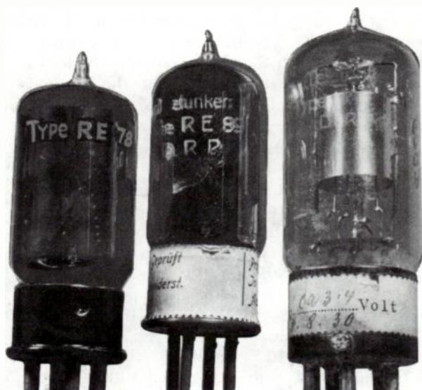
Fig. 21-17. Left to right: Telefunken RE78, RE89, RE201 tubes.
