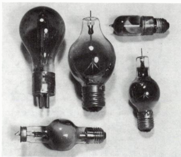
Fig. 8-29. Group of Tungar bulbs.
