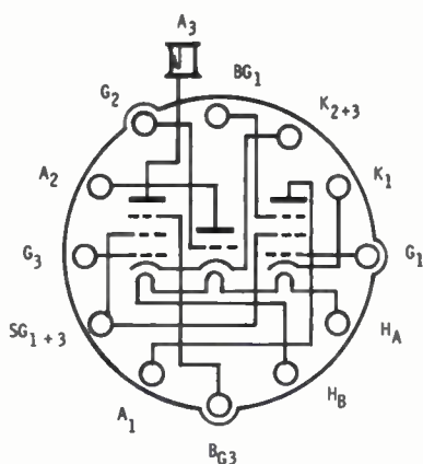
Fig. 21-34. Base connections of Loewe WC36.
