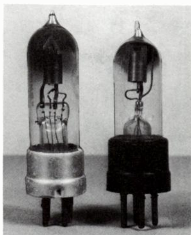
Fig. 18-30. Electron Company Amrex valves.
