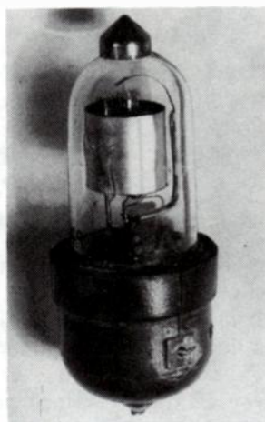
Fig. 11-26. Air Force D valve, made by Osram.
