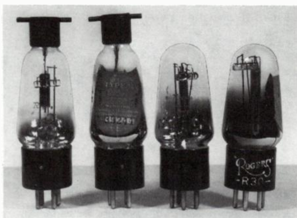
Fig. 17-21. Rogers Types 30 and 32 tubes. Left to right: Type 32 with markings etched on bulb, Type 32 with paper label, Type 30 with markings etched on bulb, and Type 30 with markings stamped on base.
