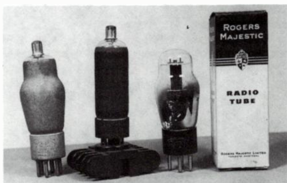
Fig. 17-23. Rogers Types 88S, 88M, and Rogers-Majestic Type 27 with carton. Left to right: 88S with spray shield, 88M with black "metallized" coating, and Rogers Majestic Type 27 with carton.
