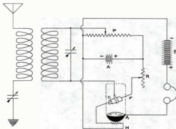
Fig. 17-11. Circuit in which early Sodian tube was used as a detector. (Reproduced from Proc. I.R.E. , Apr., 1923.)
