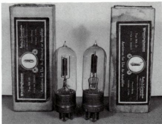
Fig. 16-4. Westinghouse E. & M. Co.'s Aeriotrons WR21D and WR21A, with packing cartons. The 21D, with lacquered tip, is at the left.
