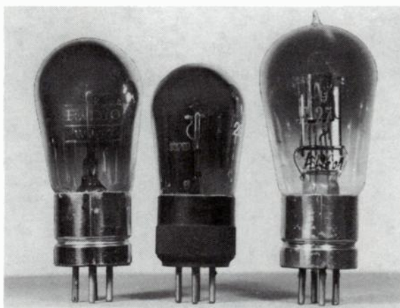
Fig. 19-7. La Radiotechnique tubes. Left to right: Radio Watt R31 (radio output tube), Super Ampli, E27 (output tube).
