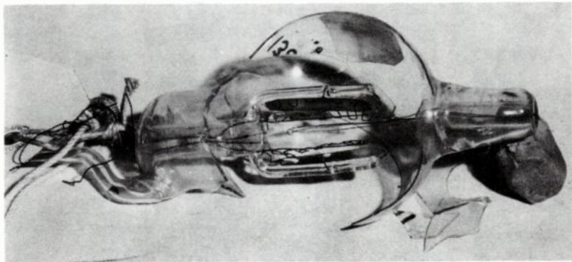
Fig. 6-5. The remains of Audion 6.11, used by Kendall at Philadelphia.
