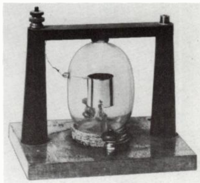
Fig. 3-6. Early type of Fleming valve using cylindrical plate.
