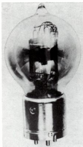
Fig. 6-21. An early form of the Type E, 205A, or VT-2 vacuum tube. This tube has a sheet-metal, wax-filled base.
