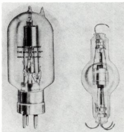
Fig. 18-19. Marconi-Osram T30 and T250 valves.
