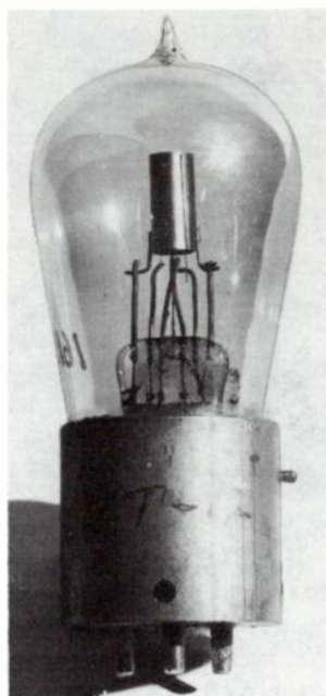
Fig. 8-21. Type T Pliotron; Signal Corps VT-12.
