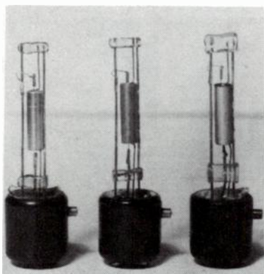
Fig. 14-26. The 215A vacuum tube with glass envelope removed. This illustration shows the increased size of the stiffening glass bead and the molded bayonet pin.
