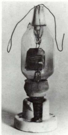
Fig. 4-15. Grid-type Audion once owned by Dr. J. A. Fleming, now in the Science Museum, London.
