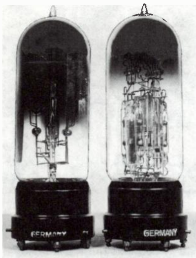
Fig. 21-26. Loewe 2HF (left) and 3NF (right) tubes.
