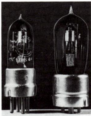
Fig. 18-14. Mullard ORA valves. Left: with British base. Right: with American UV base.
