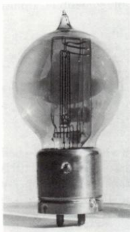
Fig. 6-15. An early 101B repeater bulb with the arbor welded to the edge of the press.
