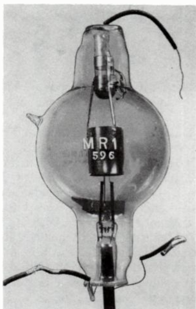
Fig. 18-22. Marconi-Osram MR1 transmitting valve.
