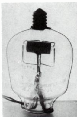
Fig. 11-22. The R4A valve.
