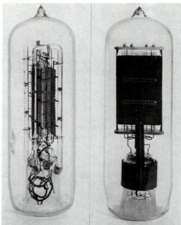
Fig. 14-15. Experimental I tubes.
