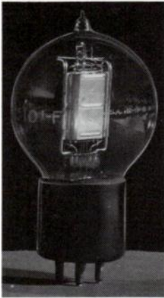
Fig. 14-5. The earliest form of the 101F vacuum tube.
