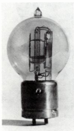
Fig. 6-16. A 101B repeater bulb with the arbor welded to the stem below the press.
