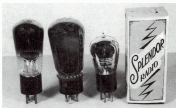
Fig. 20-17. Splendor tubes. Left to right: V1508, G450, and HF.
