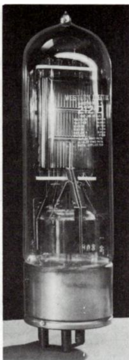
Fig. 14-17. The 212D vacuum tube.
