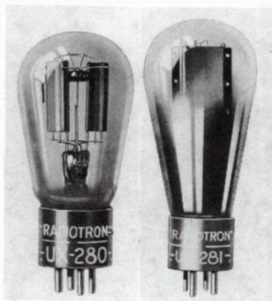
Fig. 16-19. Radiotrons UX280 and UX281.
