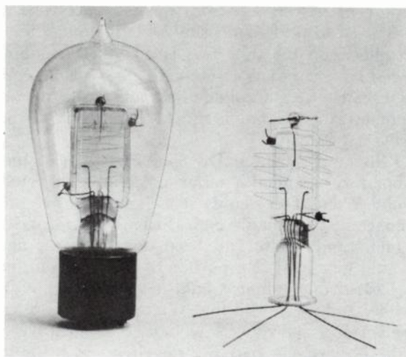
Fig. 8-7. Type CA Plotron, vintage 1918. Left: completed tube. Right: element assembly on stem.
