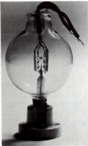
Fig. 7-1. Spherical Audion with the Hudson filament.
