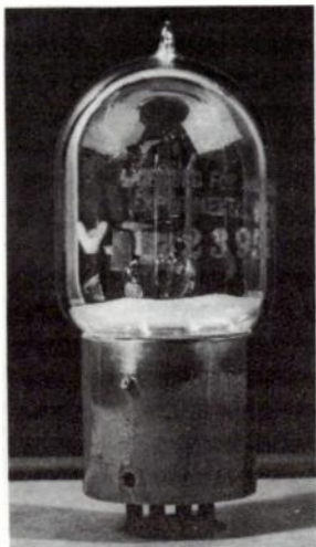
Fig. 9-14. The Marconi VT with steel-stamped base markings.
