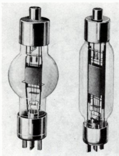
Fig. 7-27. The 250-watt-input Type 1D and 500-watt-input Type 1G Oscillions, vintage 1920, equipped with end fittings.
