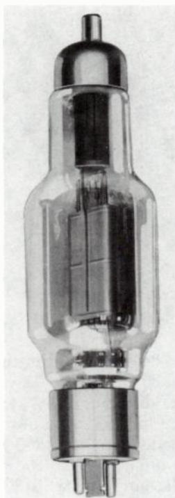
Fig. 16-24. Radiotron UV204A tube.
