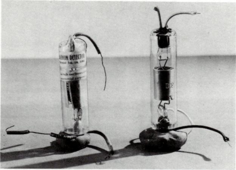
Fig. 7-12. Type T Audions. The one at the left shows the DF stamping on the plate.
