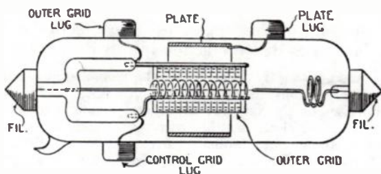
Fig. 11-29. Drawing of the F.E.1. valve. (Reproduced from H. J. Round, The Shielded Four-Electrode Valve , London, 1927.)
