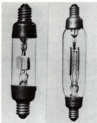
Fig. 13-3. N.V. Bal detector tubes, 1918. The one at the left is the earlier construction.
