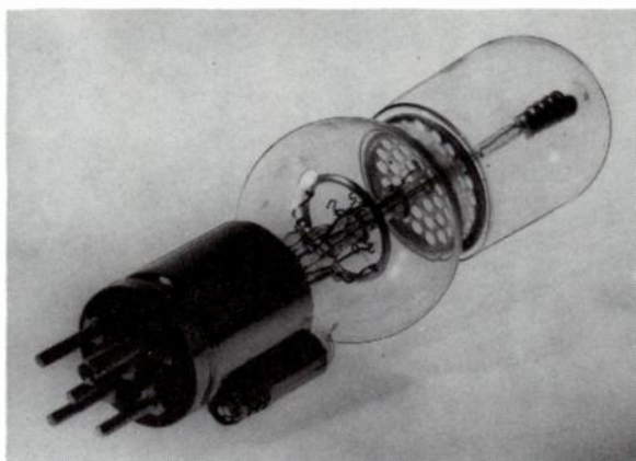
Fig. 12-6. Small LRS relay with perforated aluminum grid.
