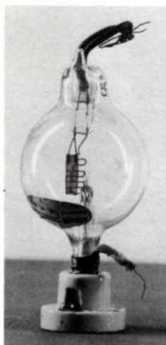
Fig. 4-19. A 1908 double-filament Audion.
