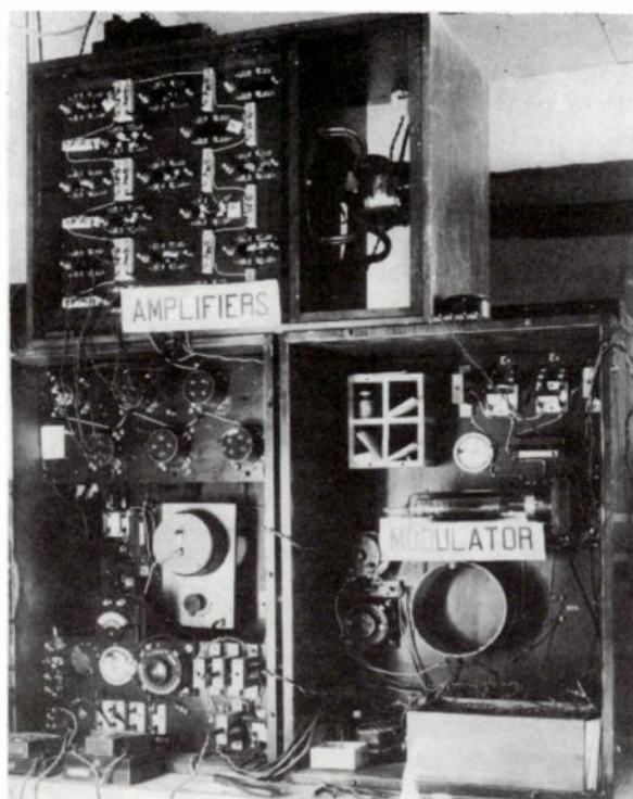
Fig. 6-28. The modulator panel at Arlington, Virginia, using a Type S or 204A vacuum tube as modulator.
