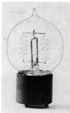
Fig. 8-6. Type CA Plotron, vintage 1917. This is a high-mu triode.
