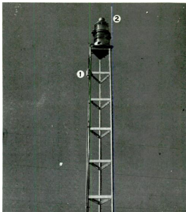
Fig. 7-7. A typical beacon installation. Notice the location of the junction box (1) and the lightning rod protector (2).
