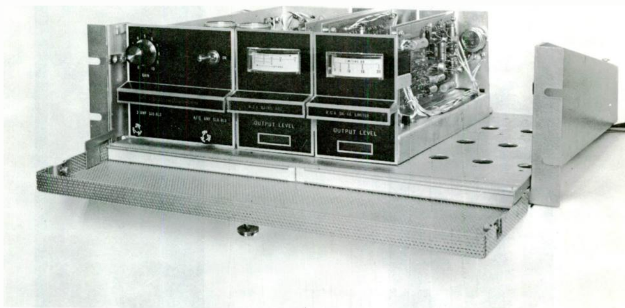
Fig. 10-13. Program amplifier shown with AGC and limiter units in a rack-mounting shelf.
