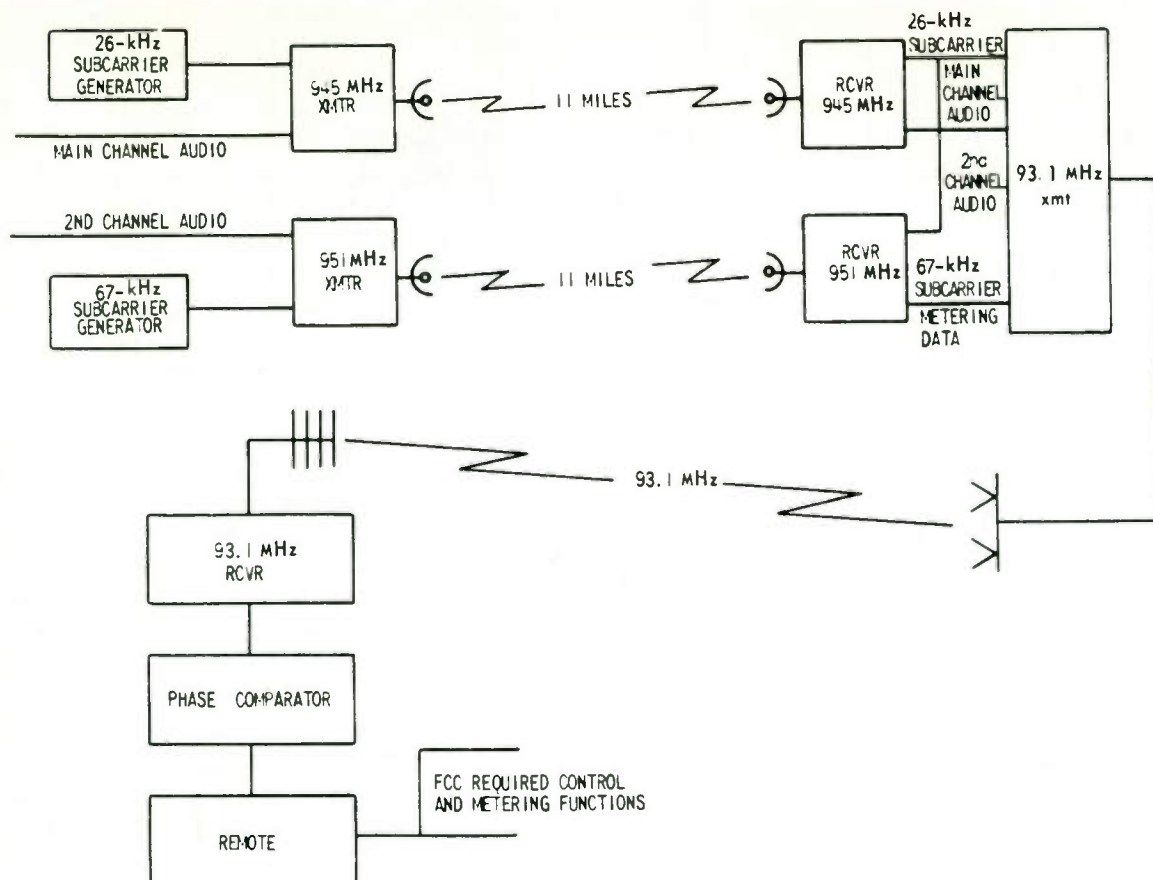
Fig. 9-5. Block diagram of a typical FM remote control system using an STL.
