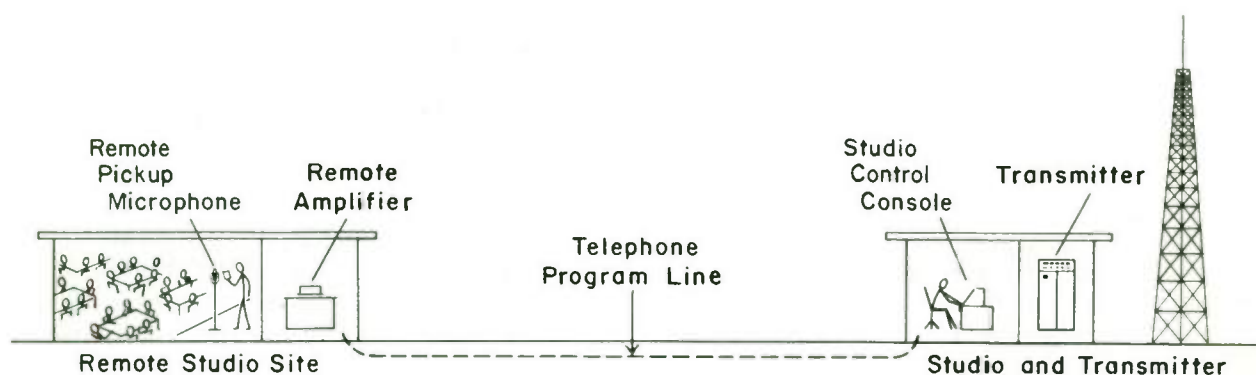
Fig. 1-5. Another variation in separate studio and transmitter facilities: Pickup and control equipment installed in public meeting places provides additional program sources.
