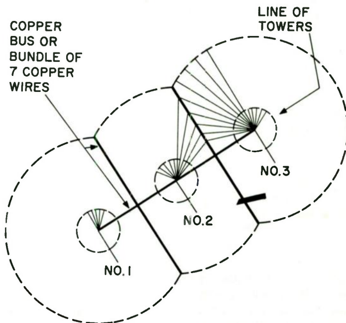
Fig. 7-20. Ground system diagram for a three-tower directional array showing, in part, ground radials which should be bonded in the main copper busses.
