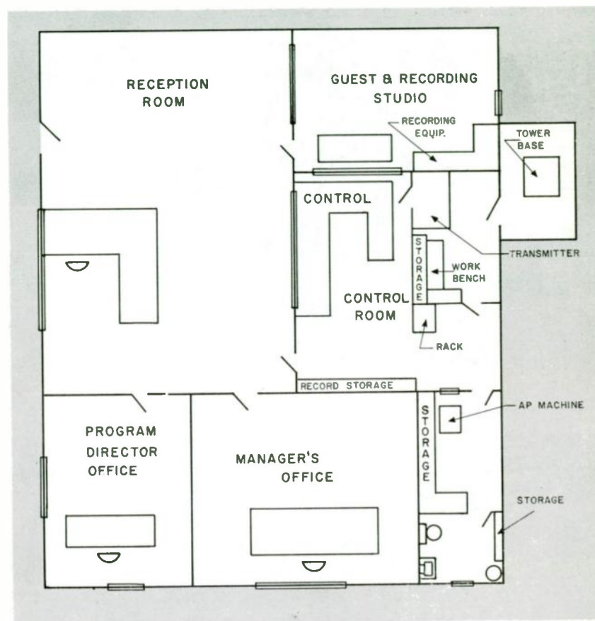
Fig. 16-18. Floor plan for WPHC's plant.
