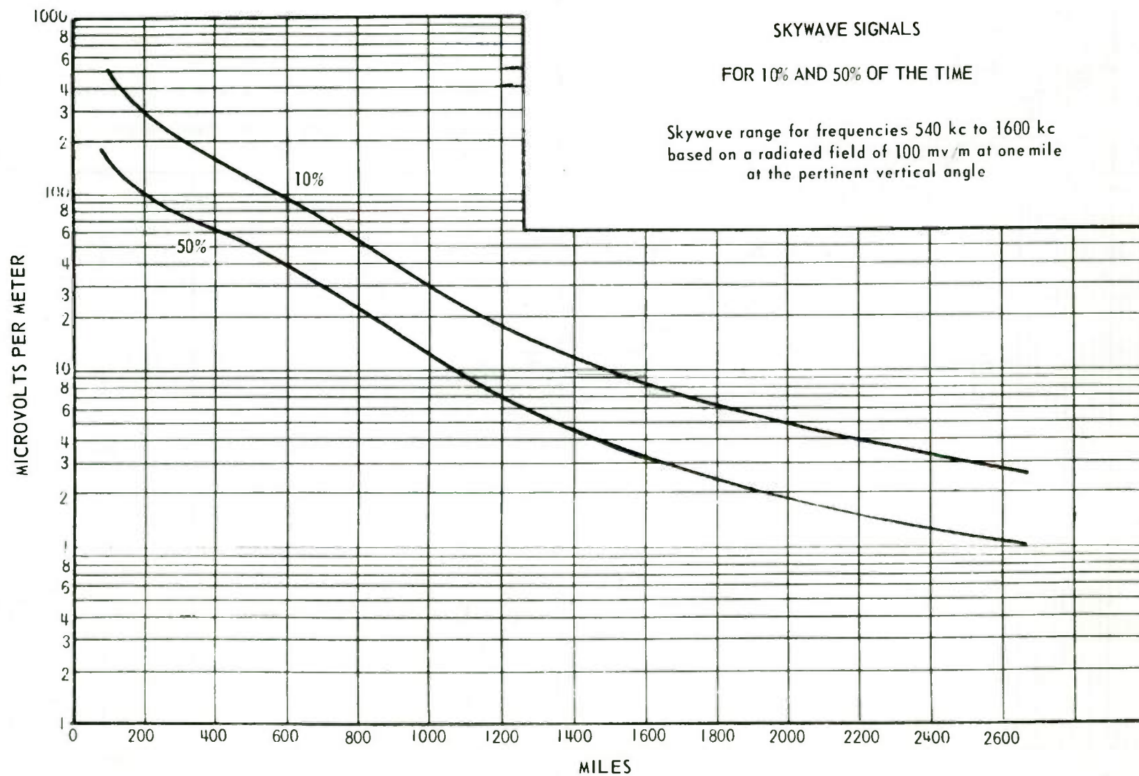
Fig. 2-5. Skywave signals for 10% and 50% of the time.
