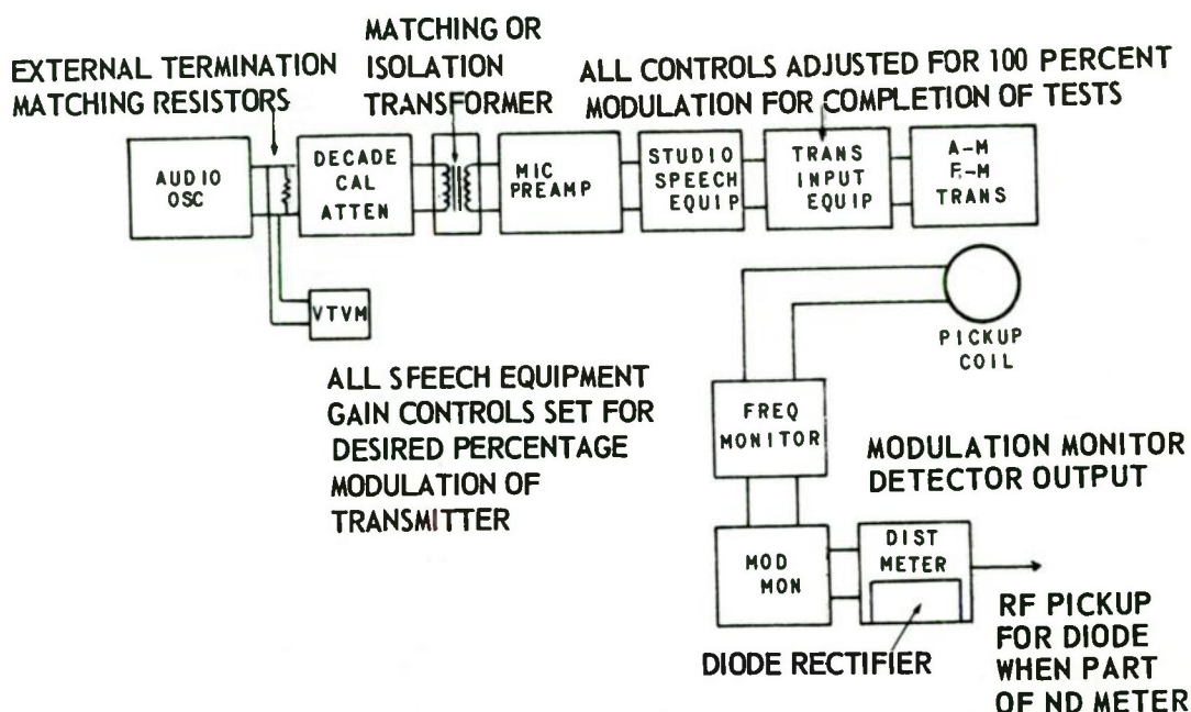
Fig. 15-2. Block diagram for complete proof-of-performance measurements.
