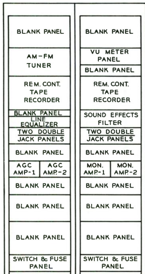
Fig. 4-14. Rack layout of the necessary equipment for the floor plan in Fig. 4-13.
