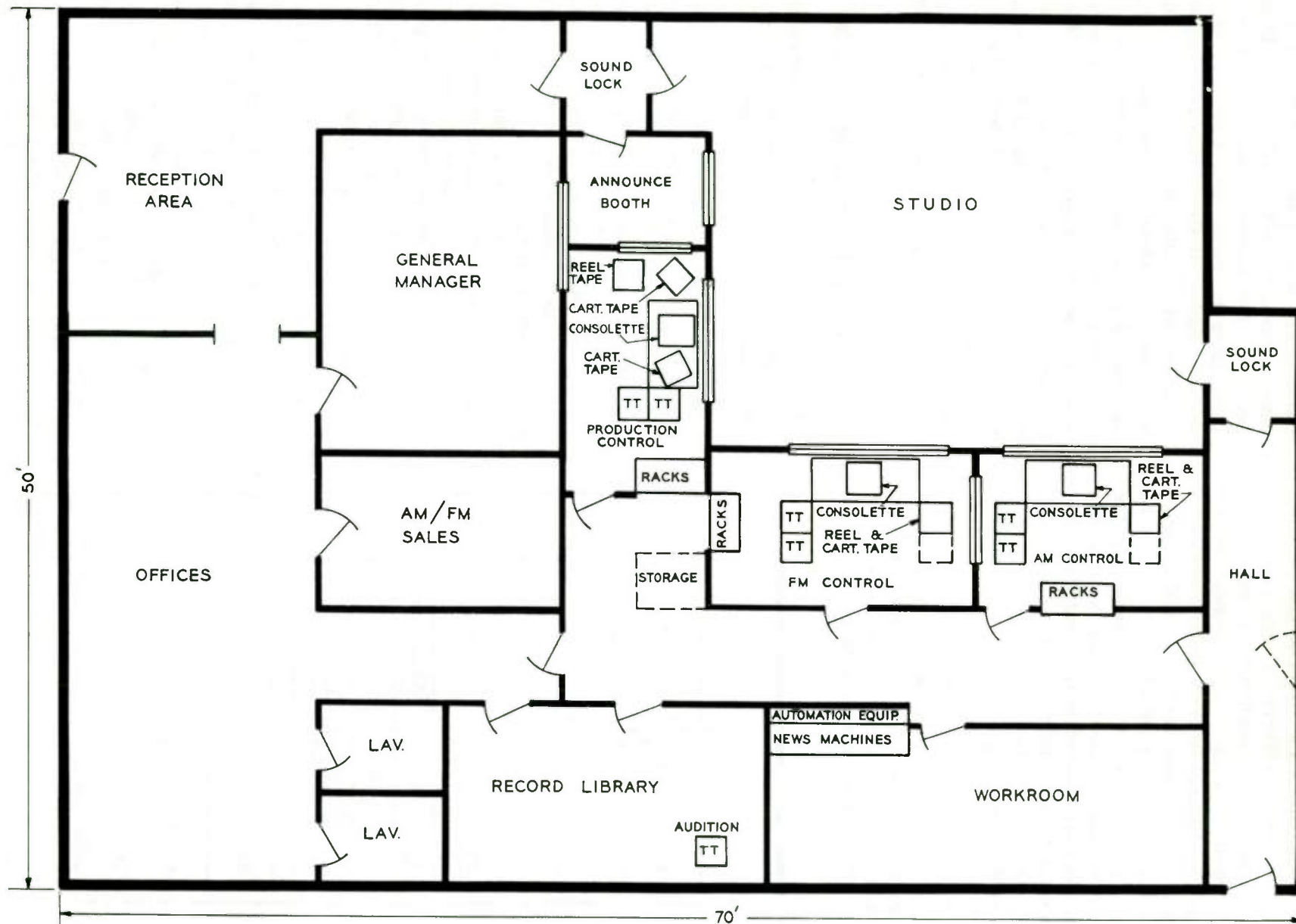
Fig. 4-15. Layout for a combined AM/FM broadcast facility.
