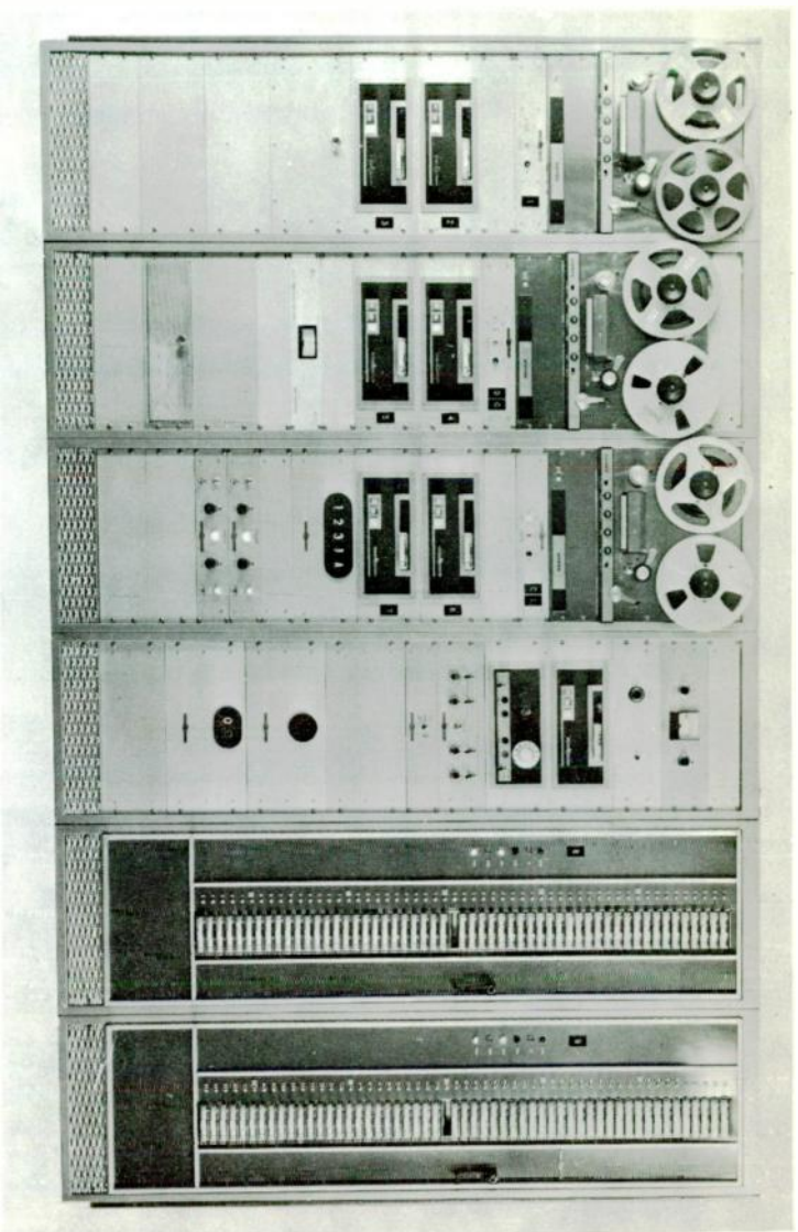
Fig. 11-12. WRKO's system employs reel-to-reel and cartridge tapes.
