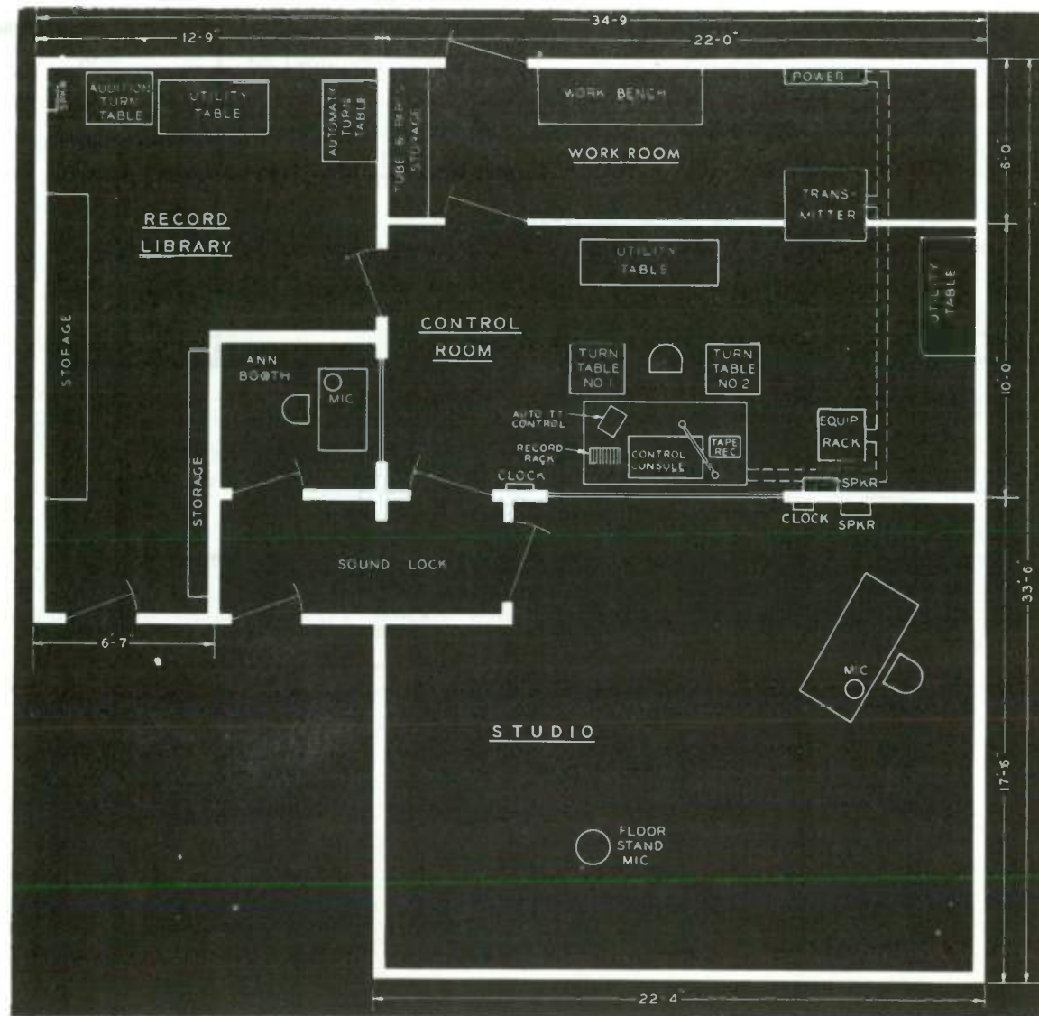
Fig. 4-7. Basic layout for a "Plan 2" facility.
