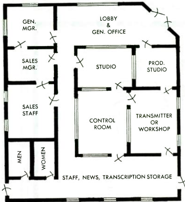
Fig. 4-3. "Plan 1" small-market, minimum-staff layout.
