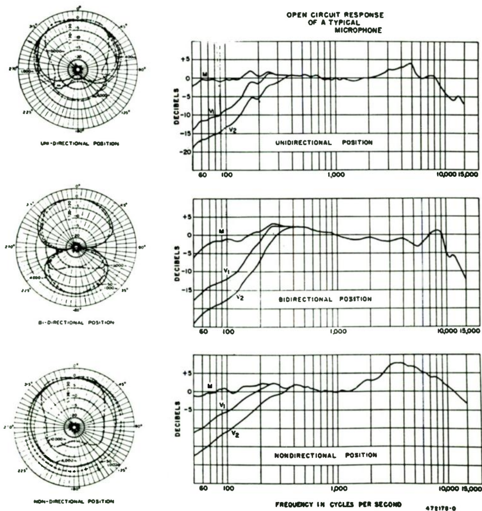
Fig. 12-3. Typical directional patterns and frequency response curves of a polydirectional microphone.
