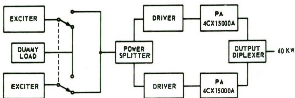
Fig. 13-5. Simplified block diagram of a 40-KW transmitter showing power splitter, diplexer, and switch for selecting either of two operating exciters.
