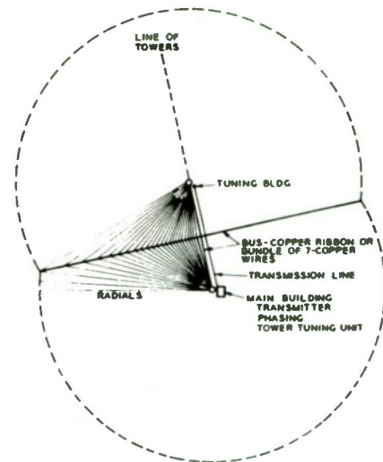
Fig. 3-5. Typical two-tower ground system.
