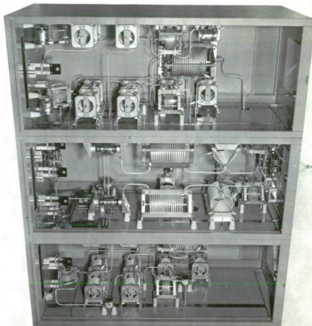
Fig. 7-11. Phasing equipment such as this is required for a directional antenna system.
