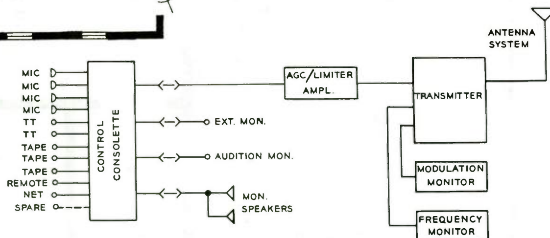
Fig. 4-5. Simplified block diagram of major equipment interconnections.
