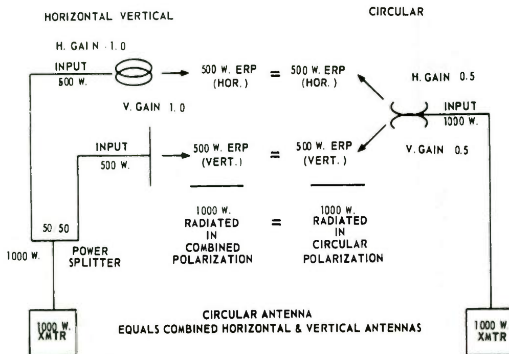
Fig. 8-9. Comparison of feed systems and the effective radiated power of a circularly-polarized antenna with combined horizontally and vertically polarized antennas. No power splitter is required for the circularly polarized antenna.
