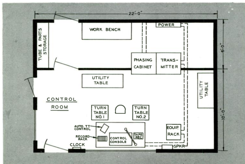
Fig. 5-1. This control room layout houses branching and phasing equipment.
