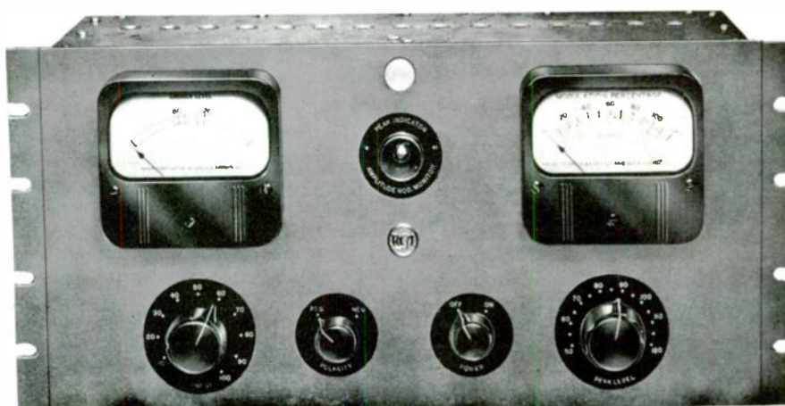
Fig. 10-19. AM modulation monitor.
