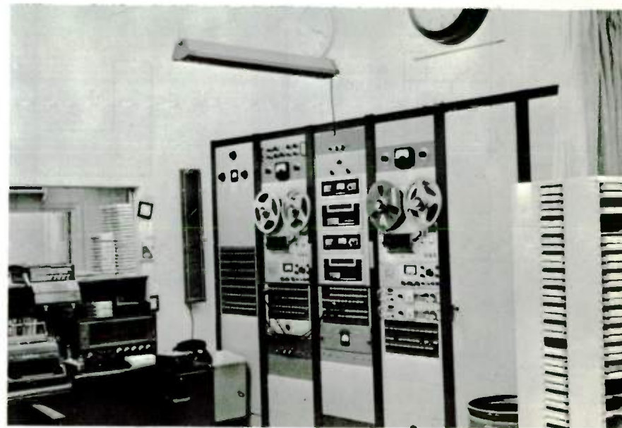
Fig. 16-15. Washington line recording racks in KYW's news gathering facilities.
