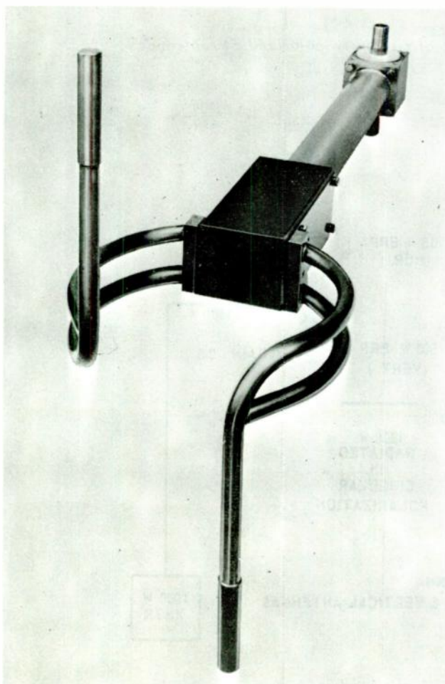
Fig. 8-7. A typical version of a circularly-polarized radiating element.
