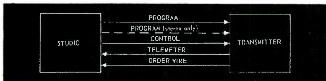
Fig. 9-6. Block diagram showing other STL remote control functions.
