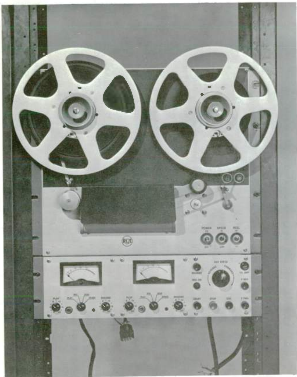
Fig. 11-4. A basic reel-to-reel audio tape recorder installed in a rack.
