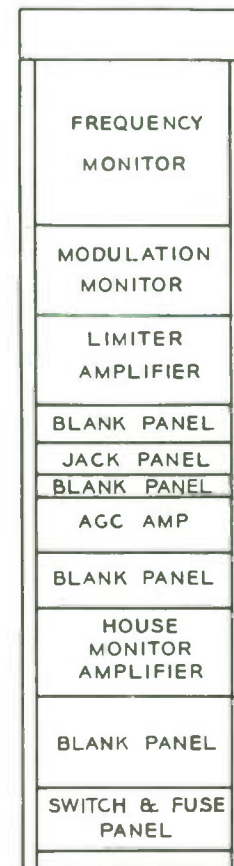
Fig. 4-8. This "Plan 2" rack layout includes a house monitoring amplifier.
