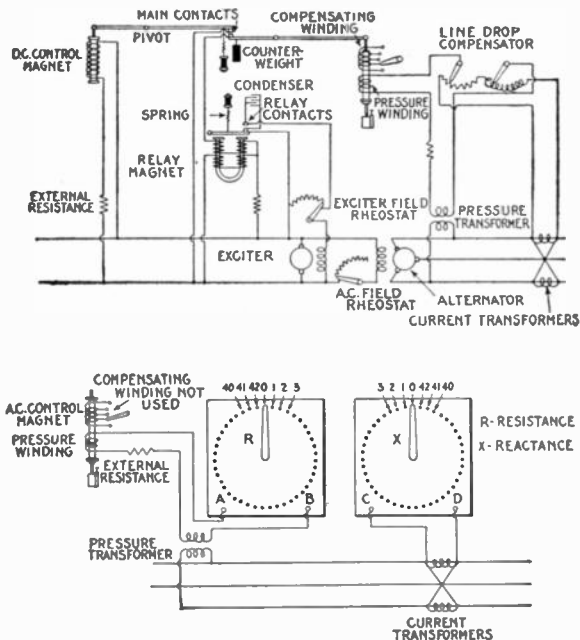
FIG. 2,462.—Diagram of automatic voltage regulator, using line drop compensator. For ordinary installations the compensating winding on the alternating current control magnet is connected to a current transformer in the main feeder. A dial switch is provided by which the strength of the alternating current control magnet can be varied and the regulator made to compensate for any desired line drop up to 15 per cent, according to the line requirements. Where the power factor of the load has a wide range of variation, a special line drop compensator, such as shown in fig. 2,459, adapted to the regulator would be desirable. The connections are readily understood by the diagram. The number of condenser sections which will prevent undue arcing at the relay contacts depends on the characteristics of the exciter. They may be roughly estimated by allowing one section for each 15 kw. capacity for exciters with laminated poles, and one for each 22 kw. capacity for exciters with solid steel poles. It is necessary though to have one condenser section for each pair of relay contacts, and at times it becomes necessary to apply a double section for each pair of contacts. In the lower part of the figure the line drop compensation and connections is reproduced in more detail on a larger scale.
