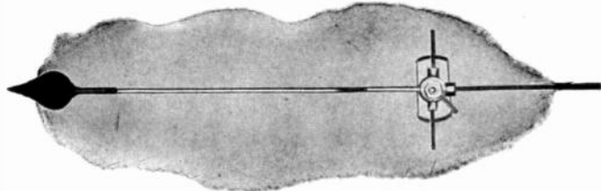
FIG. 2,492.—Wagner tubular aluminum pointer.
