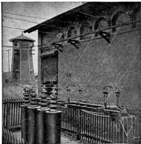
FIG. 2,397.—Highland Park sub-station, Charlotte, N. C., showing old lightning arrester tower on the left and General Electric aluminum (electrolytic) cell lightning arrester and horn gaps in foreground.
