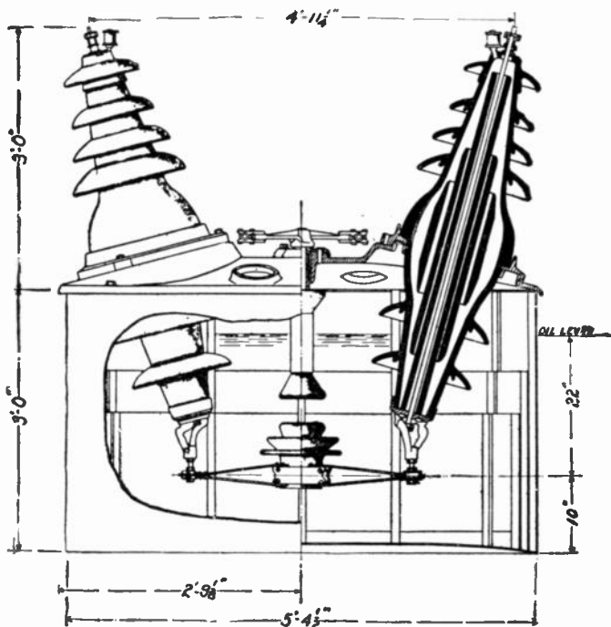
FIG. 2.221.—Sectional view of Pacific weatherproof oil switch for use in places exposed to the weather. All moving and contact parts are supported from the cast iron top and are readily removable for inspection or repair
