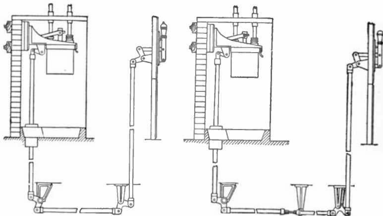
FIGS. 2,228 and 2,229.—Views showing mechanism of hand operated remote control switches. Fig. 2,228, straight mechanism; fig. 2,229, angular mechanism.
