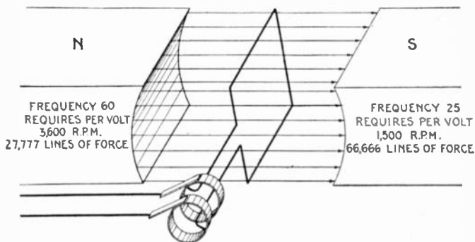
FIG. 2,149.—Elementary alternator developing one volt at frequencies of 60 and 25, showing the effect of reducing the frequency. Since for the same number of pole, the R.P.M. have to be decreased to decrease the frequency, increased flux is required to develop the same voltage. Hence in construction, low frequency machines require larger magnets, increased number of turns in series on the armature coils, larger exciting units as compared with machines built for higher frequency.
