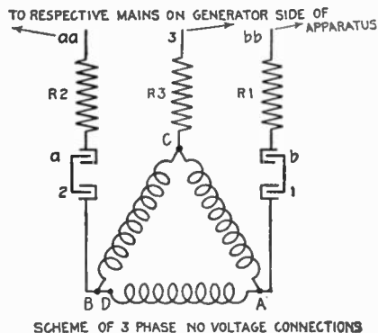
FIG. 2,336 and 2,337.—Diagram showing three phase no voltage connections for I-T-E circuit breaker. The no voltage coils for three phase circuits are connected in \Delta by means of binding posts A, B, C and D on the face of the base, and from the A and B of the no voltage coils, connections are made respectively to spring contacts 1 and 2 of the small disconnecting switch. Each of the contacts a and b of the disconnecting switch is connected respectively through resistance R 2 and R 1 to one of the mains at aa and bb . The terminal C is connected through resistance R 3 on the back of the board to the middle main as shown at point 3. The terminal D is linked on the back of the board to terminal B to complete the \Delta connection. The terminals aa , bb and 3 of the circuit breaker must, in all cases, be so connected that they will be subject to full voltage of the circuit irrespective of the position of the starting switch. Each no voltage coil is supplied with two terminal wires, one covered with green and one with black insulation. In replacing these coils particular care should be taken to see that the terminal wires connected to any one binding post are of unlike color.
