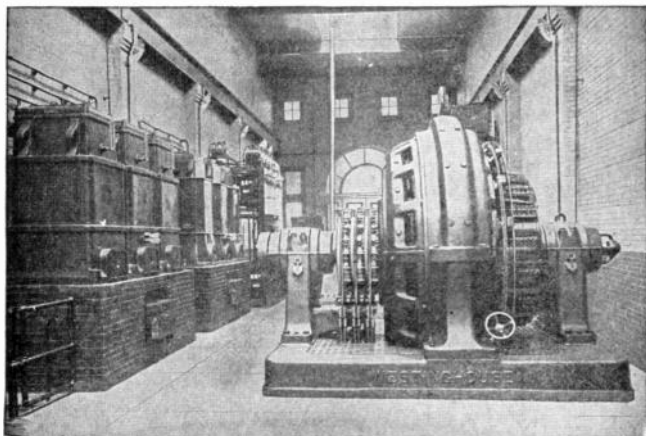
FIG. 2,198.--Example of converter sub-station, showing the Brooklyn Edison Co. Madison sub-station. The transformers are seen on the left, the converter shown at the right is a Westinghouse synchronous booster rotary converter, consisting of a standard rotary converter in combination with a revolving armature alternator mounted on the same shaft with the converter and having the same number of pole. The function of the machine is to convert and regulate the pressure. By varying the field excitation of the alternator, the A.C. voltage impressed on the rotary converter proper can be increased or decreased as desired. Thus, the D.C. voltage delivered by the converter is varied accordingly. This type of converter is well adapted for any application for which a relatively wide variation, either automatic or non-automatic, in direct current voltage is necessary. Also especially for serving incandescent lighting systems where considerable voltage variation is required for the compensation of drop in long feeders, for operation in parallel with storage batteries and for electrolytic work where extreme variations in voltage are required by changes in the resistance of the electrolytic cells.
