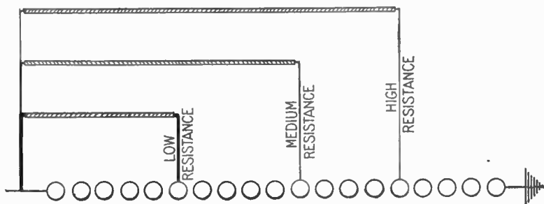
FIG. 2,358.—Arrangement of graded resistances on multigap arrester.
