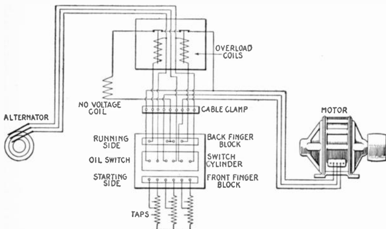
FIG. 2,468. —Diagram of connections of General Electric three phase starting compensator with no voltage release and overload relays.
