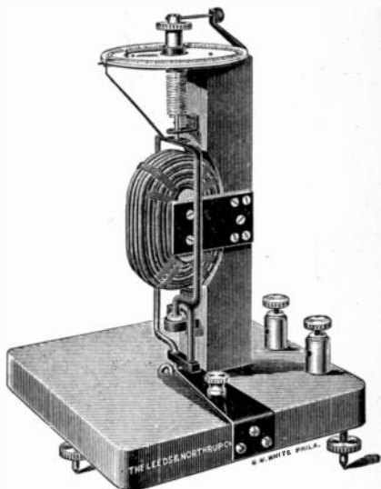
FIG. 2519.—Leeds and Northrup electro-dynamometer. It is a reliable instrument for the measurement of alternating currents of commercial frequencies. When wound with fine wire and used in connection with properly wound resistances, it is equally useful for measuring alternating pressures, and may thus be employed to calibrate alternating current voltmeters as well as ammeters. To give accurate results the instruments must be carefully constructed and designed with a view to avoiding the eddy currents always set up by alternating currents in masses of metal near, or in the circuits. The constant of a dynamometer may be obtained with a potentiometer, but this is usually done with precision by the manufacturer and a certificate giving the value of the constant is furnished with the instrument. The size and cost of dynamometers rapidly increase with the maximum currents which they are designed to carry, and when more than 500 amperes are to be measured, the use of other instruments and methods is recommended.
