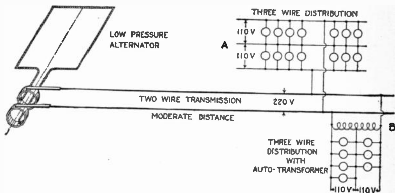
FIG. 2,143.—Diagram illustrating single phase two wire transmission and three wire distribution. The simplified three wire arrangement at A, is not permissible except in cases of very little unbalancing . Where the difference between loads on each side of the neutral may be great some form of balancing as an auto-transformer or equivalent should be used, as at B.
