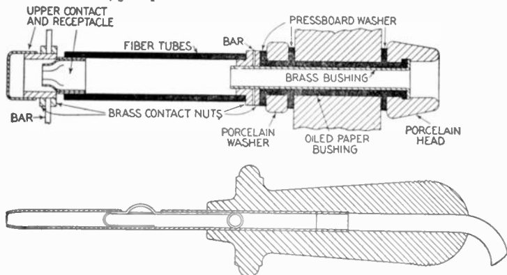
FIG. 2,203 and 2,204.—Bus transfer plug switch. The method of supporting the contact farthest from the panel consists of a porcelain pillar of the same height as the receptacle, clamped to a brass connecting or bus bar which in turn is fastened to the receptacle.
