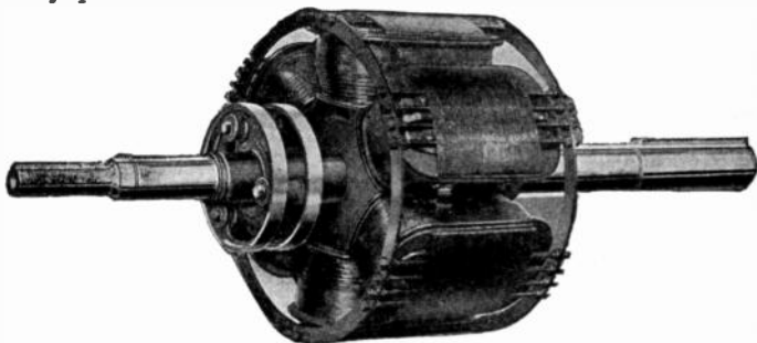
FIG. 2,481.—Field of a synchronous condenser. Note the amortisseur winding, erroneously called squirrel cage winding, consisting of two end rings which serve to short circuit spokes passing through the pole tips as shown. The amortisseur winding assists in starting and serves also as a damping device to minimize hunting.
