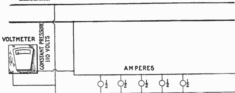
FIG. 2,136. —Diagram of parallel circuit. It is a constant pressure circuit and is very widely used for lighting and power. If each lamp take say \frac{1}{2} ampere, the current flowing in the circuit will vary with the number of lamp in operation; in the above circuit with all lamps on, the current is \frac{1}{2} \times 5 = 2\frac{1}{2} amperes.
