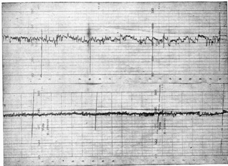
FIG. 2.483. —Curve drawing voltmeter records at Kennett, Cal. The upper curve shows voltage regulation with synchronous condenser out of service, and the lower curve, with synchronous condenser in operation.
