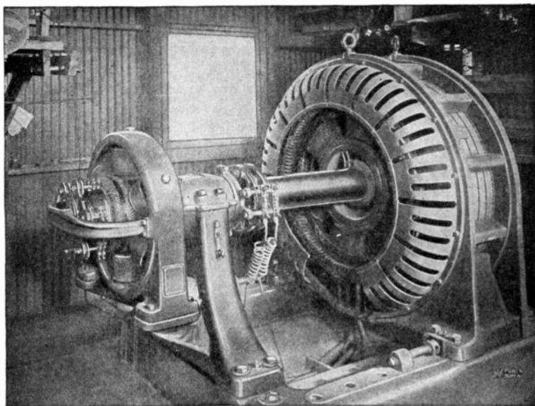
FIG. 2,479.—General Electric 400 kw., 550 volt, 600 R.P.M., synchronous condenser with direct connected exciter installed in sub-station No. 1 of the Colorado Light & Power Co., Cripple Creek, Colo. The machine is designed for alternating current starting by means of a compensator. The field is provided with a standard synchronous motor winding, and, in addition, an amortisseur winding which assists in starting and serves as a damping device to minimize hunting.
