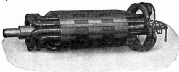
FIG. 2,417.—Moving element or primary of Westinghouse motor operated single phase induction regulator. It consists of a core of punchings built up directly on the primary shaft and carrying the primary winding, which is divided into four coils. The primary coils are machine wound and the layers of the winding are separated from each other by heavy insulating material in addition to the cotton covering of the inductors. The complete coils are insulated and impregnated with insulating compound before being placed in the slots. The coils are held in position by fibre wedges.
