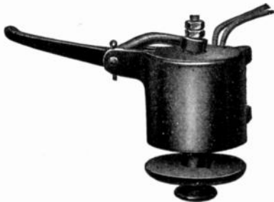
FIG. 2,272.—General Electric low voltage attachment for circuit breakers. This low voltage trip is designed to operate the circuit breaker when the line voltage drops to approximately 50 per cent or less of the normal voltage. It should be noted that the coil is always in circuit, as is the case with the overload and underload coils, and that it operates with the releasing of its armature. It is always necessary to use a fixed amount of resistance (depending upon the voltage of the system) in series with the low voltage release. The low voltage release performs the functions of a shunt trip coil when used in conjunction with a push button, auxiliary switch or speed limiting device, and is generally preferred to the shunt trip attachment.
