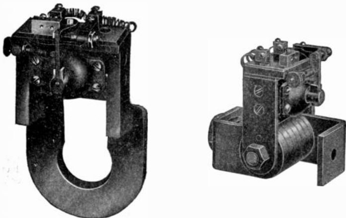
FIGS. 2,338 and 2,339.—General Electric instantaneous direct current reverse current or “discriminating” relays. Fig. 2,338, for 500 amperes; fig. 2,339 for 2,000 amperes. These relays are designed for mounting directly on circuit breaker studs. These relays consist of a horseshoe magnet with a shunt wound armature pivoted between its poles. The magnet is mounted on the current carrying stud of the circuit breaker between the back of the panel and the first contact or supporting nut, and is placed in a vertical position. The contacts are insulated from the magnet permitting the use of an auxiliary circuit for the tripping device, independent of the circuit controlled by the circuit breaker. The magnet is excited by the current flowing through the stud, and the armature is connected across the line in series with suitable resistance. Rotation of the armature in the normal direction is prevented by a stop. Reversal of the current flowing through the stud changes the direction in which the armature tends to rotate, causing it to move away from the stop and close the circuit through an auxiliary trip coil and trip the circuit breaker. These relays are used to protect dynamos, storage batteries, or main station busses from damage on reversal of current due to short circuit, or from the grounding of machines or connection. Relay contacts must not be used to open the shunt trip coil circuits. An auxiliary switch should be provided for this purpose in all cases where the opening of the circuit breaker does not disconnect the trip coil from the source of supply.
