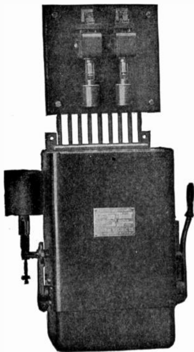
FIG. 2,460.—General Electric starting compensator with low voltage release and overload relays. On the switch shaft there are mounted two levers, held together with a strong spring which operates in either direction and prevents the switch being left on the starting position. On the running side it is held by the external low voltage release lever until released either by hand or by the action of a low voltage relay. The low voltage release consists of a cast iron frame open at the bottom and totally enclosing the coil. A laminated plunger is used to hold the tripping lever, the latter engaging with the lever mounted on the switch shaft. The compensator cannot be thrown into the running position without first going to the starting position and it cannot be left on the starting position.
