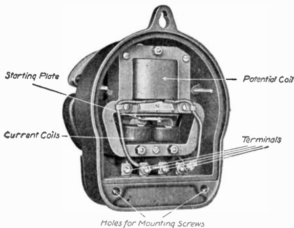
FIG. 2,543. —Rear view of Port Wayne single phase induction watt-hour meter with back cover plate removed. The pressure and current coils and their respective cores lie behind the main frame of the meter. This complete electromagnetic unit can be removed as a whole from its mounting in the case. The pressure coil is wound from enameled wire, the number of turns being very high. The current coils have but few turns each and are wound from cotton covered wire. All coils are heated with insulating compound before assembling in the meters. The laminated iron cores placed within these coils are built up from magnetic steel. The magnetic circuits formed by the cores of the pressure and current coils are so arranged that they exert a high torque upon the disc of the rotating element in order that minute variations in the friction of the moving parts, which are likely to occur will not cause any appreciable error in the registration of the meter. The iron case surrounding the electrical elements protect that part of the meter from the effects of external stray fields, while the astatic arrangement of the permanent magnets tends to prevent any influence on the damping system. The fact that the iron frame of the meter lies between the permanent magnets and the current coils protects the magnets from the effects of short circuits which create a strong magnetic field within the meter itself.
