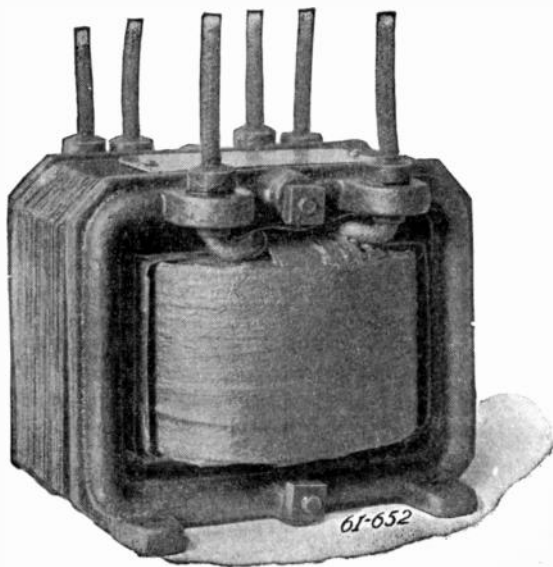
FIG. 2,516.—Wagner 25 watt pressure transformer for use with various alternating current instruments, such as voltmeters, wattmeters, etc. They are made in capacities 25, 50, 100, and 200 watts, and are built for pressures of 750 to 60,000 volts.
