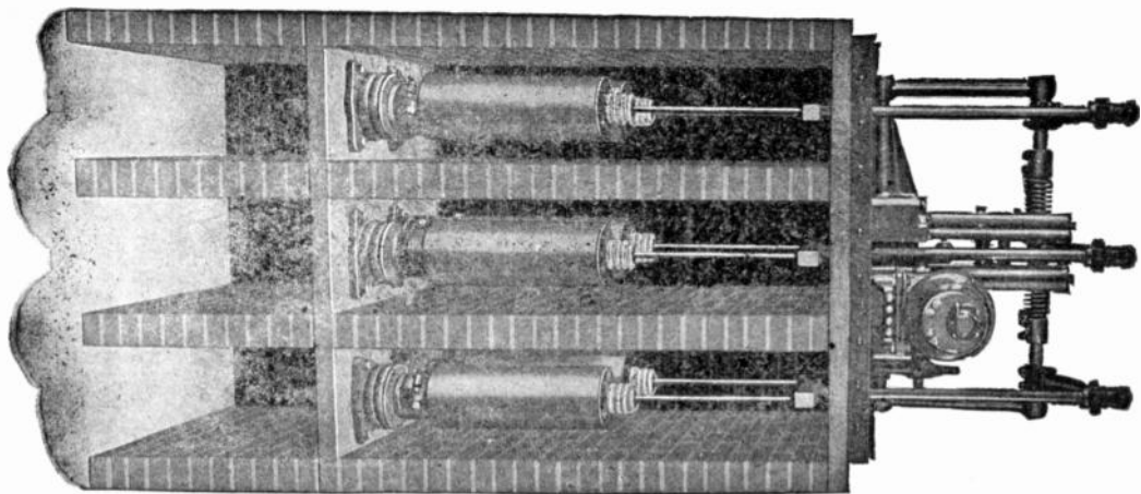
FIG. 2,232. —General Electric motor operated three phase oil switch. The operation of the oil switch is accomplished by a small hand controlling switch, generally mounted on the panel, with the instruments which are in the circuit controlled by the oil switch. The standard pressure for the operating motor is 125 volts. The switch has six breaks, each break being in a separate tank. In addition to this isolation of the breaks, each phase is enclosed in a fireproof brick compartment, making it impossible for trouble in one phase to be communicated to another. The cells are constructed of brick with top and bottom slabs of slate. The capacities of such switches, range from 2,500 to 60,000 volts, and from 100 to 1,000 amperes.
