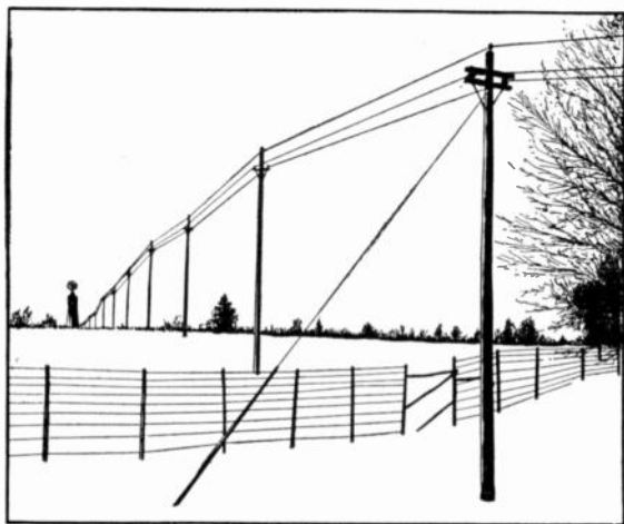
FIG. 2,194.—View of a three phase, 2,300 volt, 60 cycle line at Chazy, N. Y. The current is transmitted at the alternator voltage 2\frac{3}{4} miles over the single circuit pole line. The poles are of cedar with fir cross arms, and are fitted with pin insulators. They are from 35 to 40 feet high and are spaced at an average of about 120 feet. The conductors are bare copper wire No. 00 B. & S. The alternators consist of one 50 kw., and one 100 kw. General Electric machines.
