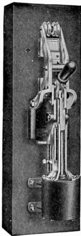
FIG. 2,331.—Condit 600 volt, 1,510 ampere, single pole type K circuit breaker pneumatically operated . It is the same as the electrically operated circuit breaker, except that a pneumatic cylinder mechanism is supplied in place of either the electromagnet or the motor. This cylinder mechanism is so arranged that the air pressure
