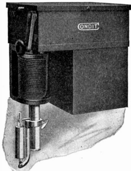
FIG. 2310. —Condit type "B" time limit attachment, designed to give sufficient time to allow an induction motor to start without opening the circuit breaker, and not have the circuit breaker trip on the momentary rush of current. Its action is inverse; that is, the greater the current the less time it takes to operate and is so arranged that four to five times full load current or a short circuit will trip the circuit breaker instantly. The time limit attachment is applied directly to the armature which trips the circuit breaker and is adapted for the so called primary trip. It consists of an air vacuum dash pot with a graphite piston, the dash pot being fastened to the stationary calibrating ring of the trip coil and the moving outside cylinder is fastened to the armature of the circuit breaker. When the current reaches a point where it overcomes the weight of the armature and lifts the same, the magnetic force tending to raise the armature is opposed by the vacuum created in the interior of the cylinder. As the magnetic force continues, the vacuum is overcome due to the leakage of air past the plunger and the armature gradually moves up until it reaches the point where it trips the circuit breaker. If at any point of the armature travel, the current drop back to normal, the armature immediately resets itself by means of a ball valve in the top of the brass cylinder
