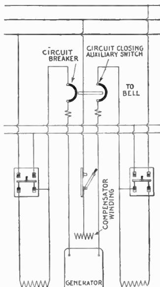
FIG. 2,348.—Diagram showing three wire dynamo protected by double pole double coil over-load circuit breaker (or two single pole breakers with interlock) with bell alarm switches. Complete protection is secured as breaker is connected between armature and series field.
