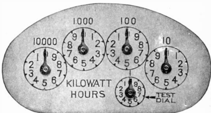
FIG. 2,550.—Canadian dial of Sangamo single phase induction watt hour meter. It has a small test circle indicating one kilowatt hour per revolution in all sizes where the first regular circle indicates 10. This is provided to conform with the requirements of the Canadian government and it is intended that the hand on the test circle shall make not less than \frac{1}{2} revolution in one hour with full load on a meter. In the case of a 10 ampere meter, it will make one complete revolution in one hour and for a 20 ampere, two revolutions, and so on. The train or indicating mechanism is carried on a rigidly formed and swaged brass bracket, accurately located by two dowel pins set in the top face of the main grid, and is held to the grid with two screws easily accessible when it is desired to remove the train for any purpose. All indicating trains used on type "H" meters are marked with symbols on the back of the train and on the compound attachment to indicate the gear ratio of each combination; this ratio being different for meters of different capacities in order to obtain a direct reading in kilowatt hours on the dial.
