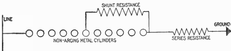
FIG. 2,350.—Low equivalent arrester. This is a modification of the multi-gap arrester shown in fig. 2,349. About half of the total number of gaps are shunted by a resistance, and another resistance is inserted between the cylinders and the earth. With this arrangement the middle point is at ground pressure, and there are between line and ground only one half of the total number of gaps. This is sufficient to prevent a bridging of the gaps under normal conditions.
