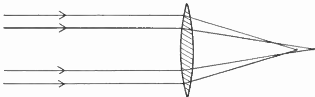
FIG. 15.—Rays from the outer edge of a simple lens whose surfaces are spherical focus closer to the lens than those through the center portion. This gives a blurred image.
