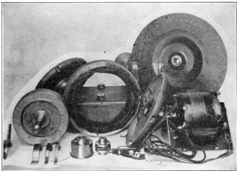
FIG. 108.—Assembly of scanning-disc motor used by Bell apparatus.
