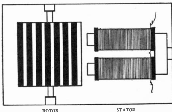
FIG. 55.—Simple phonic drum. This illustrates the fundamental construction of a synchronous A. C. motor.
