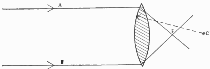
FIG. 13.—The diagram above shows the path of parallel rays which after refraction by the lens pass through the focus. C is the center of curvature for one face of the lens.
