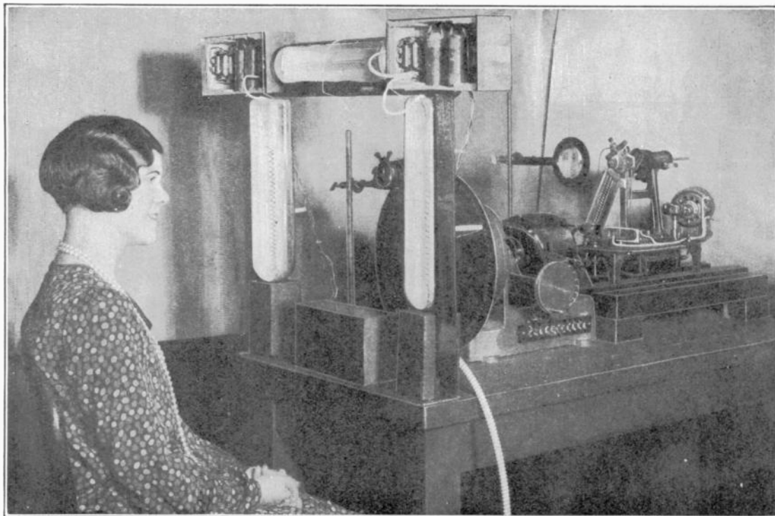
FIG. 90.—The transmitting apparatus used in the Bell system demonstration.
