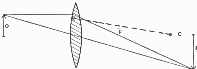
FIG. 14 a .—The above is typical of the position of object and image for a double convex lens when the object is outside the focus. This will be the case in most television apparatus.
