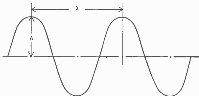
FIG. 20.—This shows a typical wave form, where \lambda is the wave-length and A , the amplitude.
