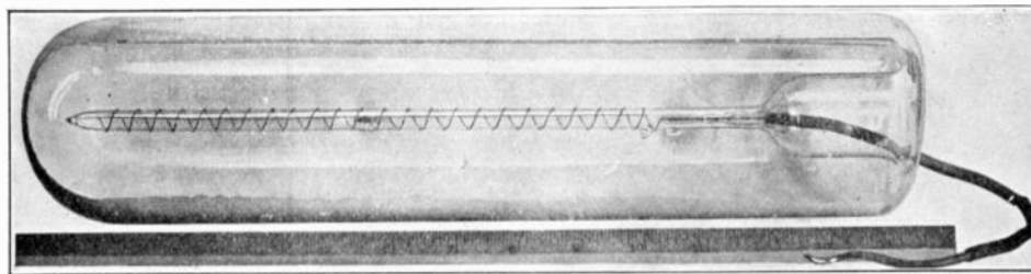
FIG. 92.—Detail of a photoelectric cell of the type used in the Bell apparatus. Note large area of photo-sensitive coating.
