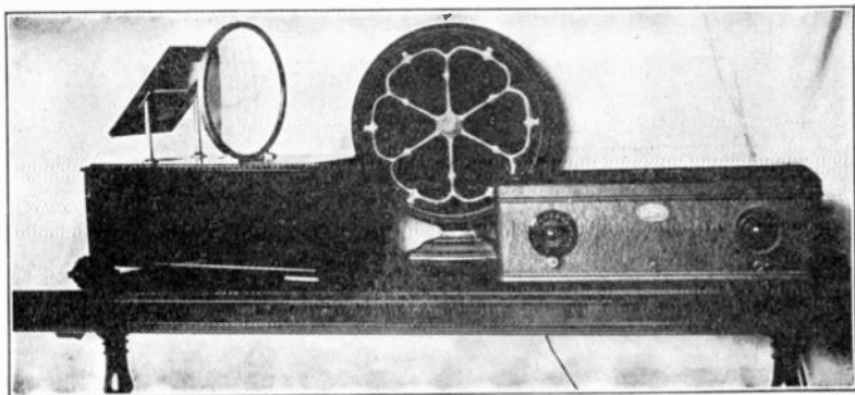
FIG. 119.—Complete radio and radio-movies equipment. Note comparative size.
