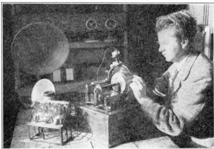
FIG. 87.—A phonovisor, in which the television sounds are recorded on a cylinder, as in a phonograph, later to be re-created into a picture at any time desired.
