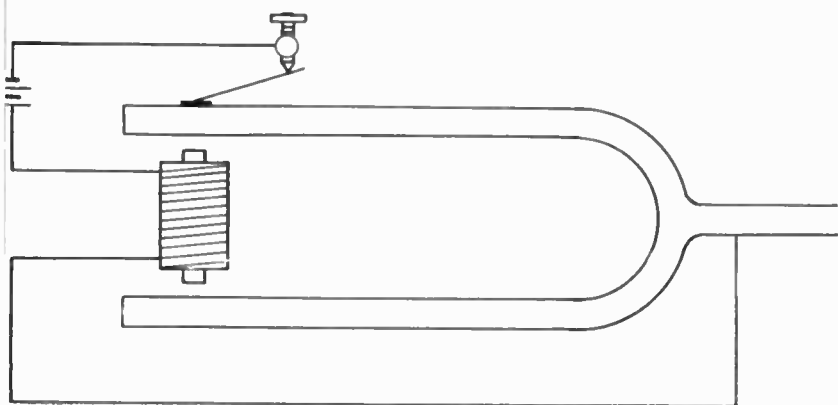
FIG. 52.—Electrically driven tuning fork.
