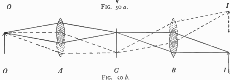
FIG. 50.—Moving a single lens will displace the image I as shown in a , but moving two lenses A and B in opposite directions will give a greater displacement as shown. B picks up the image from the ground glass screen G .
