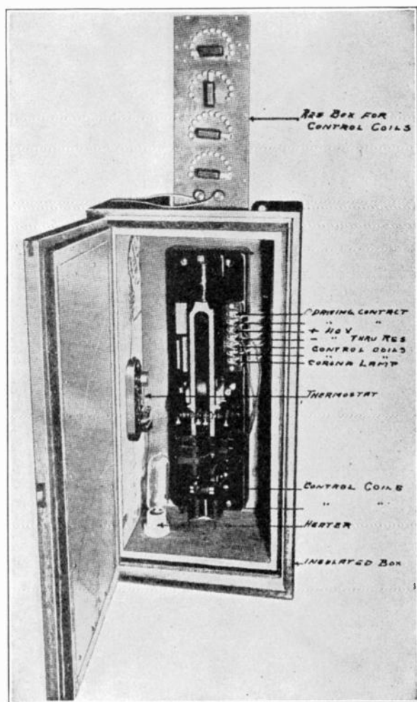
FIG. 54.—Mounting of synchronizing tuning fork in constant temperature box, Ranger system.
