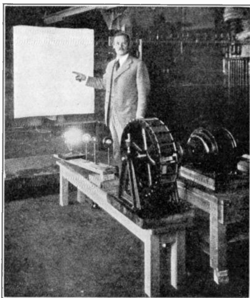
FIG. 120.—The Alexander projection drum.
