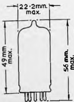
B9A Noval Base
