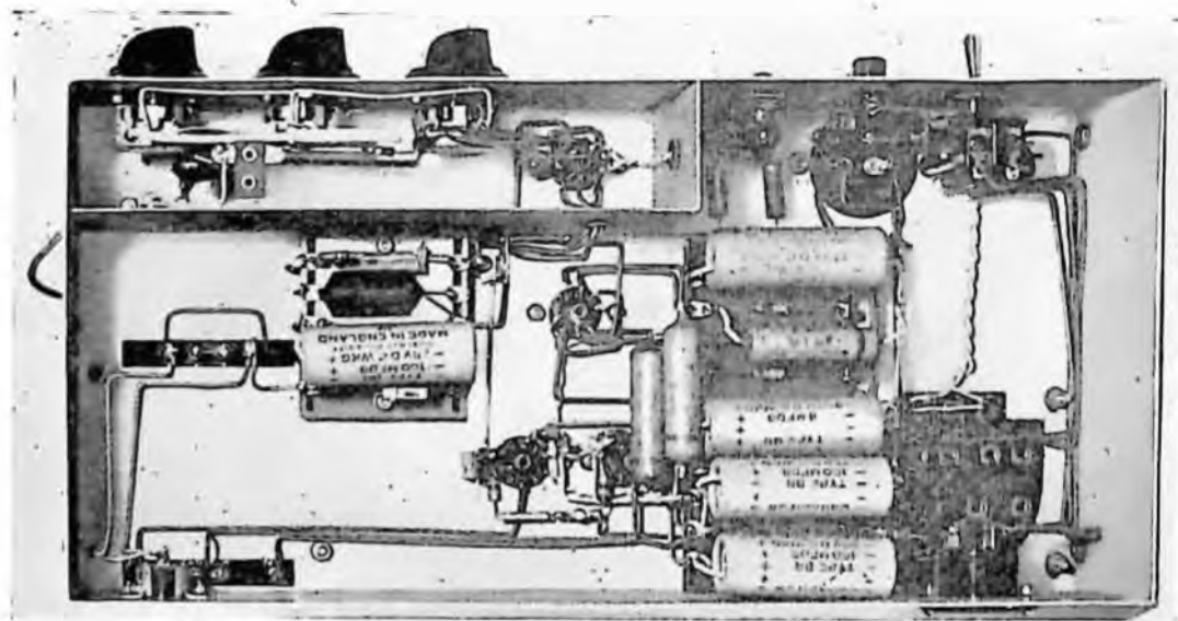
UNDER CHASSIS VIEW OF AMPLIFIER BUILT TO RECOMMENDED LAYOUT
