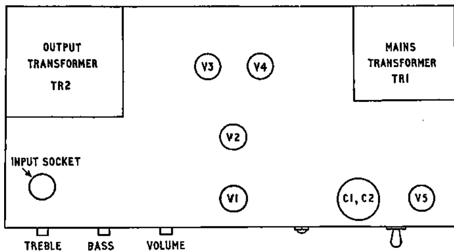
TOP CHASSIS VIEW OF RECOMMENDED LAYOUT
