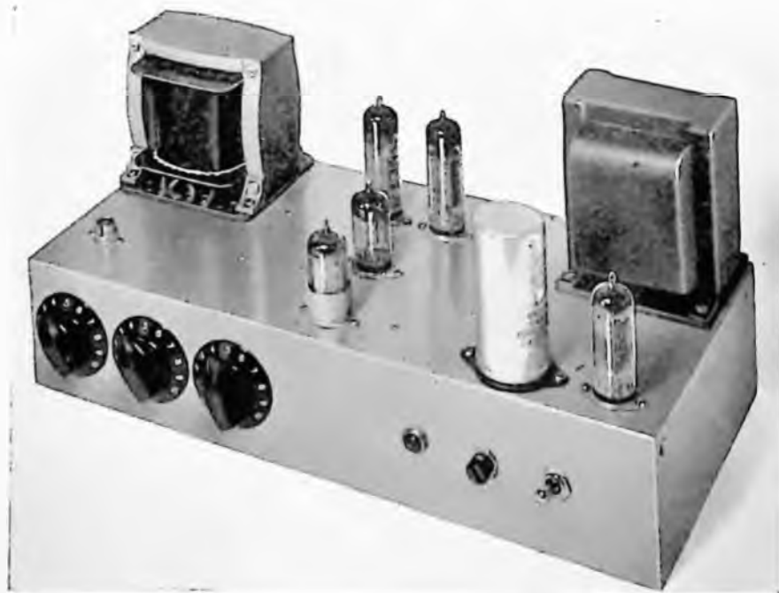
VIEW OF AMPLIFIER BUILT TO RECOMMENDED LAYOUT WITH PERFORATED COVER REMOVED. THIS PARTICULAR MODEL HAS BEEN CONSTRUCTED WITH AN EZ80 RECTIFIER (V5)
