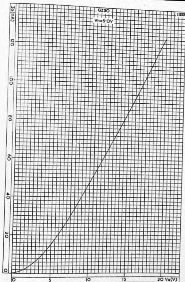
ANODE CURRENT PLOTTED AGAINST ANODE VOLTAGE
