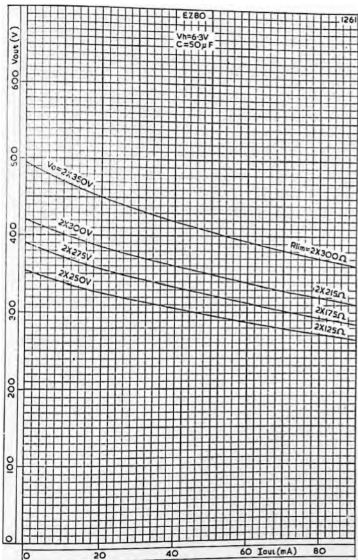
REGULATION CURVES
