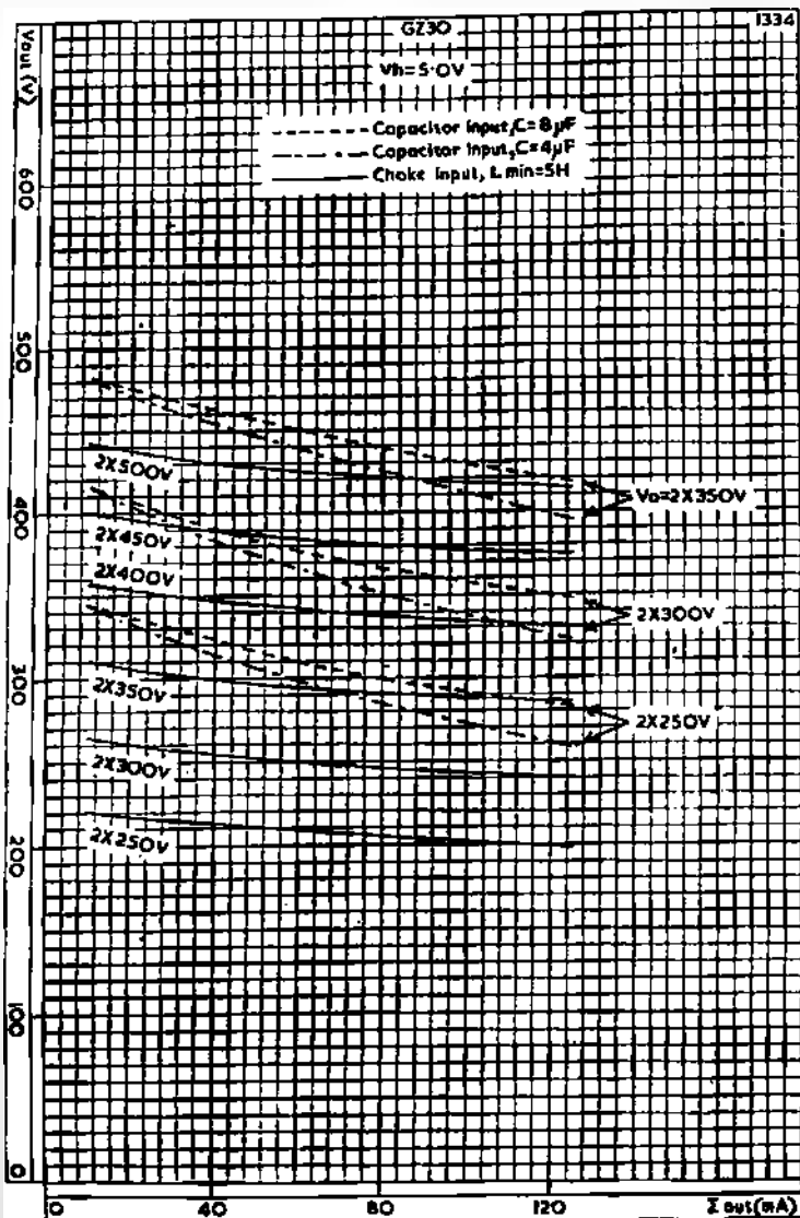
REGULATION CURVES FOR CAPACITOR OR CHOKE INPUT
