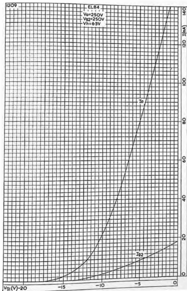
ANODE AND SCREEN-GRID CURRENT PLOTTED AGAINST CONTROL-BIAS
