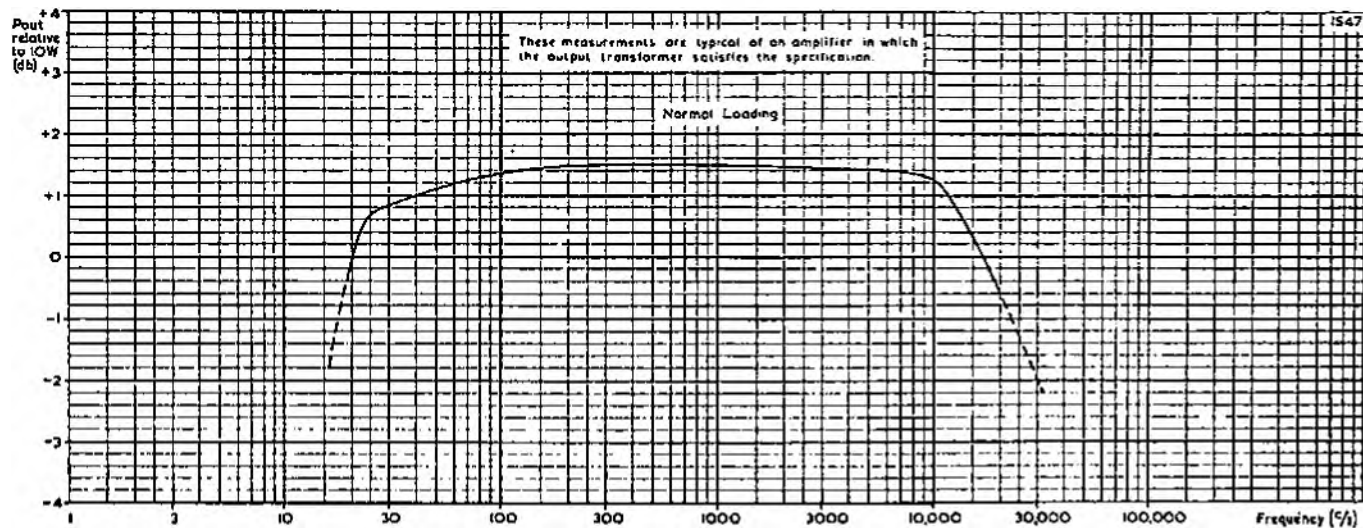
FIG. 2 MAXIMUM OUTPUT POWER RELATIVE TO 10 WATTS PLOTTED AGAINST FREQUENCY
