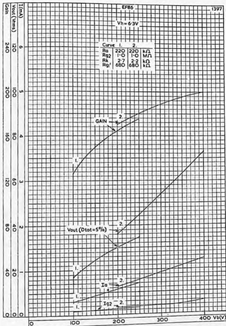
PERFORMANCE OF EF86 AS PENTODE CONNECTED R.C. COUPLED AMPLIFIER PLOTTED AGAINST LINE VOLTAGE, FOR R_a=220k\Omega .
