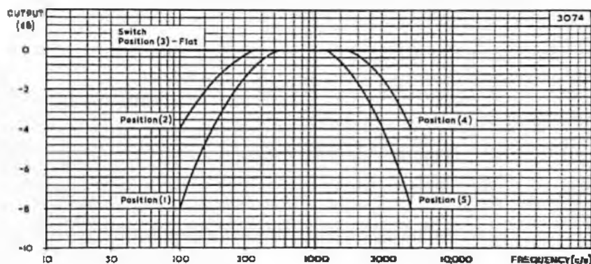
Fig. 30—TONE-CONTROL CHARACTERISTIC; TAPE SPEED 3\frac{1}{2} IN./SEC
