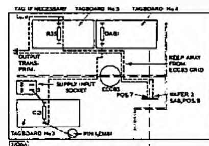
Fig. 21—H.T. SUPPLY FOR EL84
