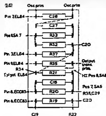
Fig. 20—TAGBOARD No. 5
