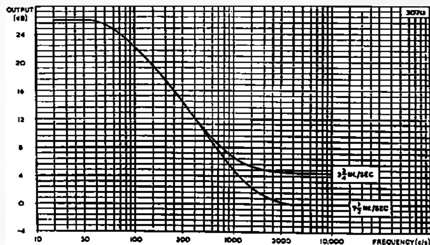
Fig. 28—BASS BOOST CHARACTERISTICS
