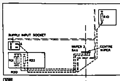
Fig. 14—H.T. SUPPLY FOR EM81
