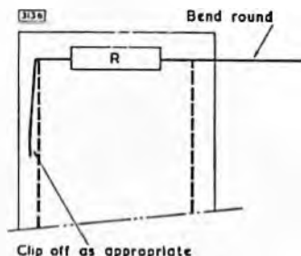
Fig. 7—MOUNTING OF SMALL COMPONENTS
