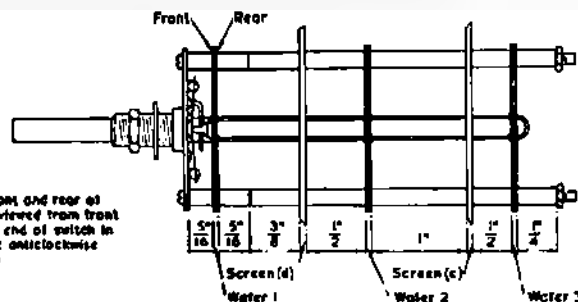
Fig. 5—RECORD/PLAYBACK SWITCH DETAILS
