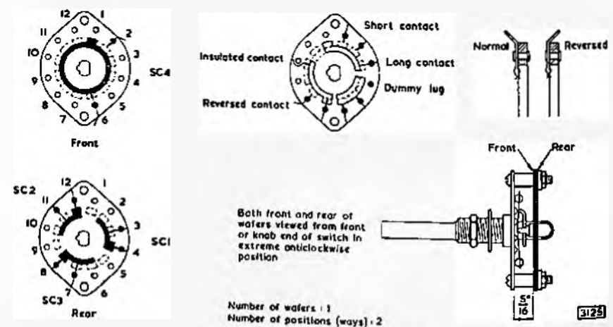
Fig. 17—EQUALISER SWITCH DETAILS
