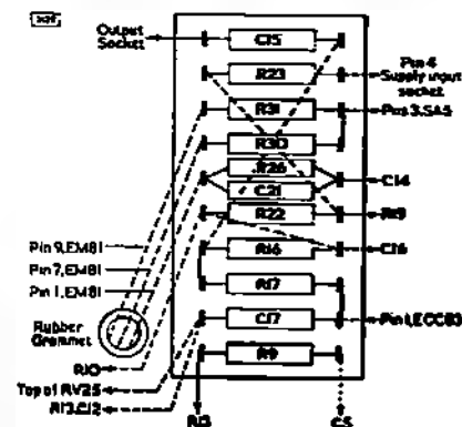
Fig. 13—TAGBOARD No. 3
