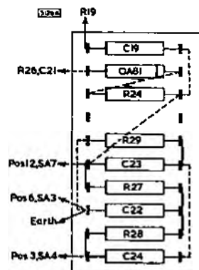
Fig. 22—TAGBOARD No. 4
