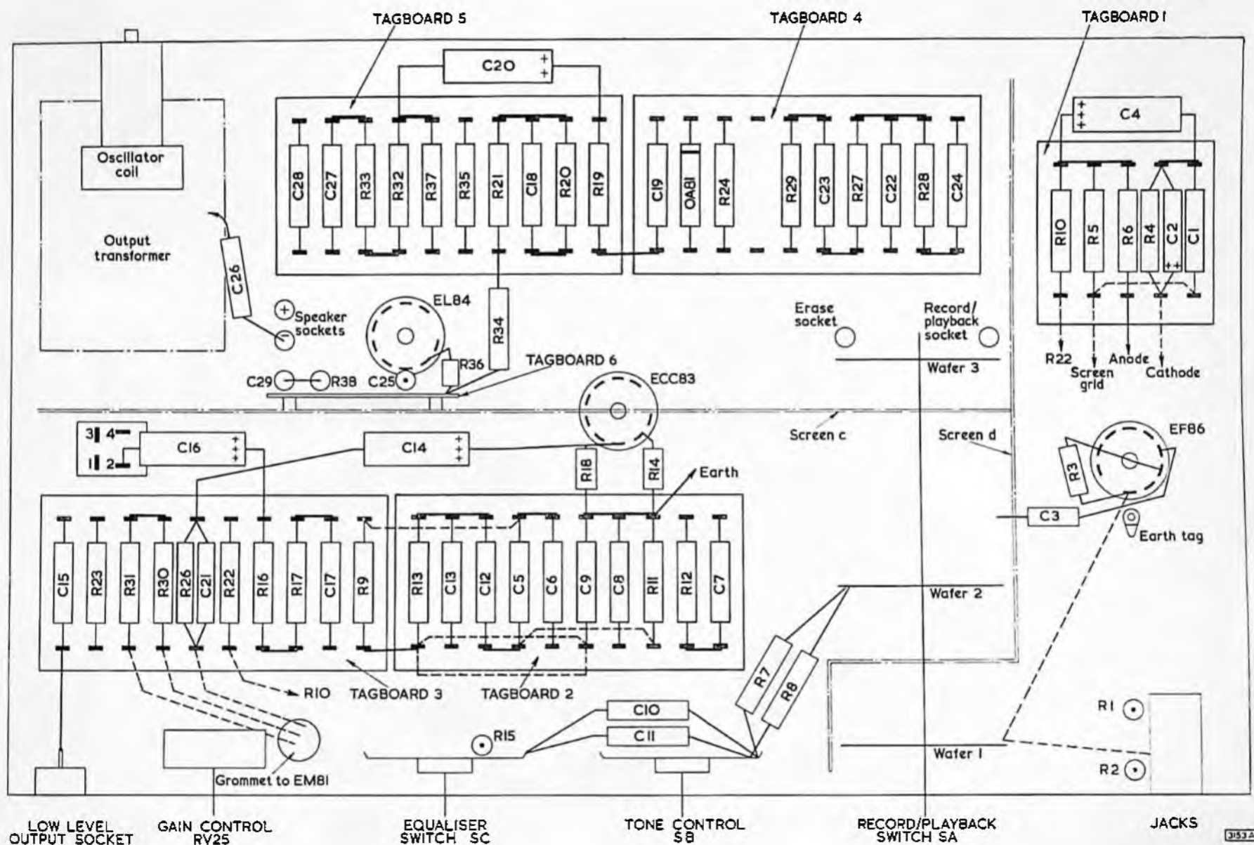
Fig. 4—COMPONENT LAYOUT DIAGRAM (Components which would obscure parts of the layout have not been shown)
