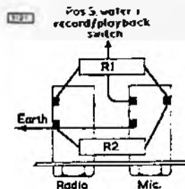
Fig. 12—INPUT-ATTENUATING RESISTORS
