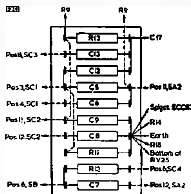
Fig. 15—TAGBOARD No. 2
