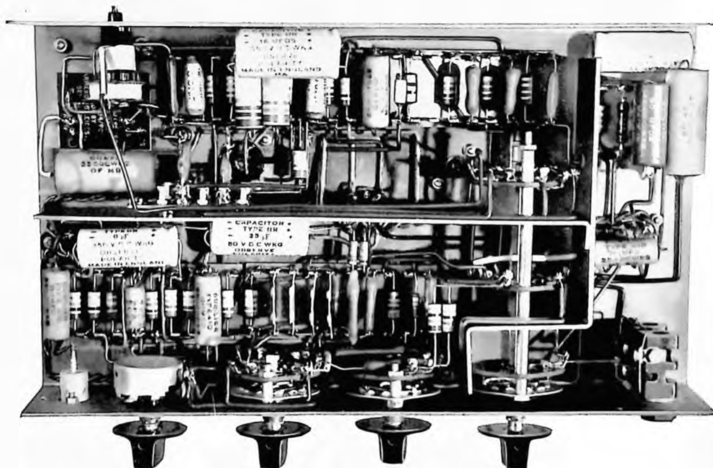
PHOTOGRAPH OF UNDERSIDE OF PROTOTYPE AMPLIFIER
