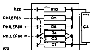
Fig. 10—TAGBOARD No. 1
