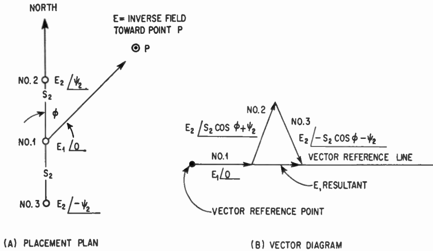
FIG. C-1. Three-tower-in-line array.
