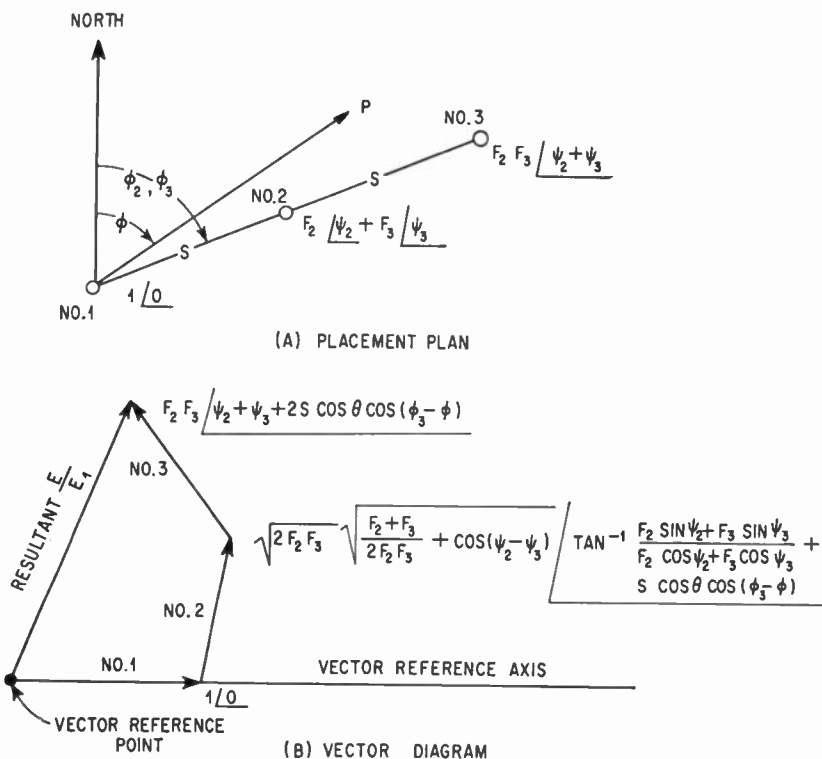
FIG. C-3. Special three-tower-in-line array.
