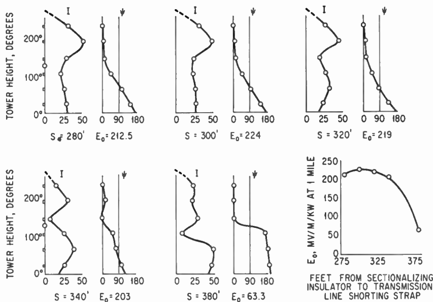
FIG. A-6. Performance of sectionalized tower with top section excited through reactance element from bottom section.
