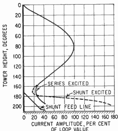
FIG. 3-3. Experimental current distribution on shunt- and series-fed tower. (Morrison and Smith, Proc. IRE , June, 1937.)
