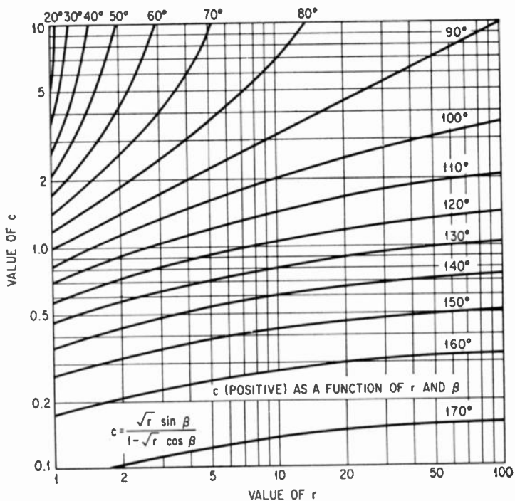
FIG. B-23. Design chart for c (positive) as function of r and \beta .
