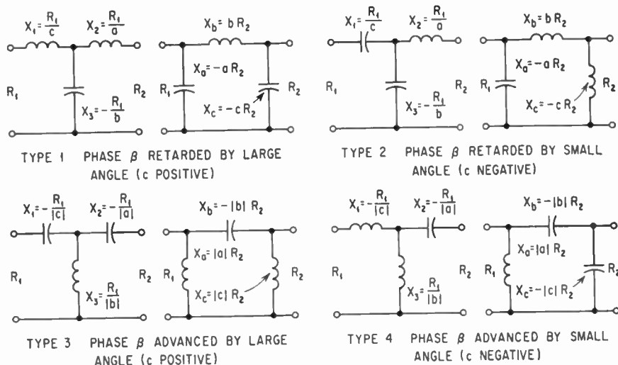
FIG. B-19. Specific three-element reactance networks.
