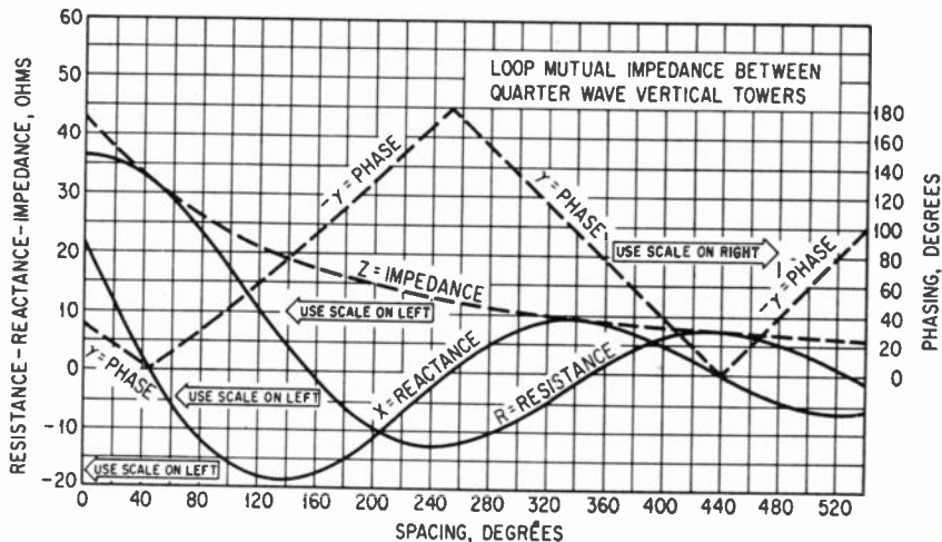
FIG. B-14. Loop mutual impedance between quarter-wave vertical towers.
