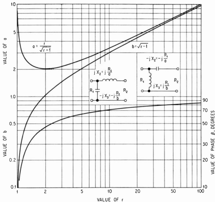
FIG. B-17. L-section design chart.
