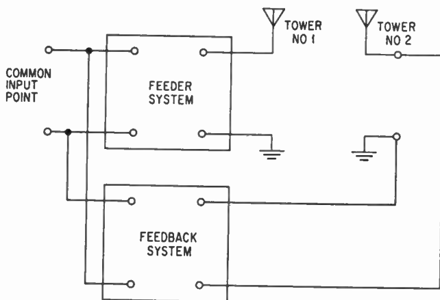
(B) NEGATIVE TOWER CONNECTED THROUGH FEEDBACK SYSTEM TO COMMON POINT
