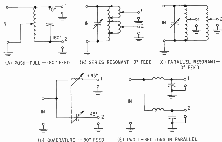
FIG. B-28. Typical power-dividing networks.
