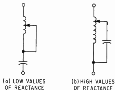
FIG. B-29. Methods of varying reactance.
