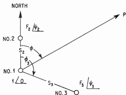
(A) PLACEMENT PLAN
