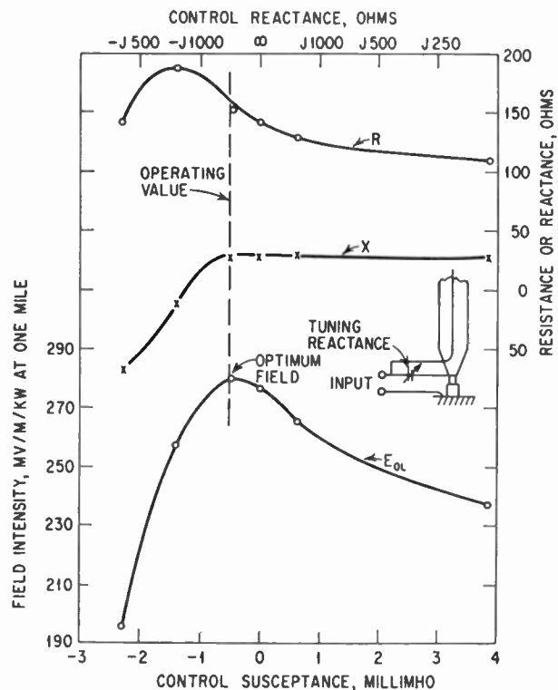
(A) INPUT IMPEDANCE AND FIELD STRENGTH OF TOP LOADED SECTIONALIZED 258° TOWER AS FUNCTION OF TUNING REACTANCE
