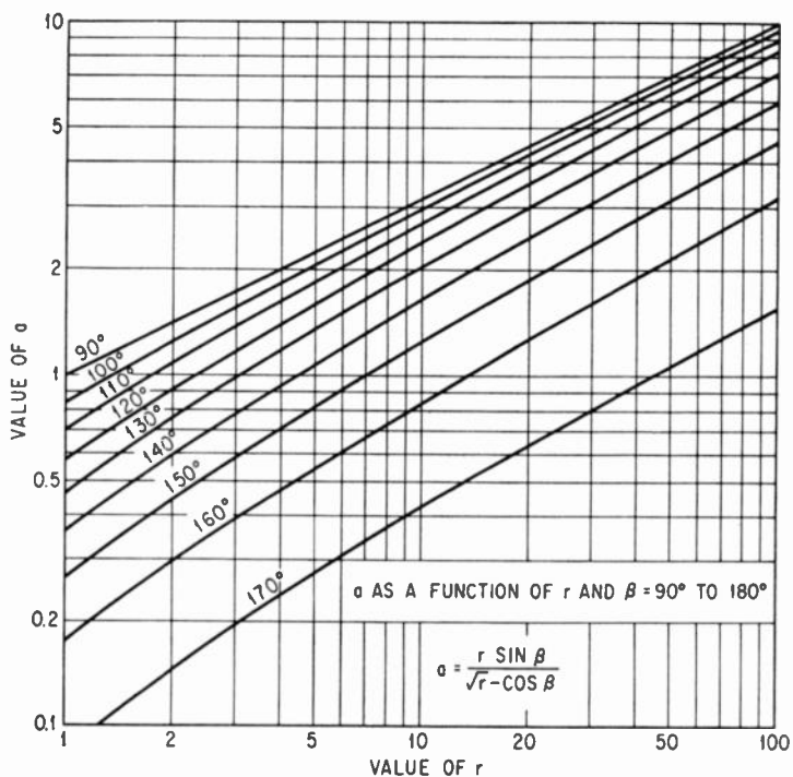
FIG. B-21. Design chart for a as function of r and \beta = 90 to 180^\circ .
