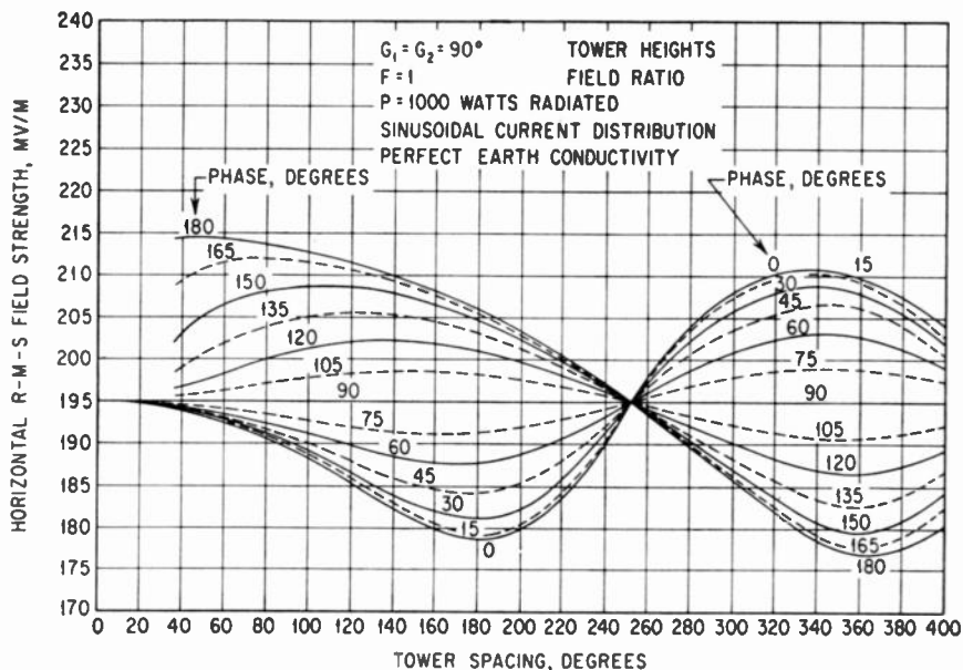
FIG. B-15. Horizontal rms field strength of two-tower directional antenna.
