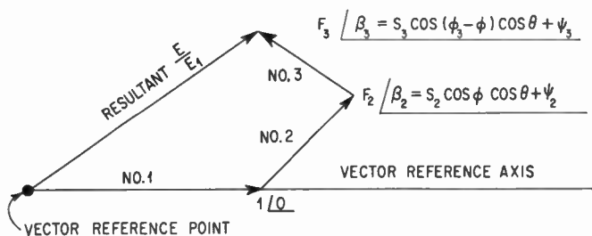
(B) VECTOR DIAGRAM
