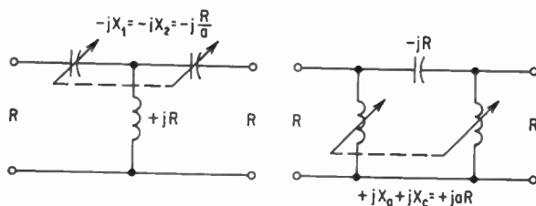
FIG. B-26. Phase-shifting networks.
