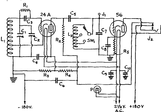
FIG. 2—CIRCUIT OF THE FREQUENCY-METER-MONITOR
