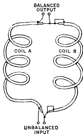
Fig. 1—Two tightly-coupled coils of coax connected to provide a unbalanced to balanced transformation.
