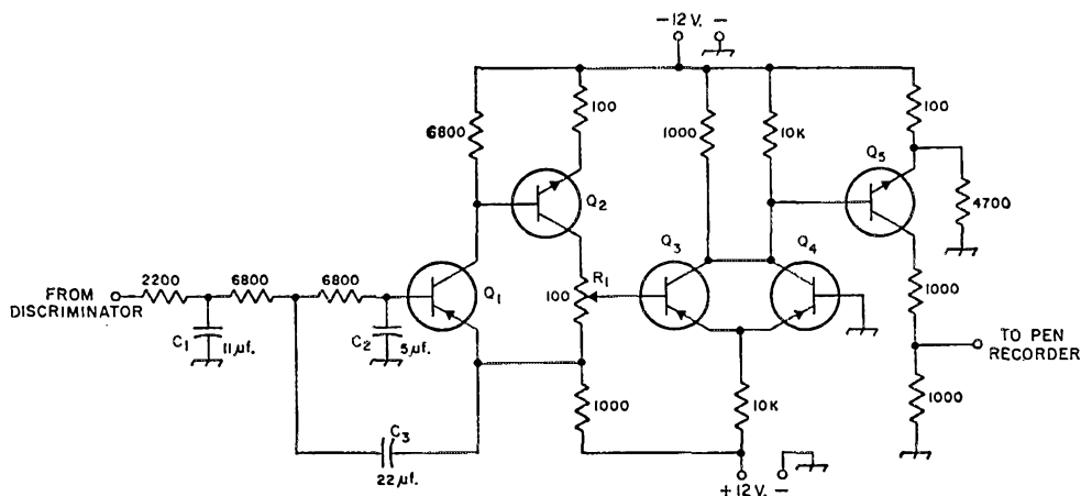
Fig. 2—Circuit of the low-pass filter and slicer. Resistances are in ohms; fixed resistors are ½ watt composition.
