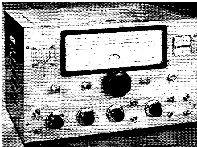
The HBR-13C, built by Alexander Stewart, WA4ZNI, is the basic HBR-11 or HBR-12 plus the additions and modifications described in the text. Major electrical changes are the addition of an amplifier stage at the first intermediate frequency (1610 kc.) and one more transformer in the 100-kc. second-i.f. amplifier. The mechanical arrangement permits centering the large Eddystone dial.
