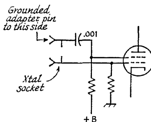
Fig. 2—In transmitters using modified Pierce oscillators, the adapter should be plugged into the transmitter crystal socket in such a direction that the grounded side of the adapter connects to the screen blocking capacitor, as indicated here.
