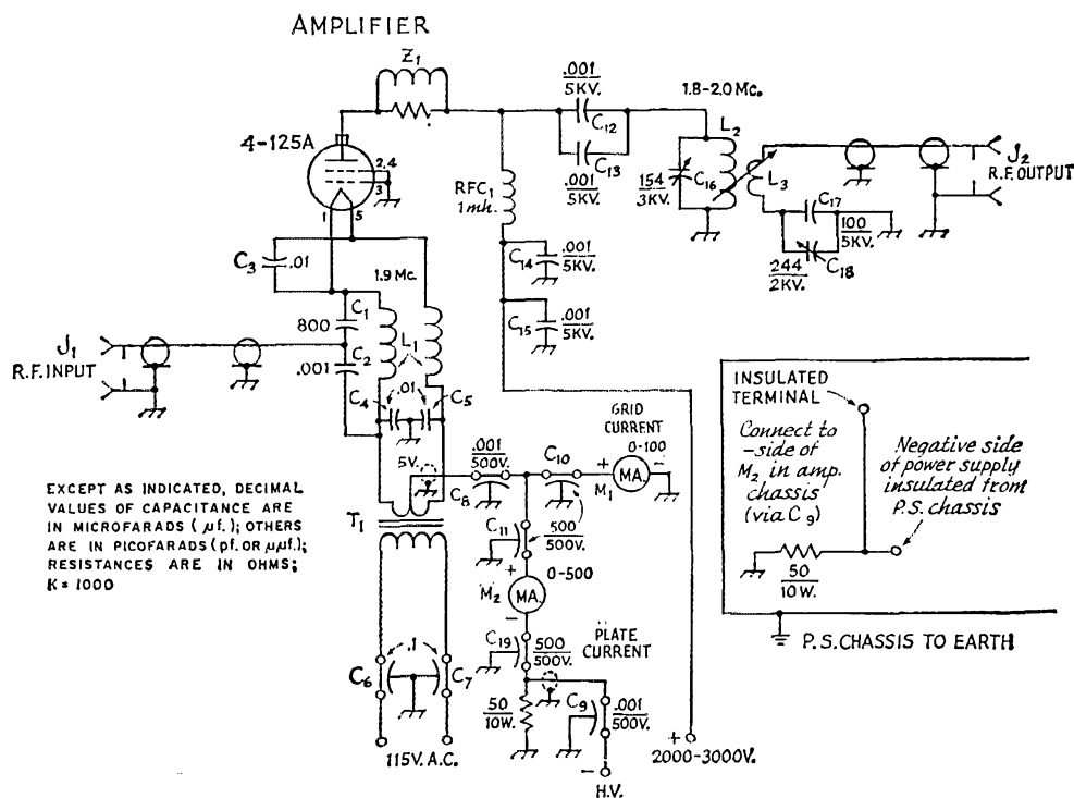
Fig. 1—Circuit of the 160-meter grounded-grid amplifier.
