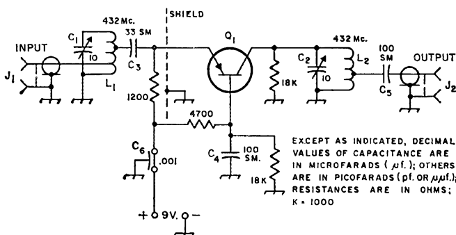
Fig. 2—Schematic diagram of the 432-Mc. preamplifier. 5 M indicates silver mica. Resistors are \frac{1}{4} watt, carbon.
