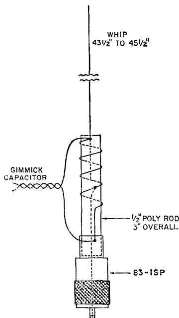
Fig. 1—The \frac{5}{8} -wave 2-meter whip mounts in a poly rod, inserted in the top of a coaxial plug. Impedance matching coil is wound on the rod, and the line to the transmitter is tapped up one turn from the bottom end. The coil is tuned with a "gimmick" capacitor.
