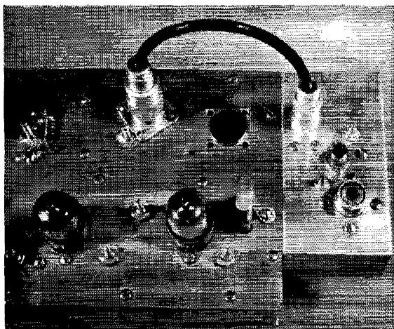
Fig. 1—Top view of the 432-Mc. preamplifier showing it attached to the converter as a subassembly.
