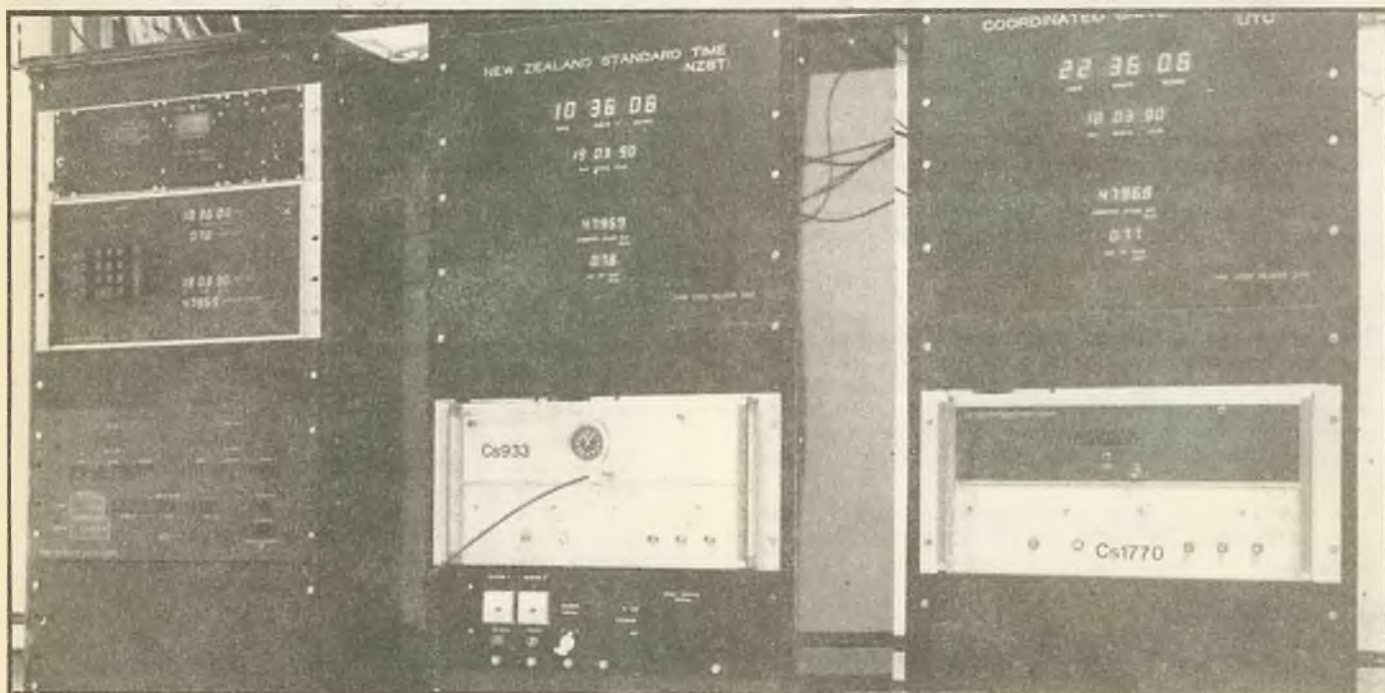
Two of the three atomic clocks constituting the New Zealand time and frequency standard (lower centre and lower right). The time pip generator is upper left.
