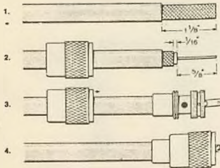
UHF type (soldered screen)
