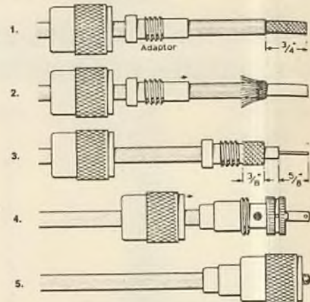
UHF type (clamped screen)
