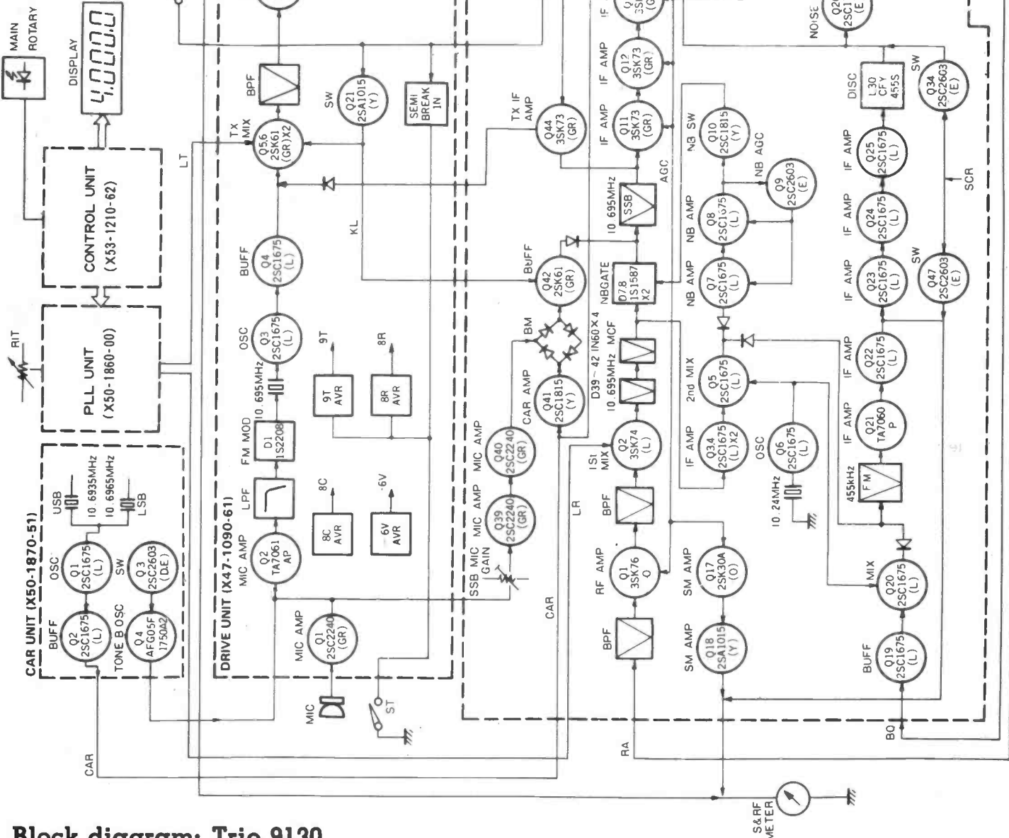
Block diagram: Trio 9130
