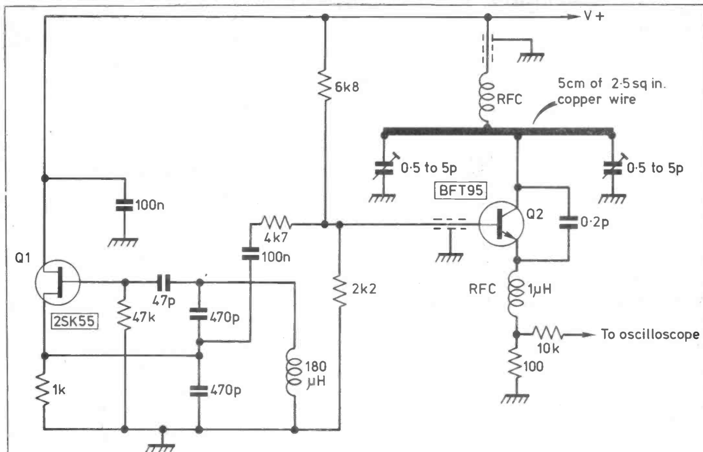
Fig. 5. 23cm Super regenerative test circuit.
