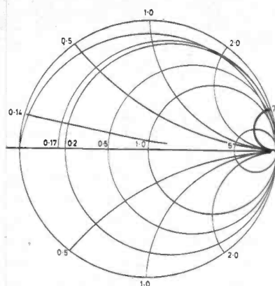
Fig. 8f. Calculating the value of the series capacitor, C1.
