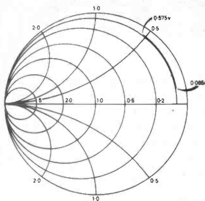
Fig. 8e. Admittance overlay.
