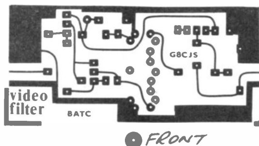
Foil Patterns for the Video Low Pass Filter and Vision Switching PCBs.
