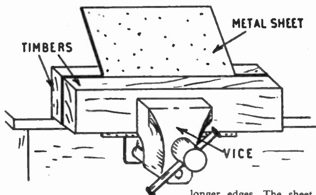
Fig. 1—Bending up a chassis
