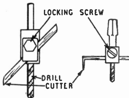
Fig. 2—Valveholder hole cutters
