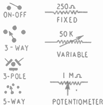
Fig. 1 Switches and resistances
