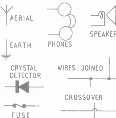
Fig. 4 Other symbols
