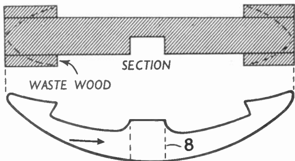
PIECE 9. CUT ONE \frac{3}{8} in.
