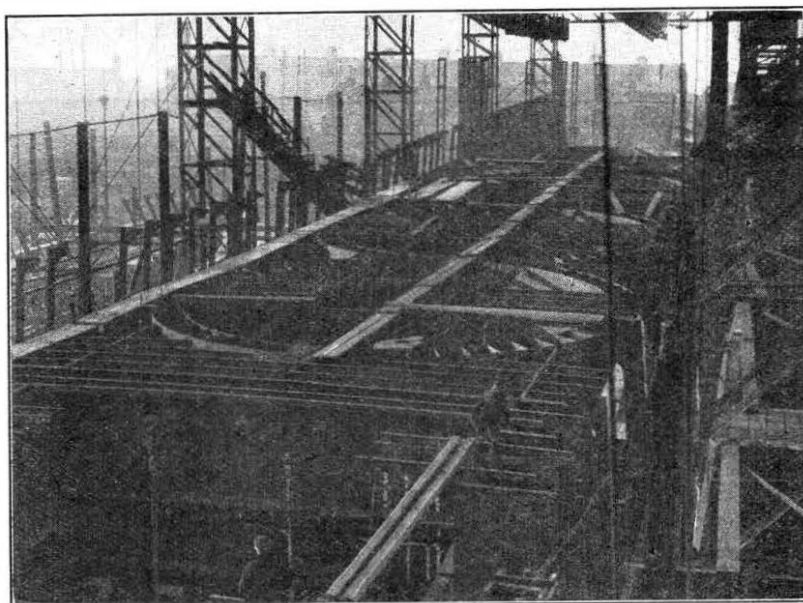
Fig. 2.—FRAMING, SHOWING CABLE TANKS AND COFFERDAM.
