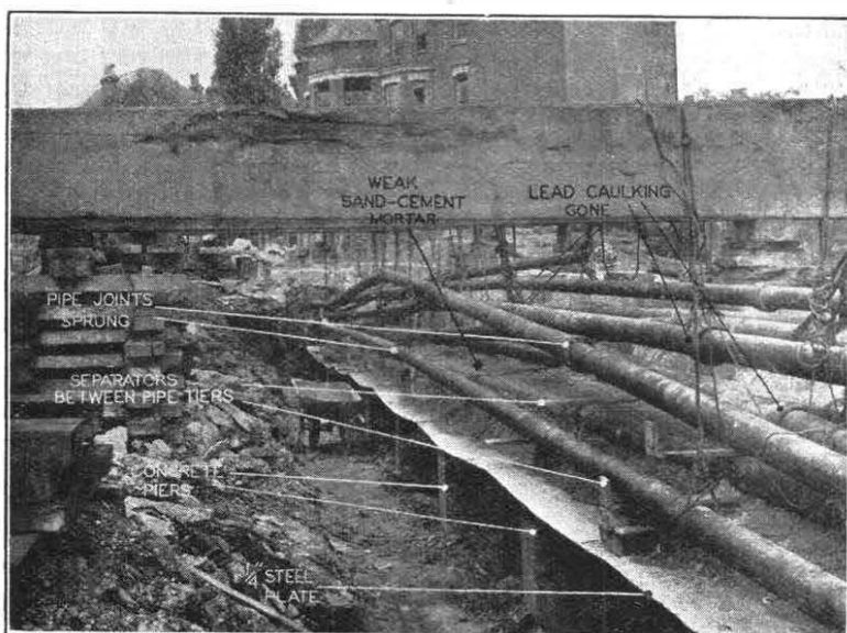
FIG. 5.—RECONDITIONING OF PIPES AT ADVANCED STAGE.
