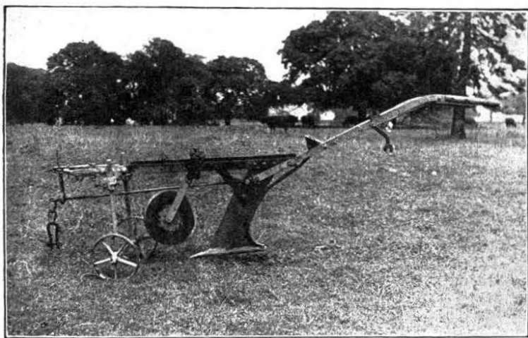
FIG. 1.—LIGHTWEIGHT MOLEDRAINER.
