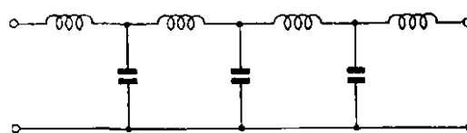
FIG. 3.—LOW-PASS FILTER CONSISTING OF 3-PROTOTYPE SECTIONS.
