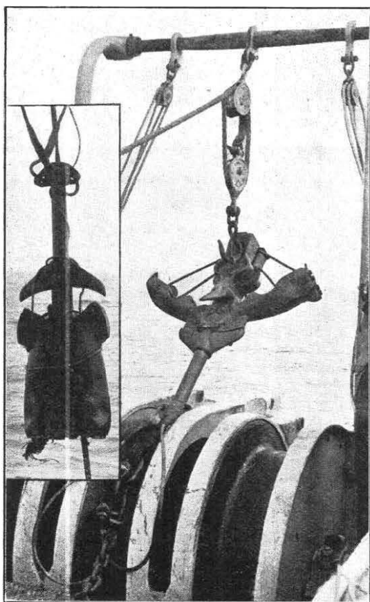
Fig. 11.—LUCAS GRAPPLE IN OPEN POSITION (INSET CLOSED).
