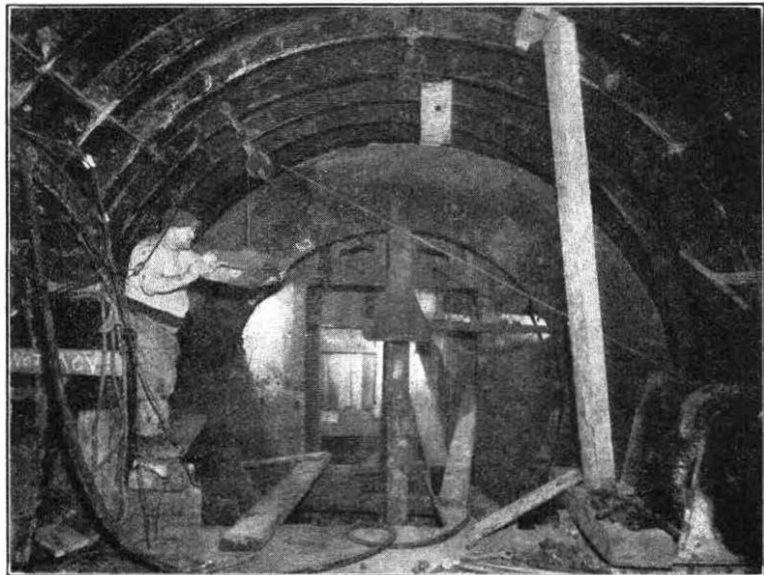
FIG. 6.—"GREATHEAD" SHIELD BEING ERECTED.
