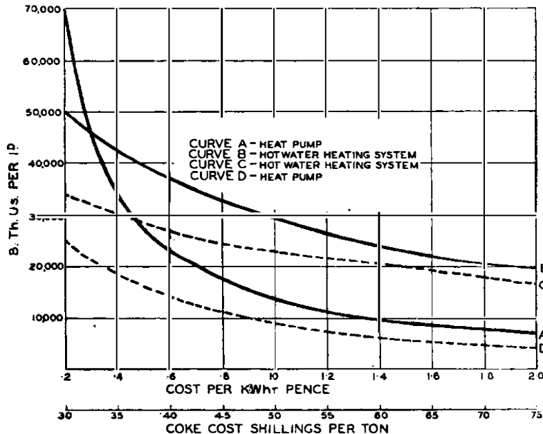
FIG. 7.—CURVES SHOWING RELATIVE COST OF HEAT UNITS BASED ON BOILER EFFICIENCY 70% AND HEAT PUMP COEFFICIENT OF PERFORMANCE OF 4.
