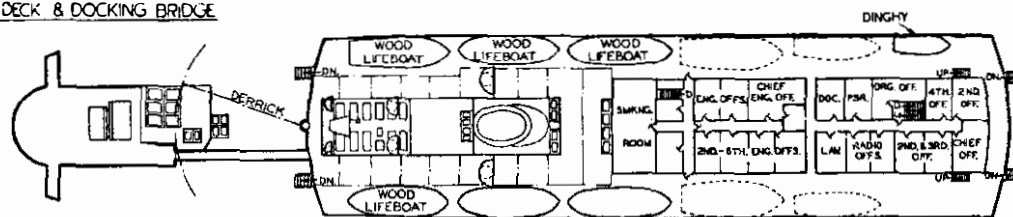
BOAT DECK &amp; DOCKING BRIDGE
