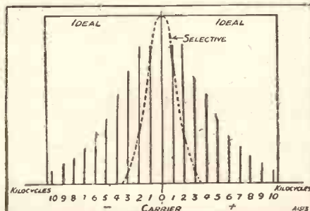
The ideal response would be flat-topped, as shown, and the dotted line, representing a selective receiver, shows how far from ideal such a set can be.
