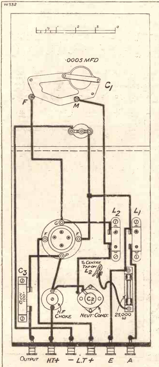
You will find no difficulty in wiring this amazing little unit.
