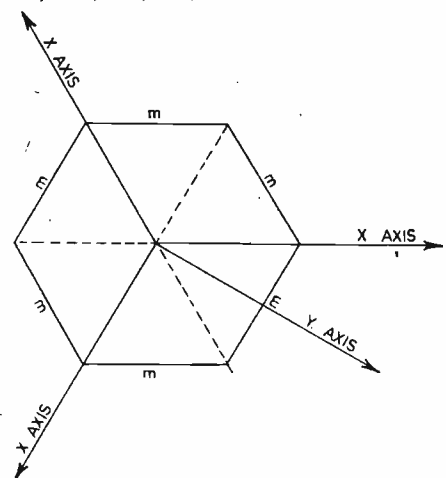
Fig. 2. Section of Quartz crystal normal to Z axis showing location of X and Y axis and m faces
