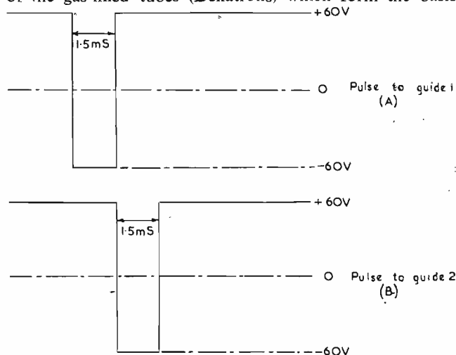
Fig. 3. Pulse to operate counting tube.
