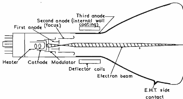
Fig. 2. Electrostatic focus, magnetic deflexion
