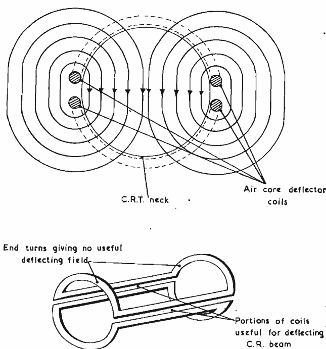
Fig. 11. Air-core deflector coils
