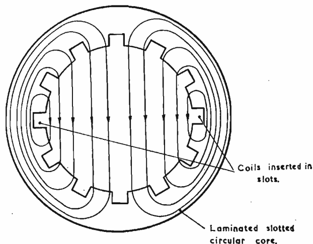
Fig. 10. Slotted iron-core deflecting coil
