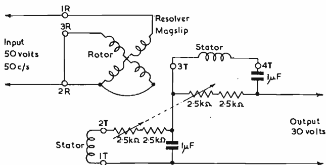
Fig. 1. Connexions of mag-slip
