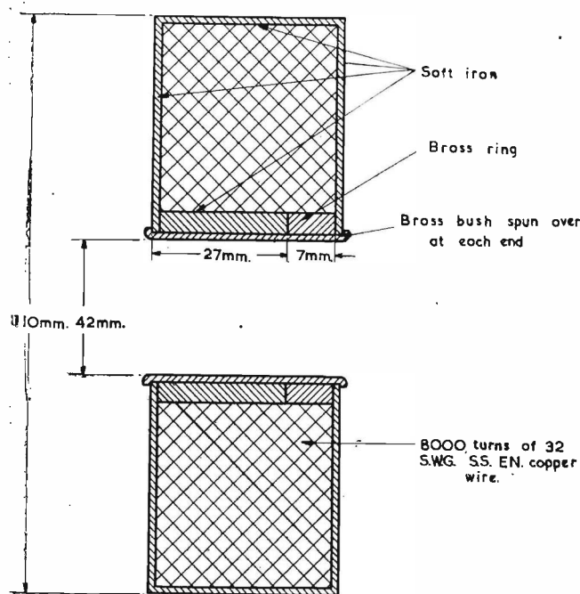
Fig. 6. Typical electromagnet for use with C.R.T.
