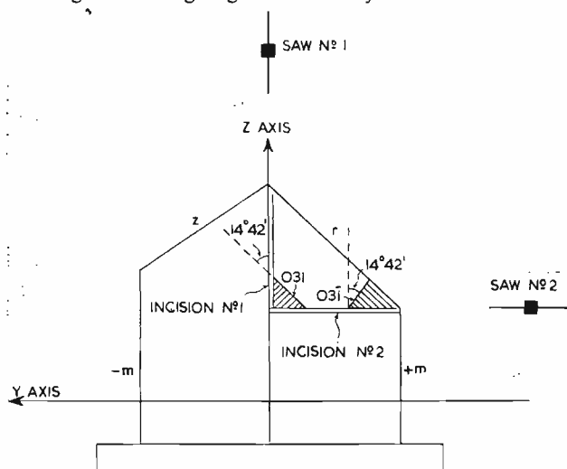
Fig. 8. Cutting the test piece
