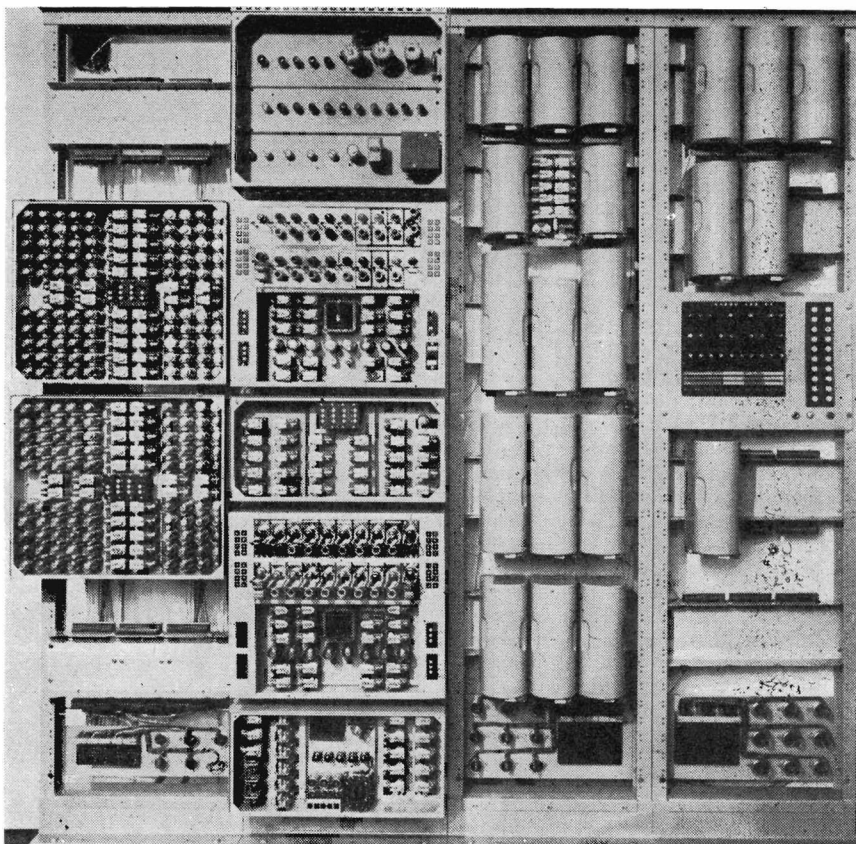
Computer fitted with 20 stores, but excluding tape readers, printers and power supply. The left hand rack carries two units each of ten stores. The left centre rack carries the electronic pulse generator (top), the arithmetic units with relay shift unit (centre) and the translator unit (bottom). The two right hand racks contain the relay sequence control circuits.
