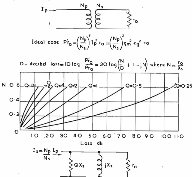
Fig. 1. Shunt loss of transformer
