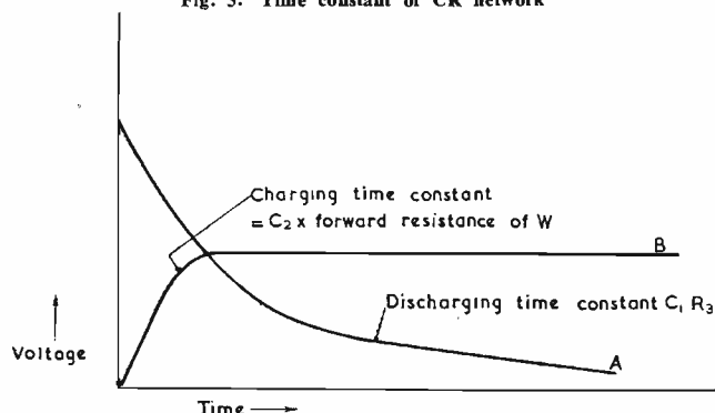
Fig. 3. Time constant of CR network
