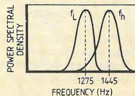
Fig. 2. Power spectral density of the new tones standard for 170Hz shift at 50 baud sending speed is accurately matched by the digital filter realisations achieved by the use of an inexpensive 8 bit microprocessor using 16 bit arithmetic.
