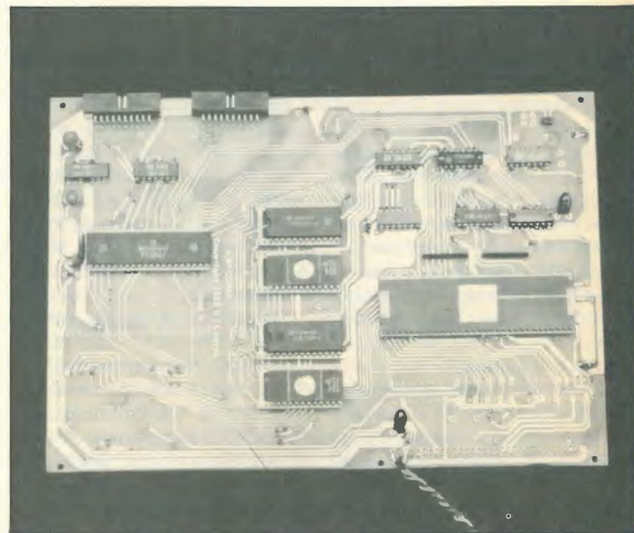
The kit p.c.b. is not a plated-through type; this saves money but requires use of turned-pin i.c. sockets.
