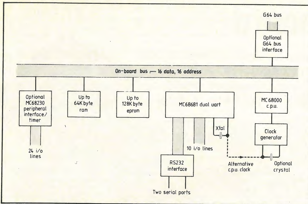
Fig. 2. Kaycomp uses a full 68000 processor and two peripheral i.c.s from the same family. Using these instead of more common 6800 peripherals means higher performance and increases the board's value as an evaluation tool.
