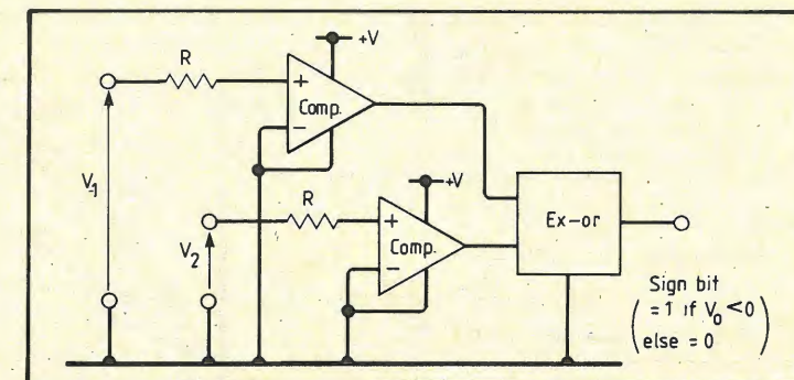
Fig. 6. Sign-information circuit.
