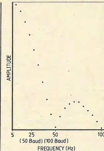
Fig. 6. In addition to the digital realisation of the channel filters, further post-detector filtering tailored to the bit rate is also provided.
