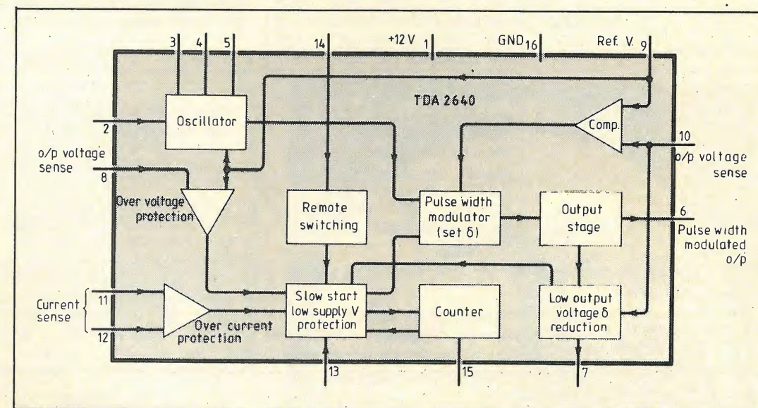
Fig. 4. TDA2640 contains advanced control and monitoring circuitry, as outlined here.
