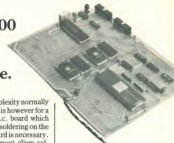
Our front cover shows the 68000 board in its fullest form with G64-bus interface — this is the basic version.
