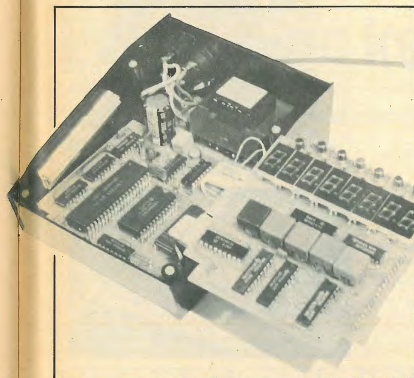
The instrument, based on a Z80 processor with 2K of ram, uses low-cost components throughout. The same hardware could be used to implement a general i/o controller, for example in a security installation or central heating system.
