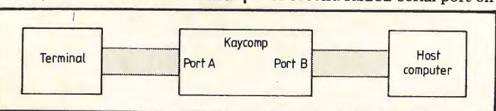
Fig. 3. Kaycomp can be used by simply connecting a dumb terminal but in this configuration, it is effectively connected in the terminal line from the host computer. In this way, software developed using 68000 assemblers and compilers on the host can be fed directly into the board.
