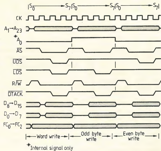
Fig. 7. Action of upper and lower data strobes UDS and LDS used when addressing bytes. These strobes are needed because the 68000 has no address-line zero.
